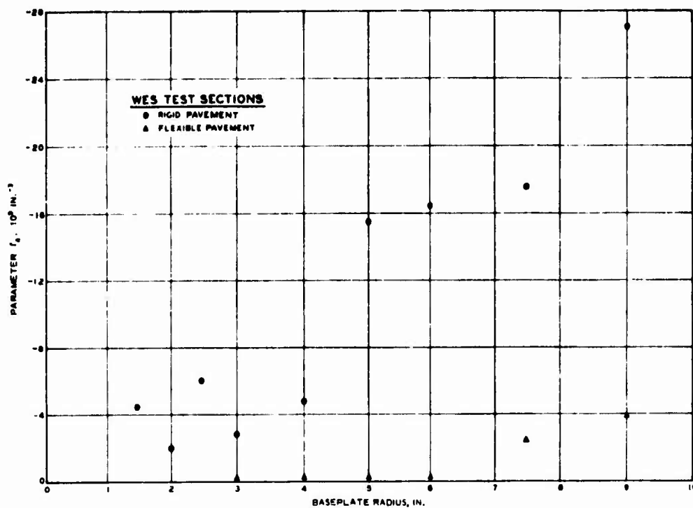
Figure 27. Experimentally derived values of the parameters l_4 versus baseplate radius
