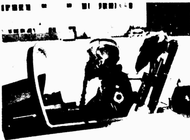
Fig. 4. A YF-16/17 test pilot is shown demonstrating the seated posture used by him on maneuvers in the YF-17 ( 18^\circ seatback angle).
