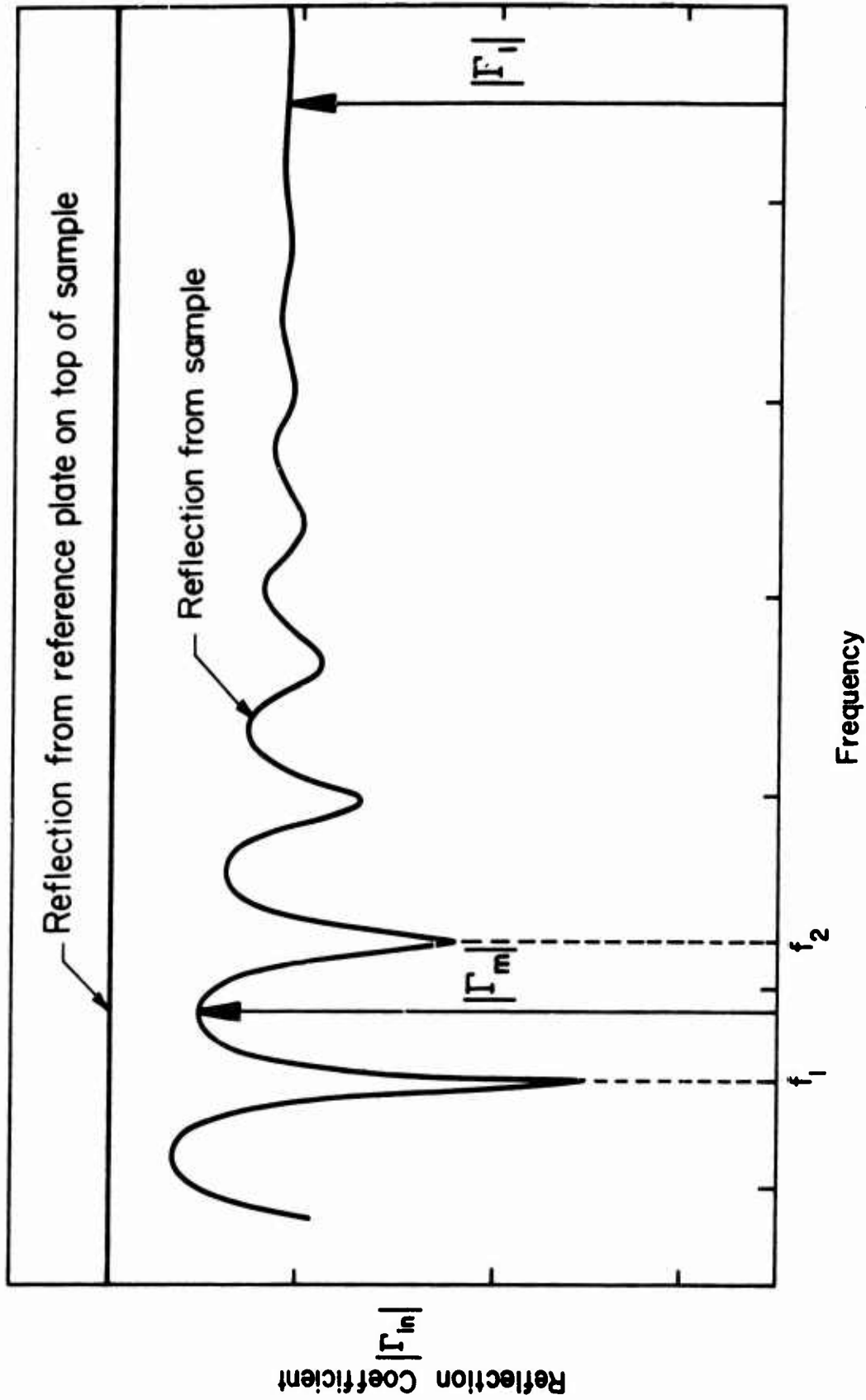
Figure 6. Reflection Coefficient Relationship
