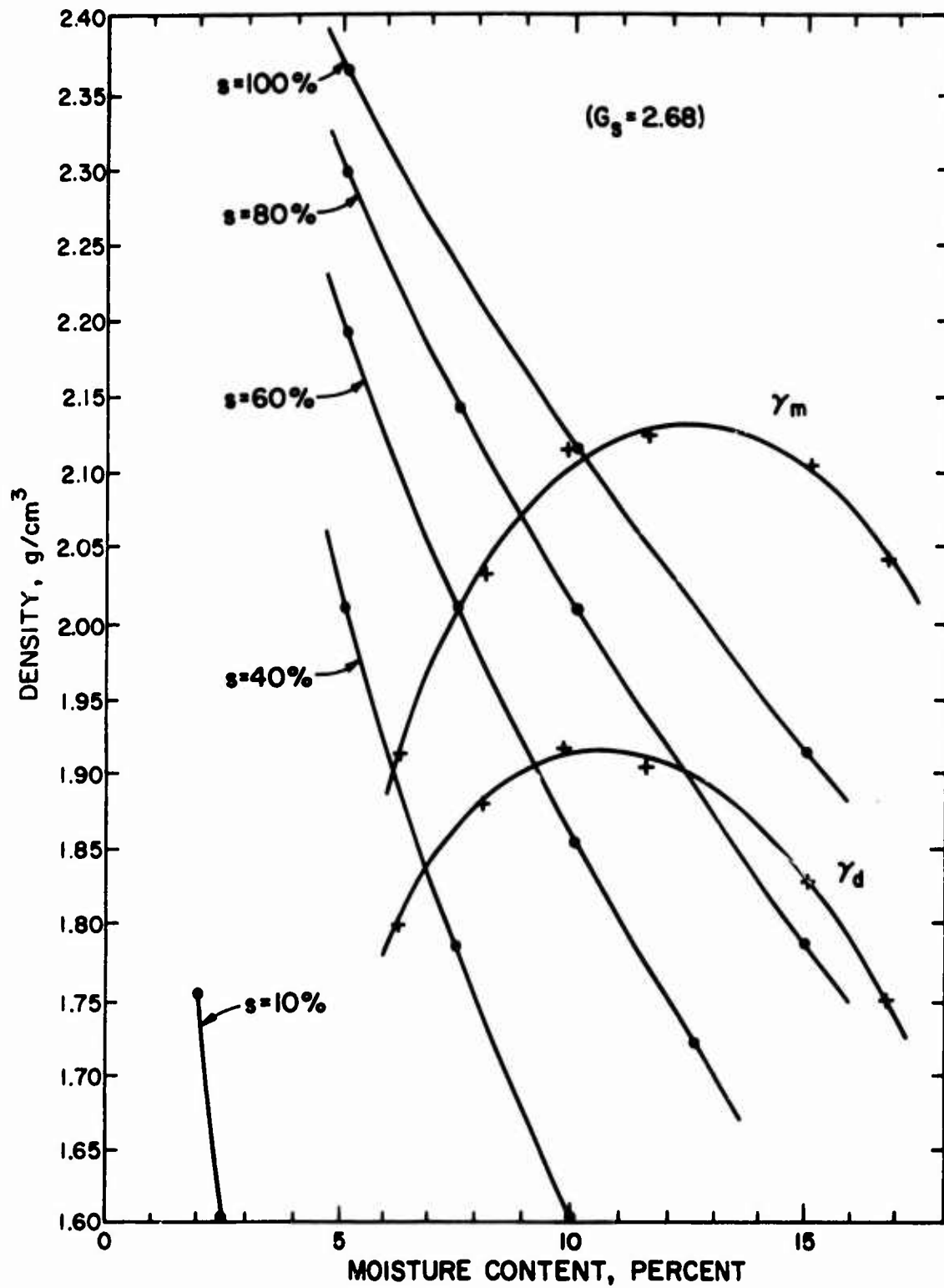
Figure 4. Modified Proctor Compaction of Clay
