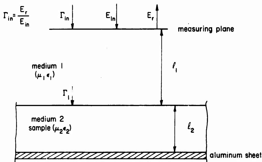
Figure 5. Plane Waves Normally Incident on a Plane Dielectric Boundary
