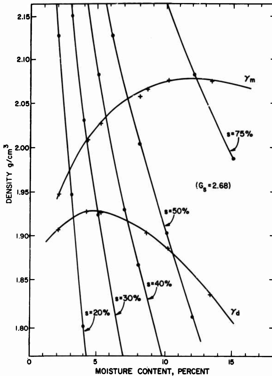
Figure 2. Modified Proctor Compaction of Gravel
