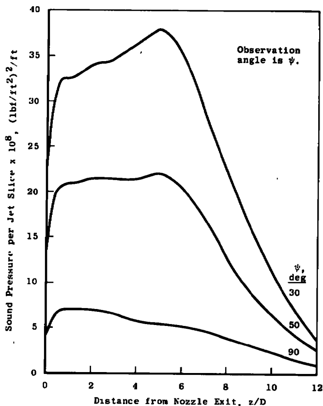
Figure 8. Sound pressure level per jet slice, U_j = 500 ft/sec.
