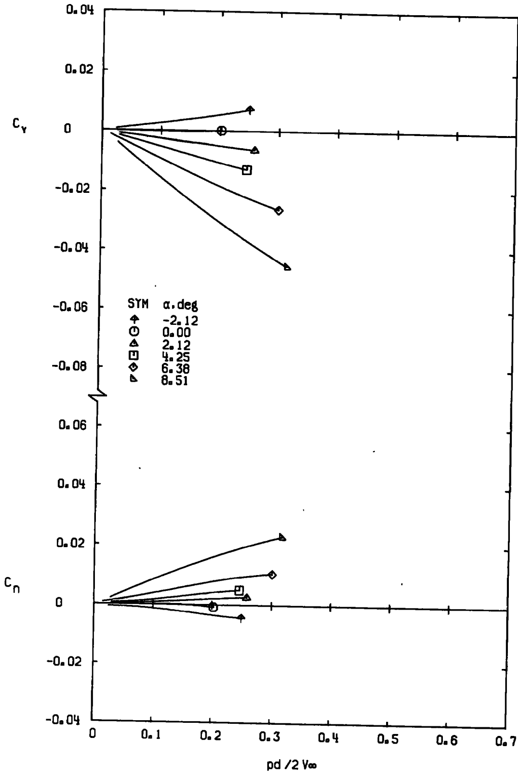
f. M_\infty = 1.10 Figure 12. Continued.
