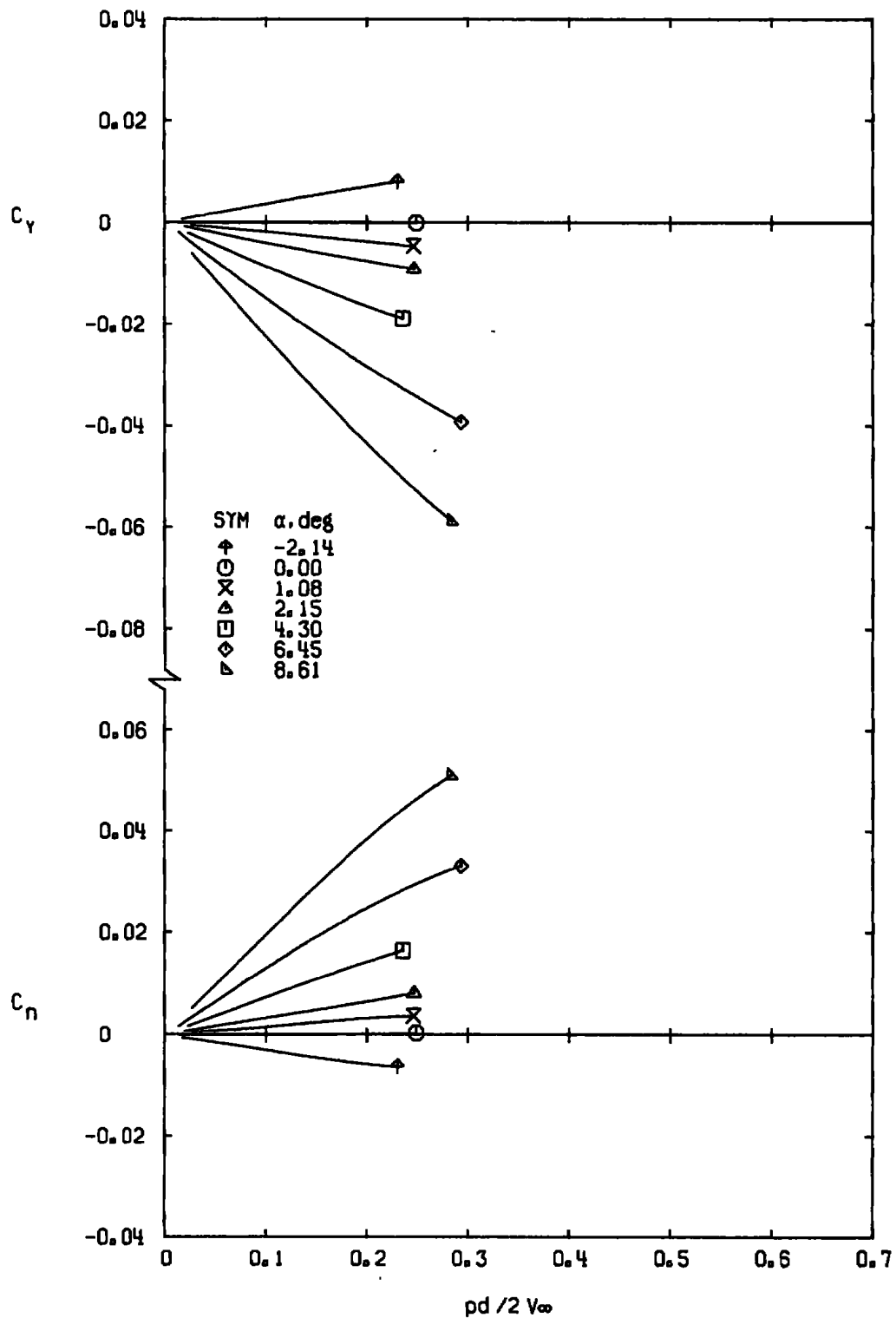
g. M_\infty = 1.30 Figure 17. Concluded.
