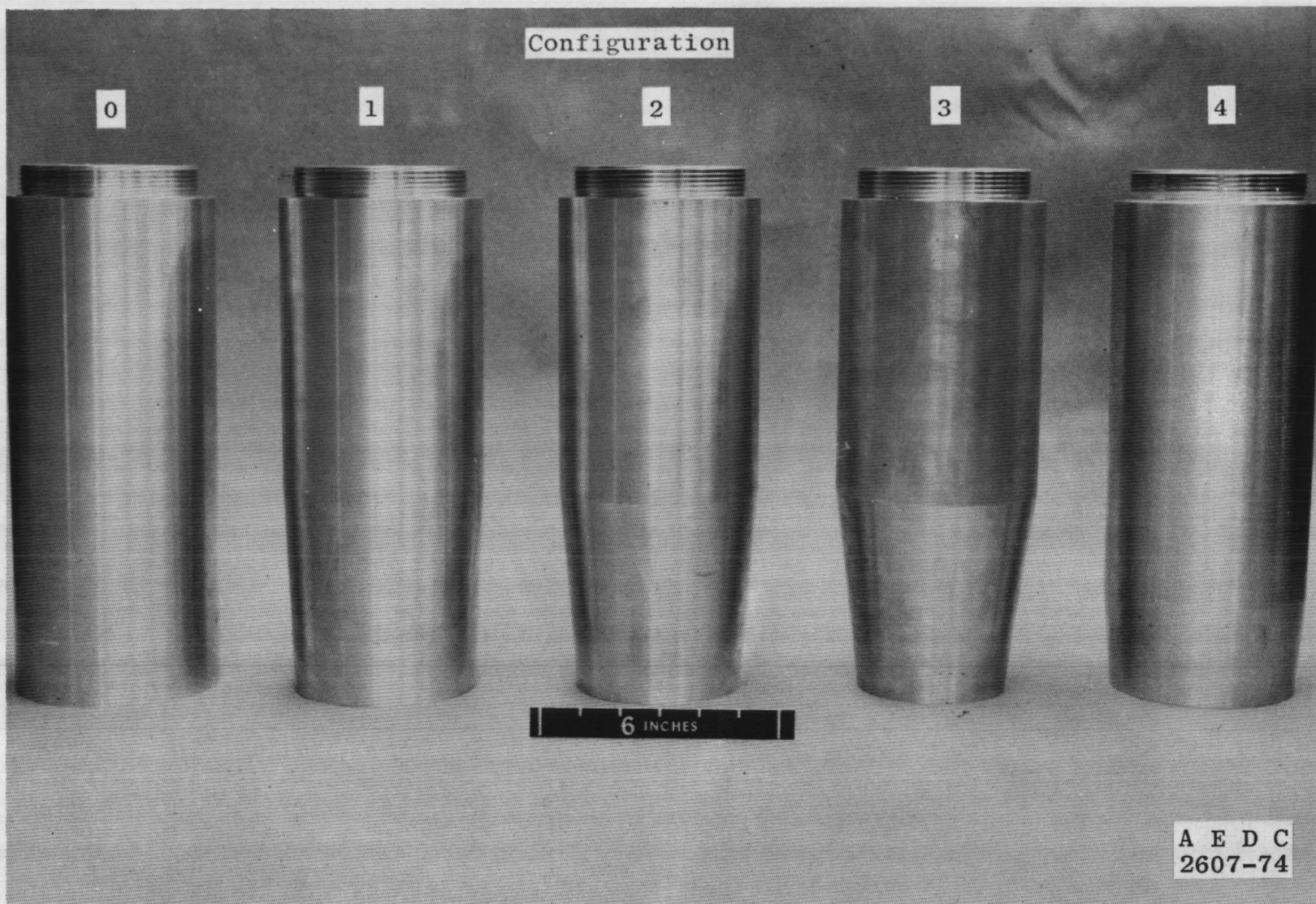
b. Boattail configurations Figure 1. Continued.
