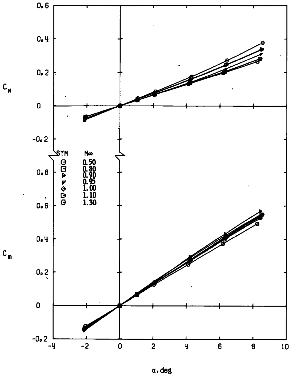
e. Configuration 4 Figure 5. Continued.
