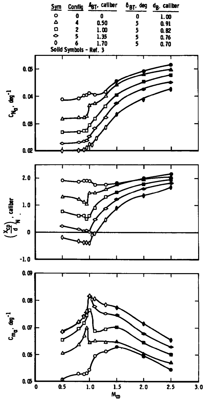
b. Effect of boattail length with a constant boattail angle Figure 6. Continued.
