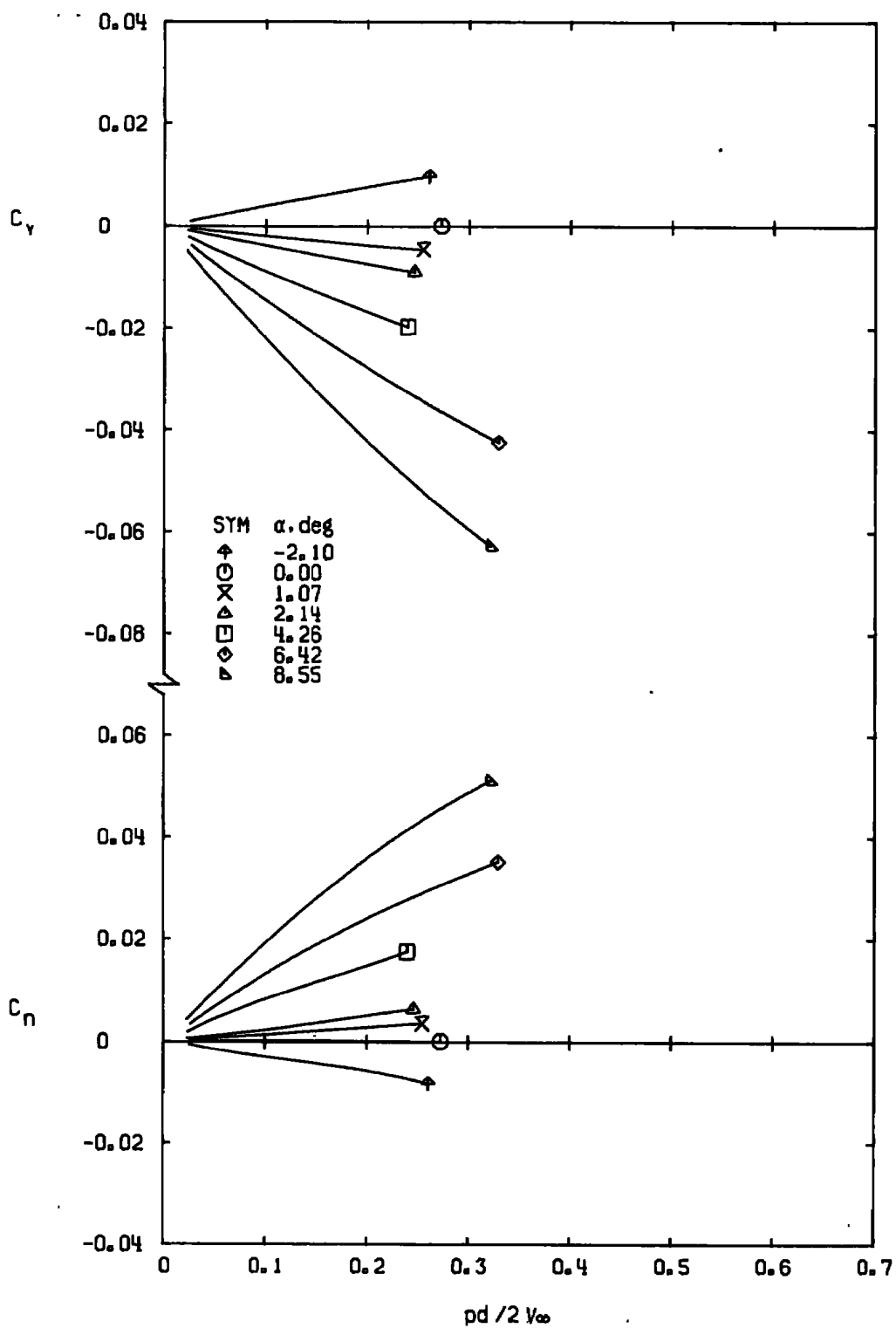
f. M_\infty = 1.10 Figure 11. Continued.
