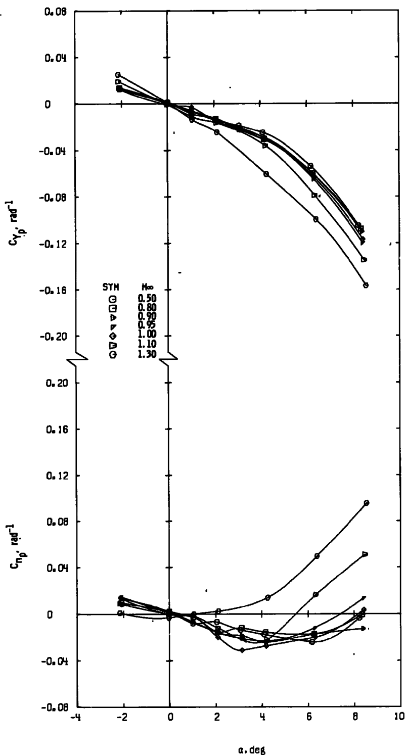
Figure 18. Variation of C_{Yp'} and C_{Np'} with angle of attack, Re_\rho = 9.6 \times 10^6 .
