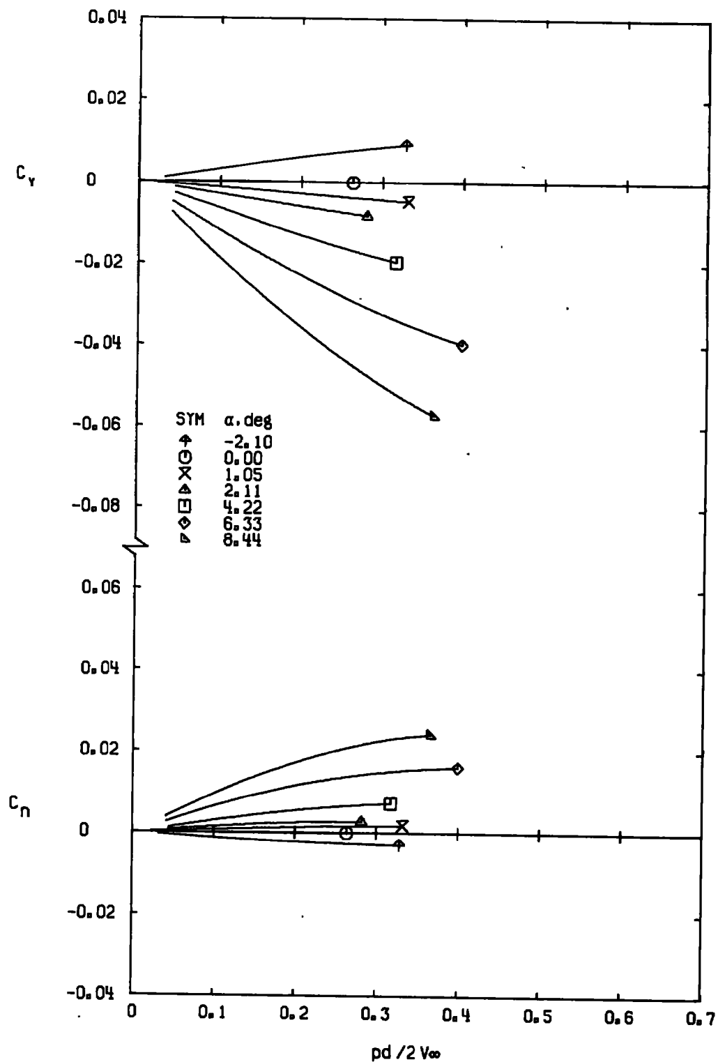
c. M_\infty = 0.90 Figure 13. Continued.
