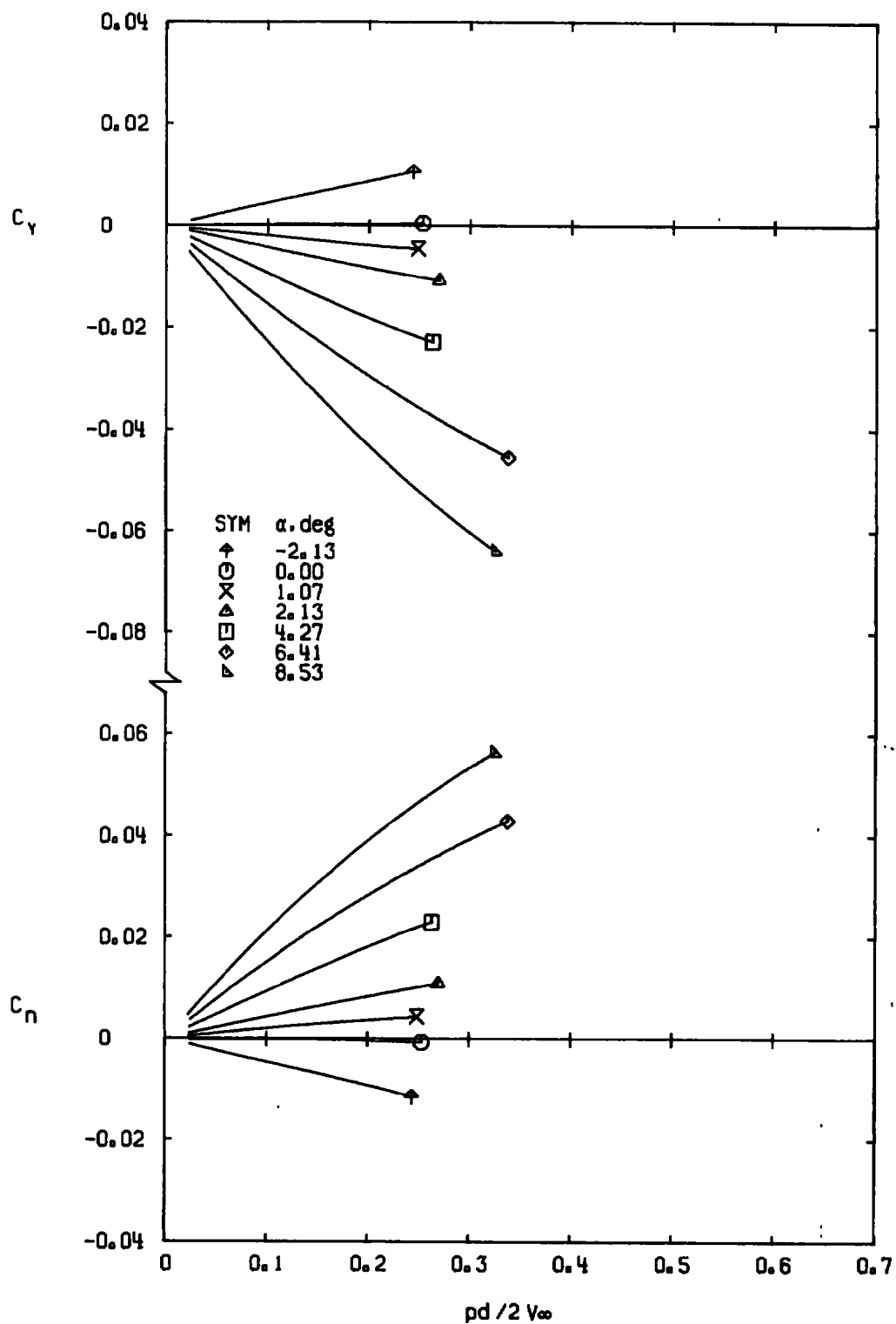
f. M_\infty = 1.10 Figure 16. Continued.
