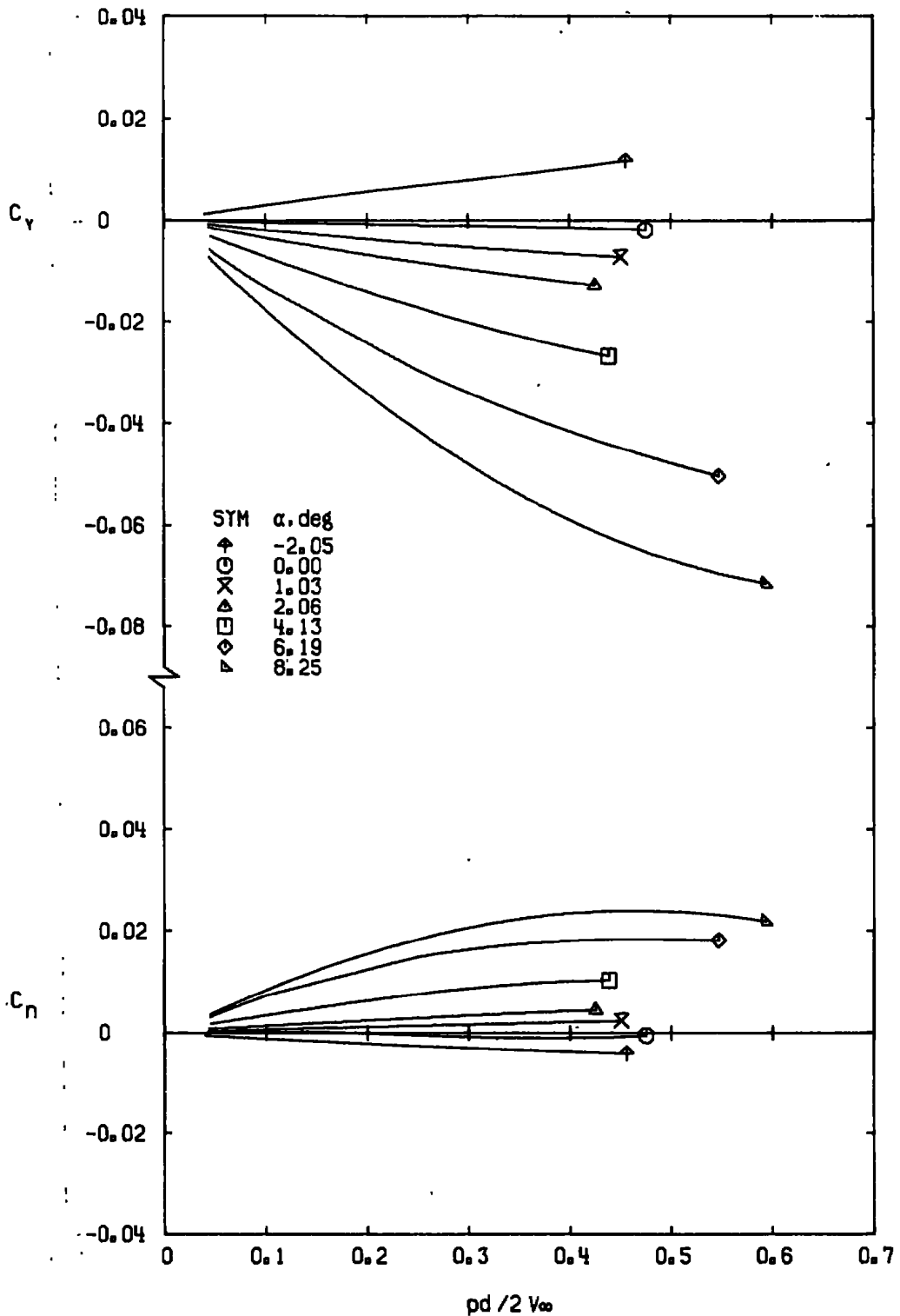
Figure 14. Variation of C_y and C_n with pd/2V_{\infty} for Configuration 6.
