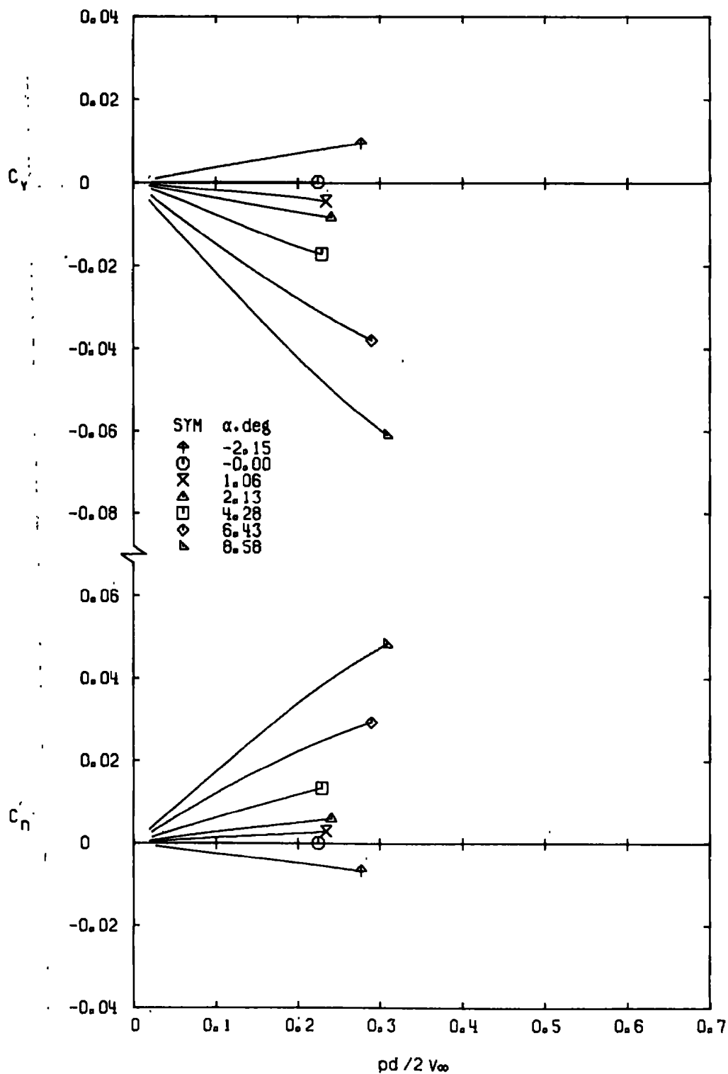
g. M_\infty = 1.30 Figure 14. Concluded.
