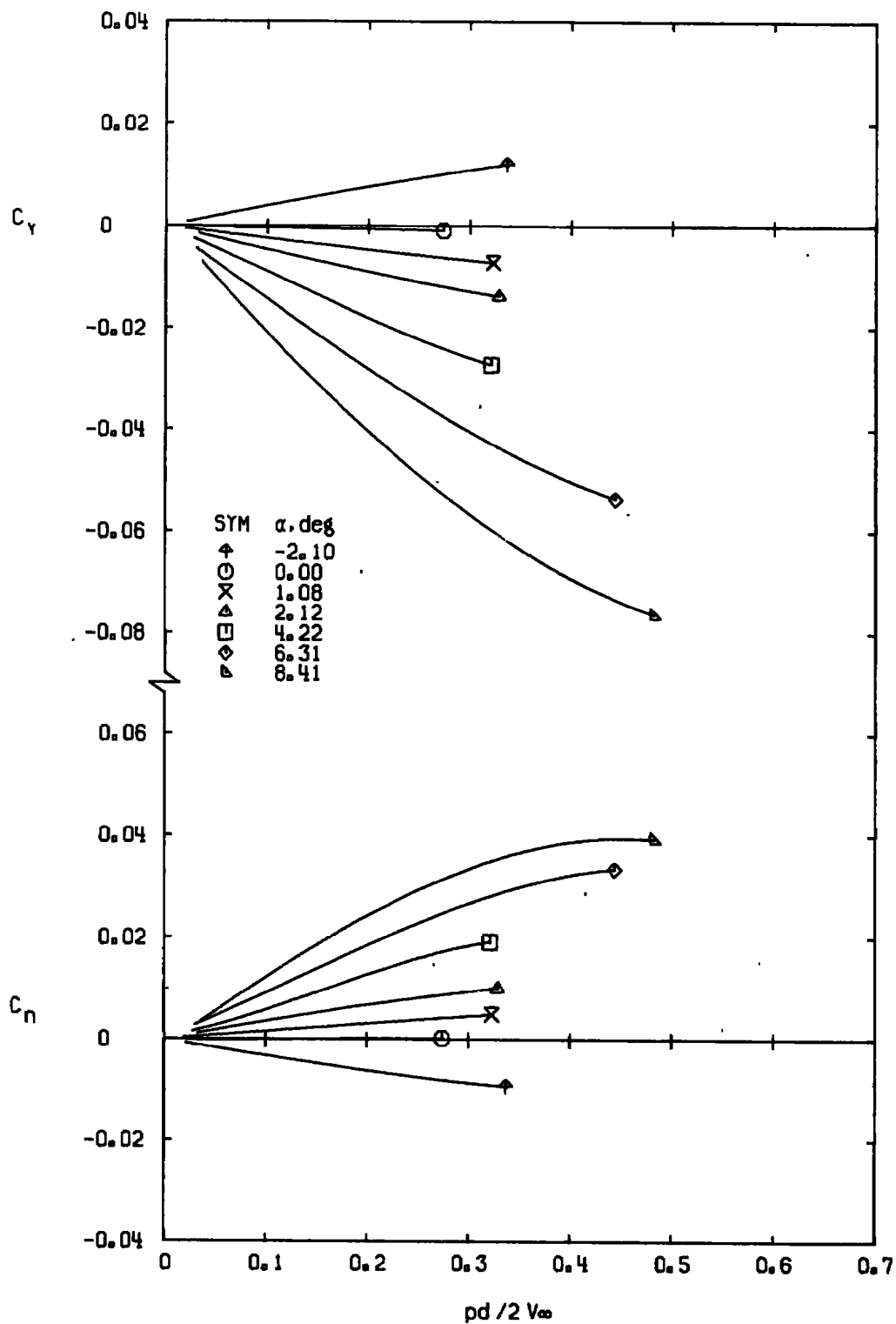
b. M_\infty = 0.80 Figure 16. Continued.
