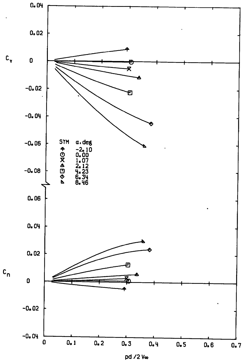
c. M_\infty = 0.90 Figure 11. Continued.
