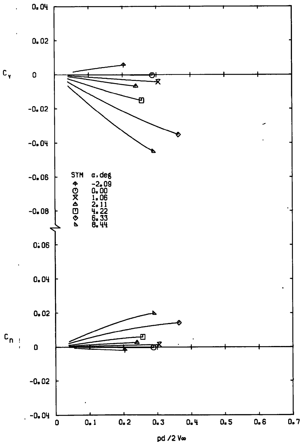
c. M_\infty = 0.90 Figure 10. Continued.
