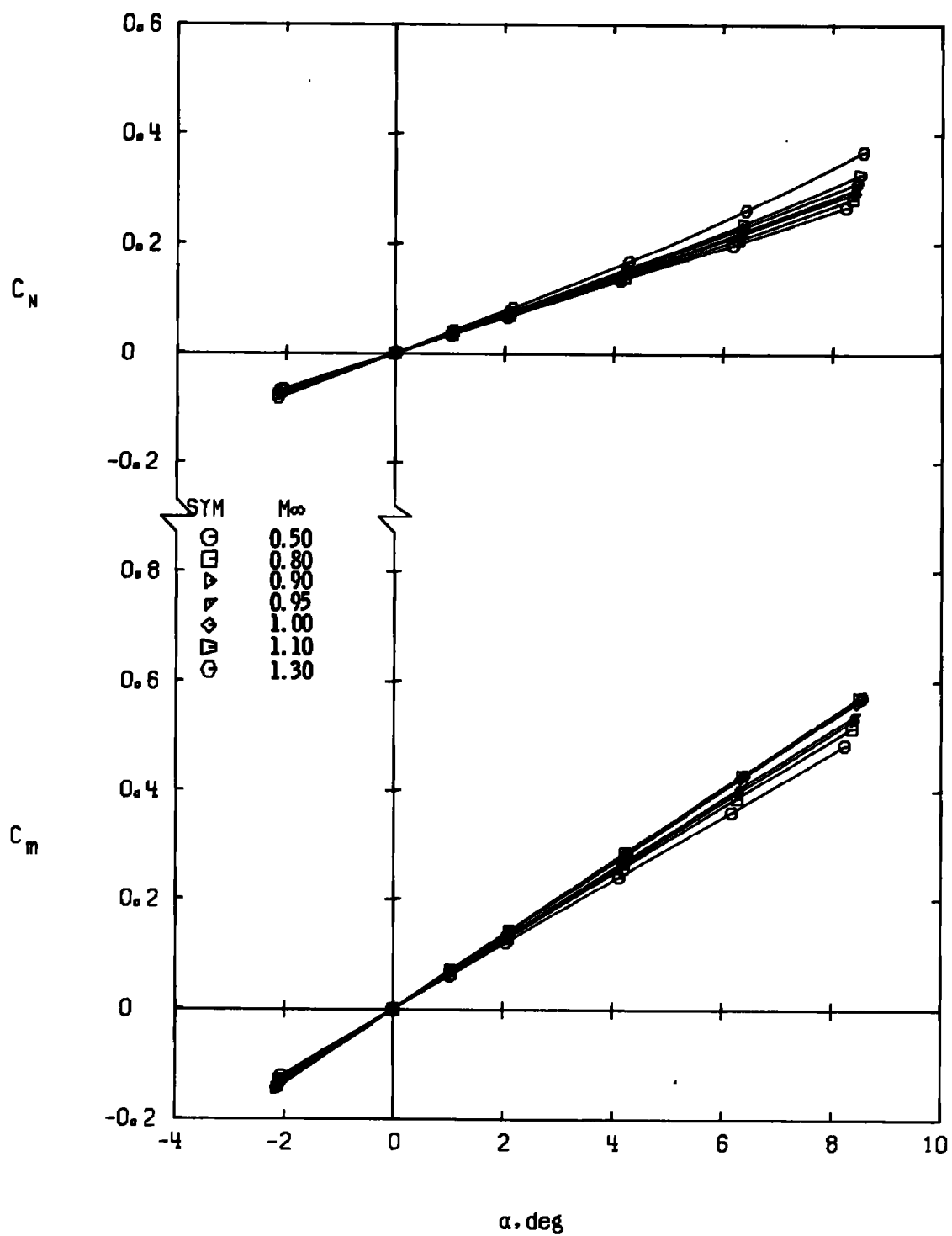
b. Configuration 1 Figure 5. Continued.
