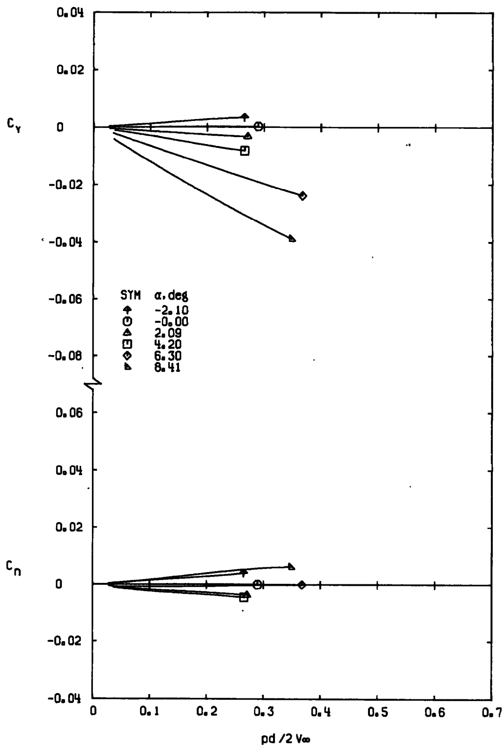
d. M_\infty = 0.95 Figure 8. Continued.
