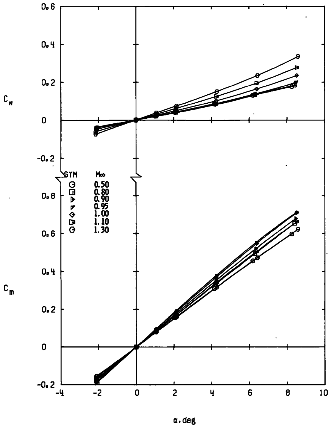
i. Configuration 8 Figure 5. Continued.
