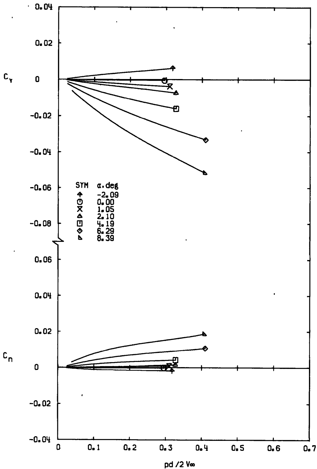
b. M_\infty = 0.80 Figure 12. Continued.
