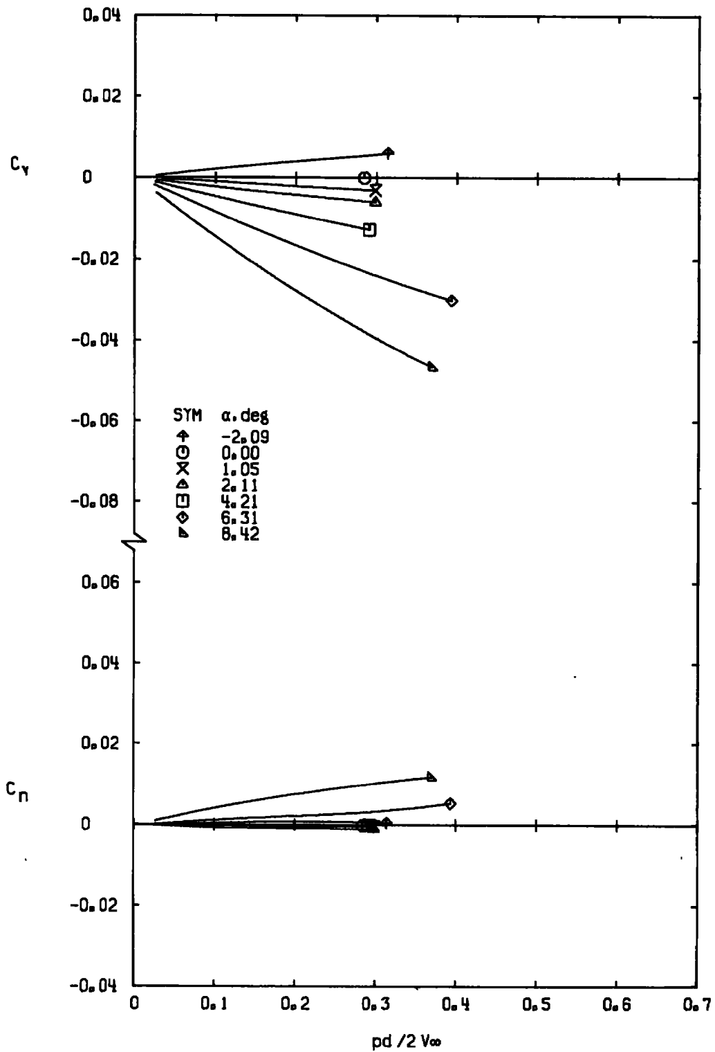
c. M_\infty = 0.90 Figure 9. Continued.
