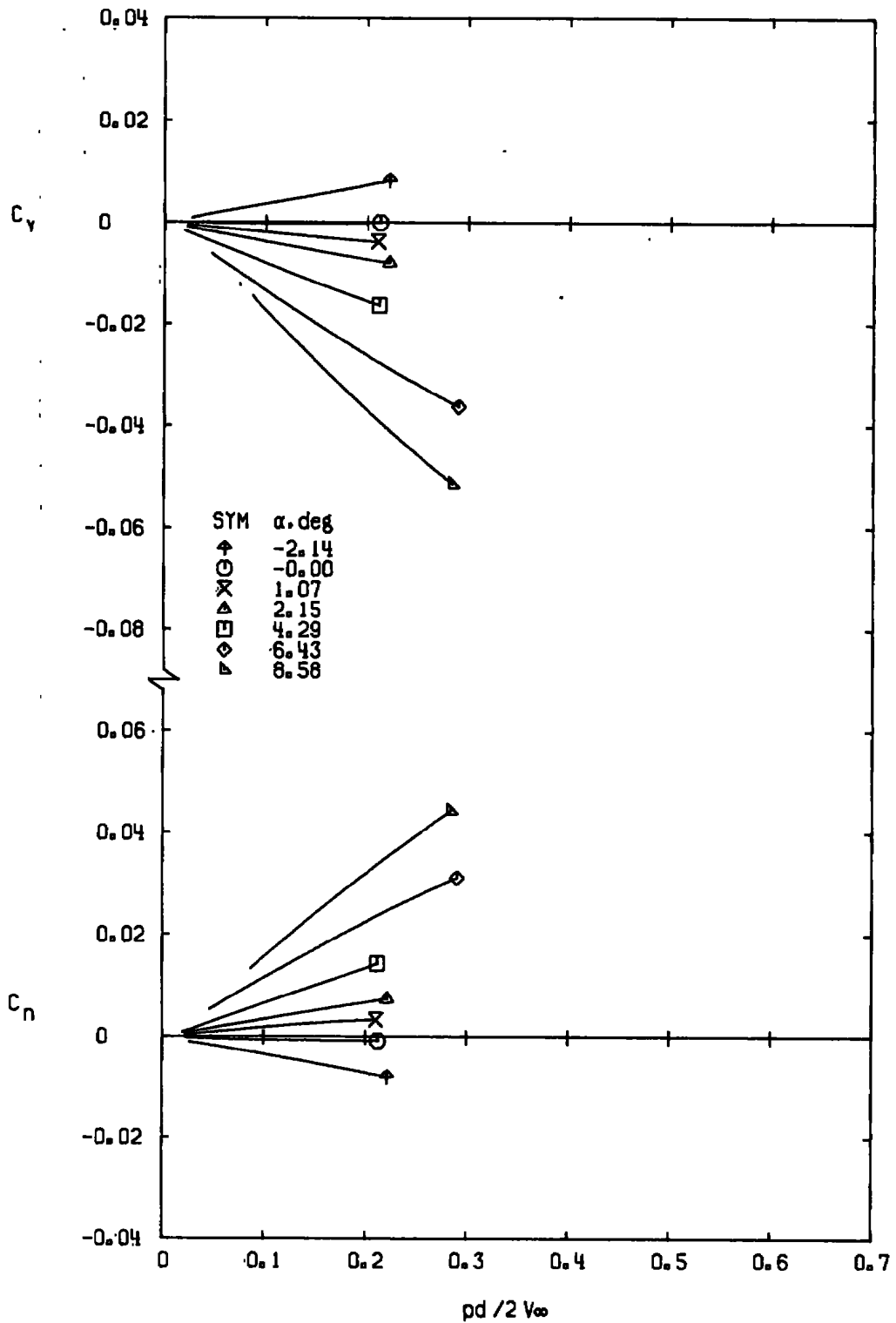
g. M_\infty = 1.30 Figure 16. Concluded.
