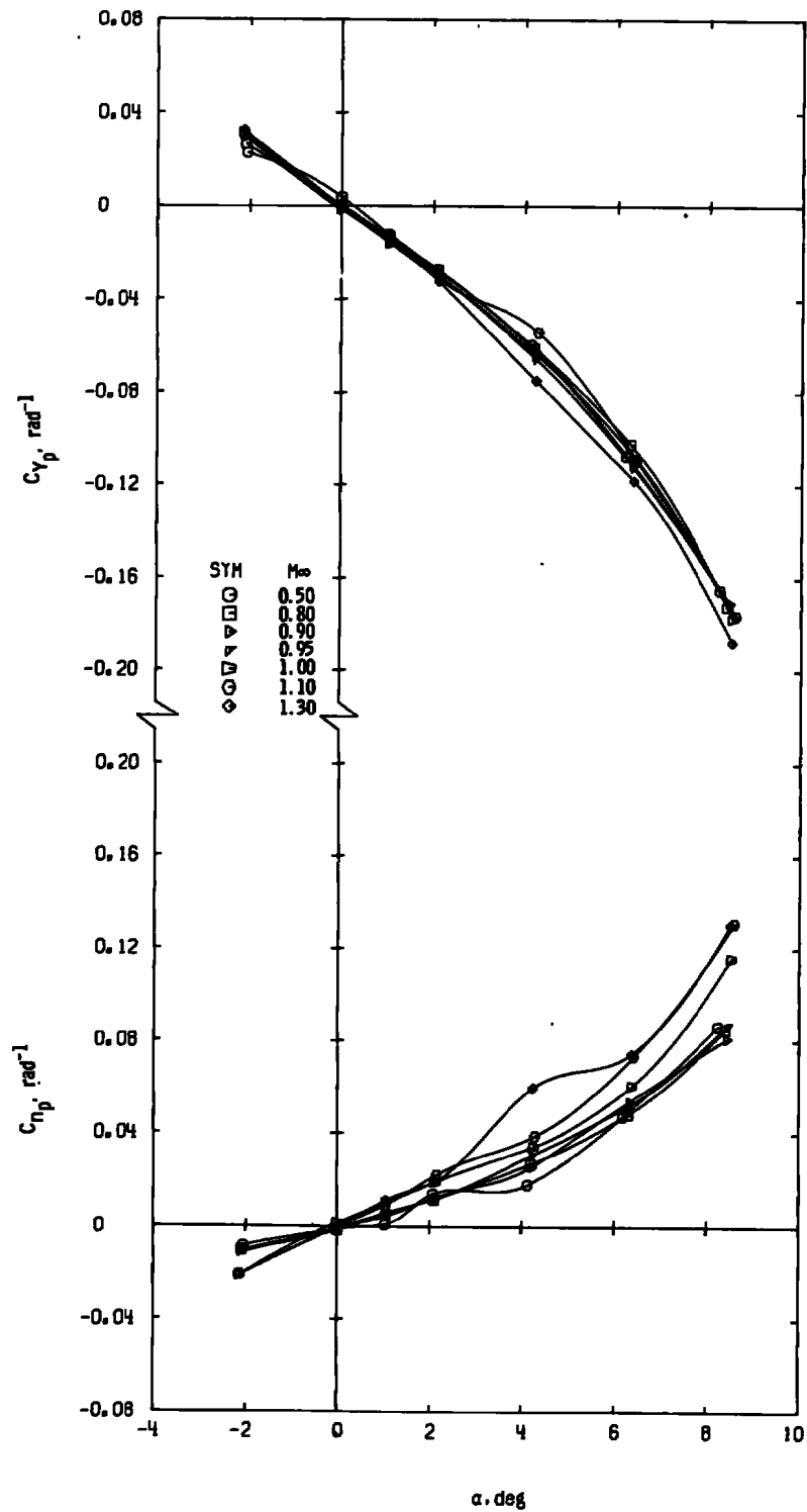
c. Configuration 2 Figure 18. Continued.
