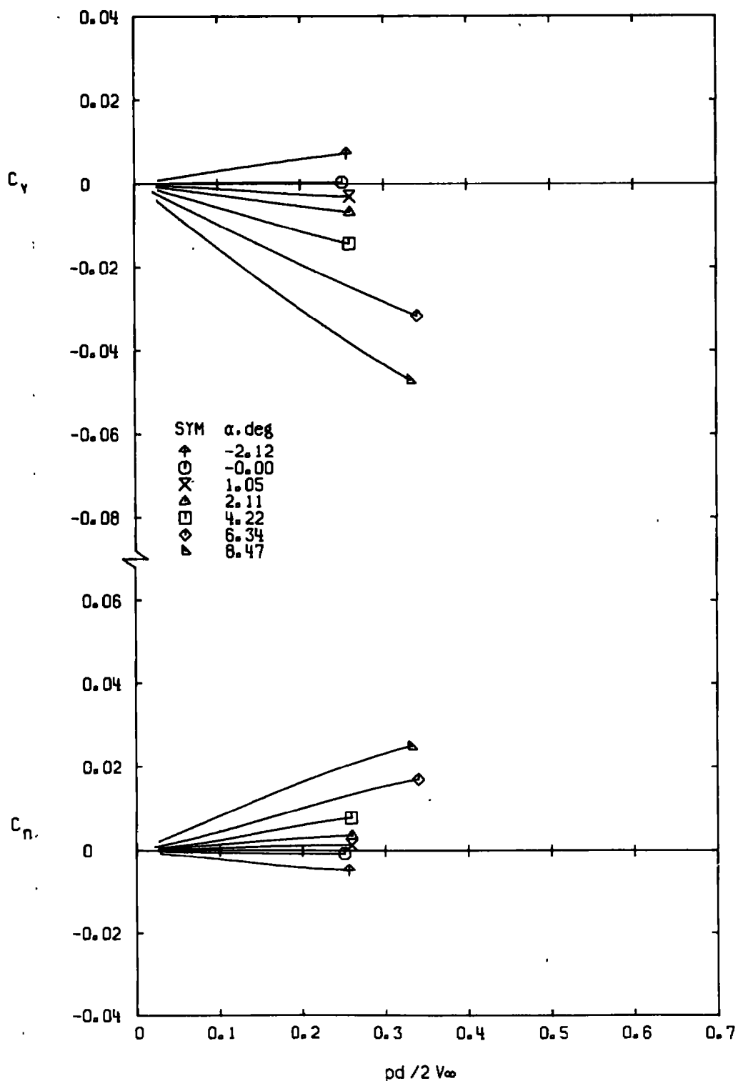
e. M_\infty = 1.00 Figure 12. Continued.
