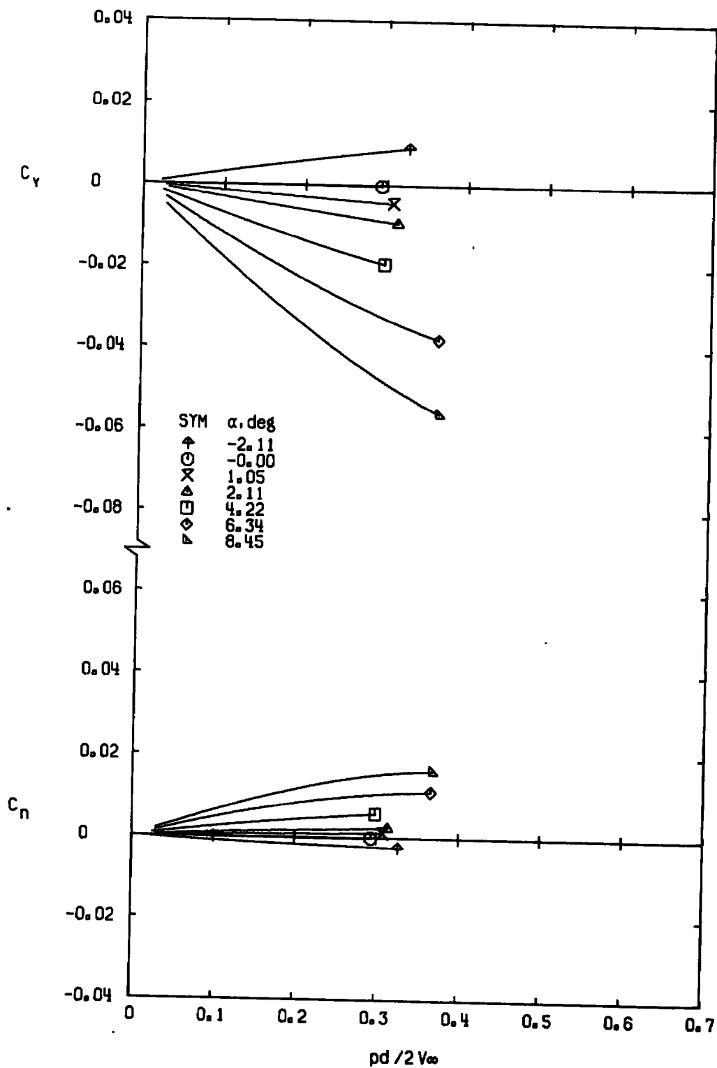
d. M_\infty = 0.95 Figure 14. Continued.
