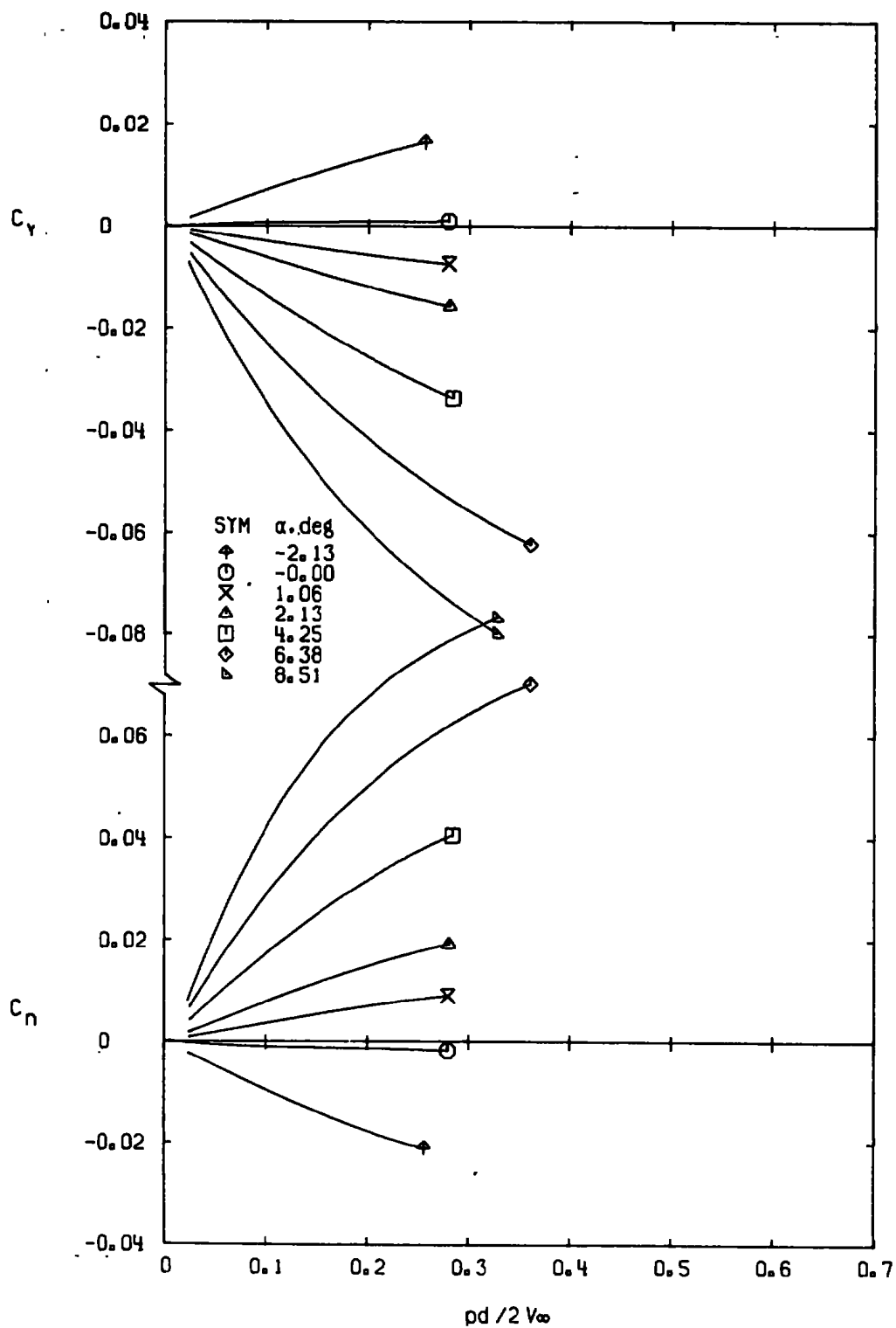
e. M_\infty = 1.00 Figure 16. Continued.
