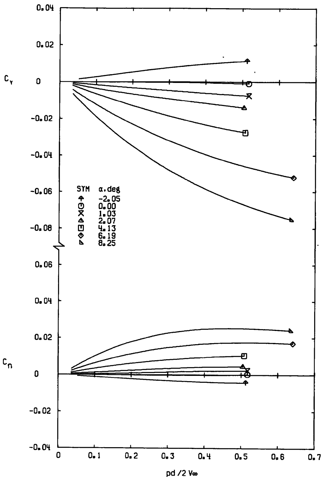
Figure 13. Variation of C_Y and C_N with pd/2V_\infty for Configuration 5.
