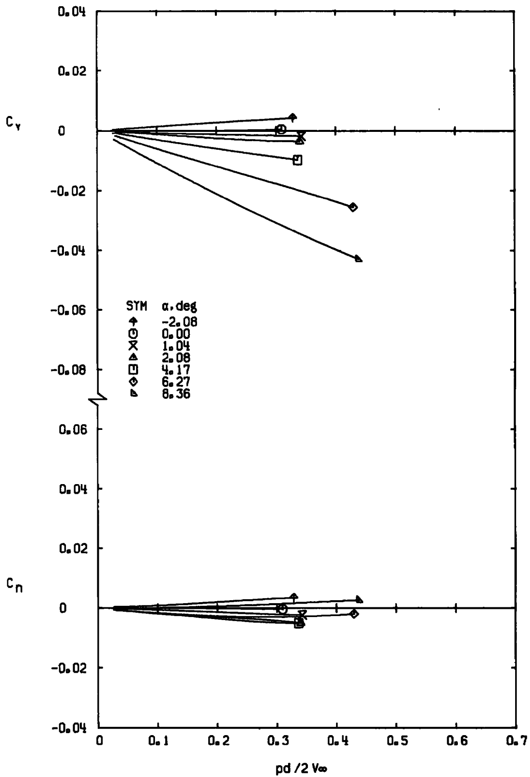
b. M_\infty = 0.80 Figure 8. Continued.
