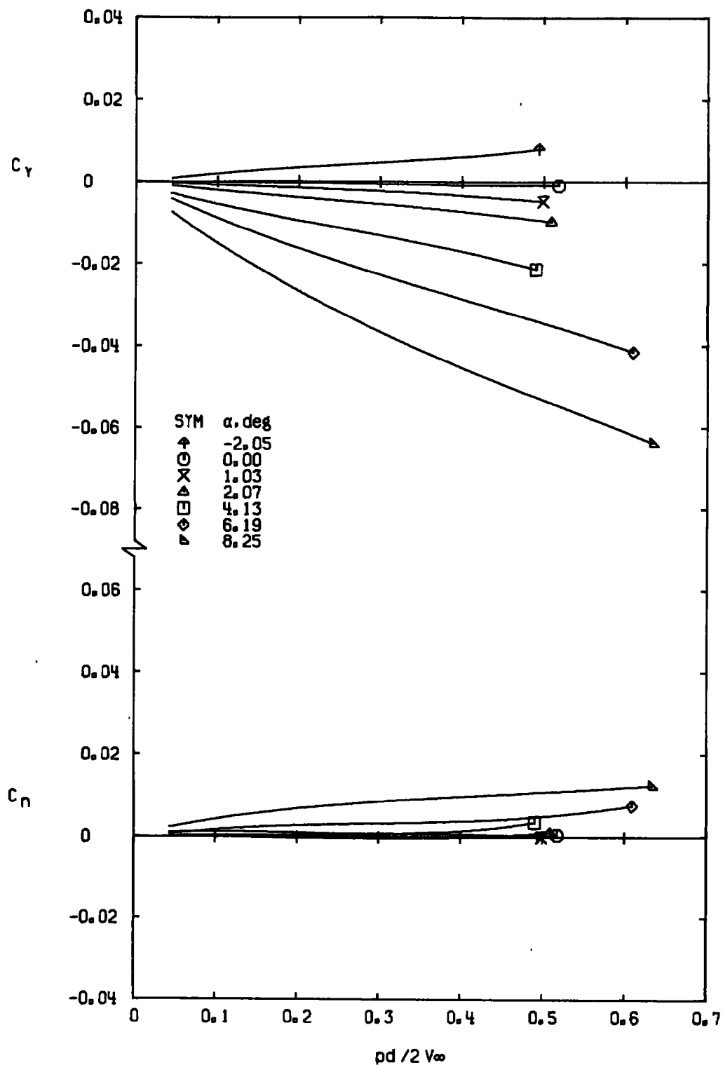
Figure 9. Variation of C_Y and C_N with pd/2V_\infty for Configuration 1.
