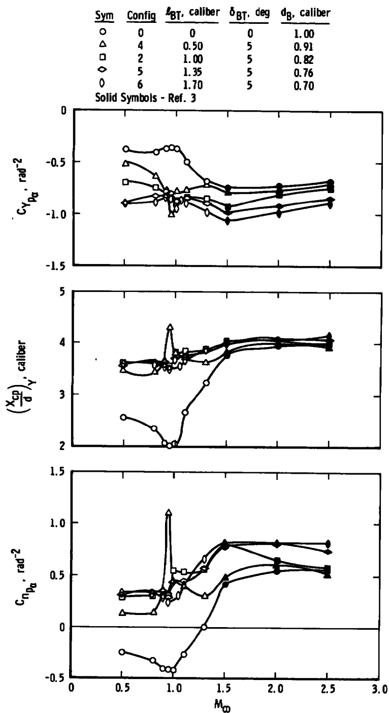
b. Effect of boattail length with a constant boattail angle Figure 19. Continued.
