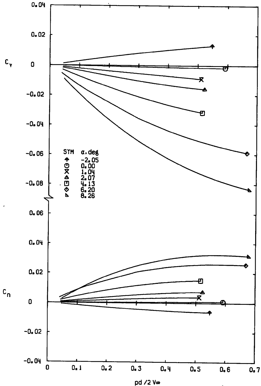
Figure 11. Variation of C_Y and C_N with pd/2V_\infty for Configuration 3.
