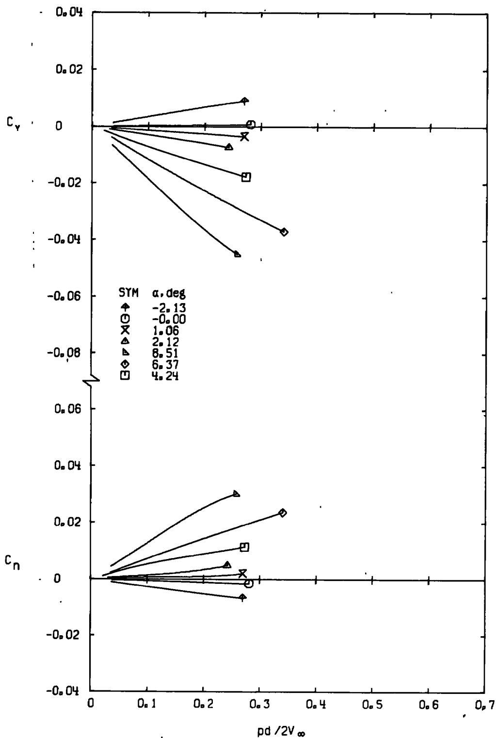
e. M_\infty = 1.00 Figure 10. Continued.
