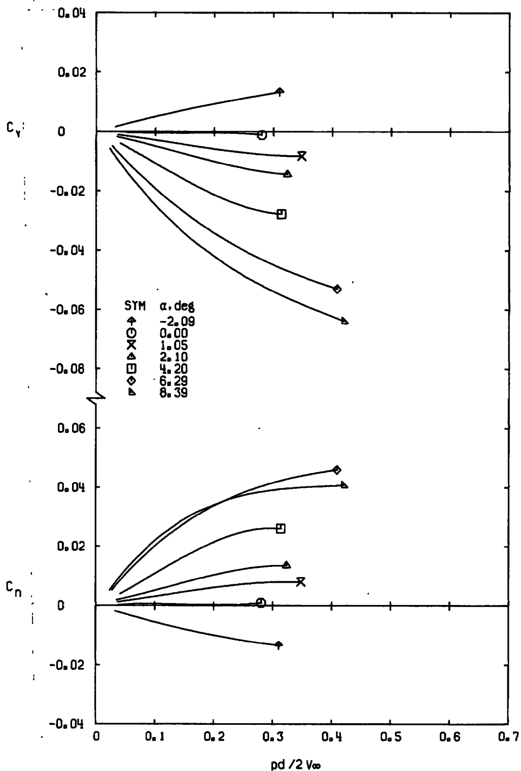
b. M_\infty = 0.80 Figure 15. Continued.
