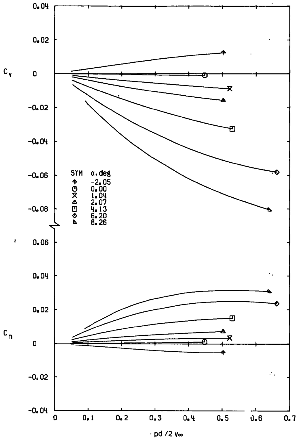
Figure 17. Variation of C_Y and C_N with pd/2V_\infty for Configuration 9.
