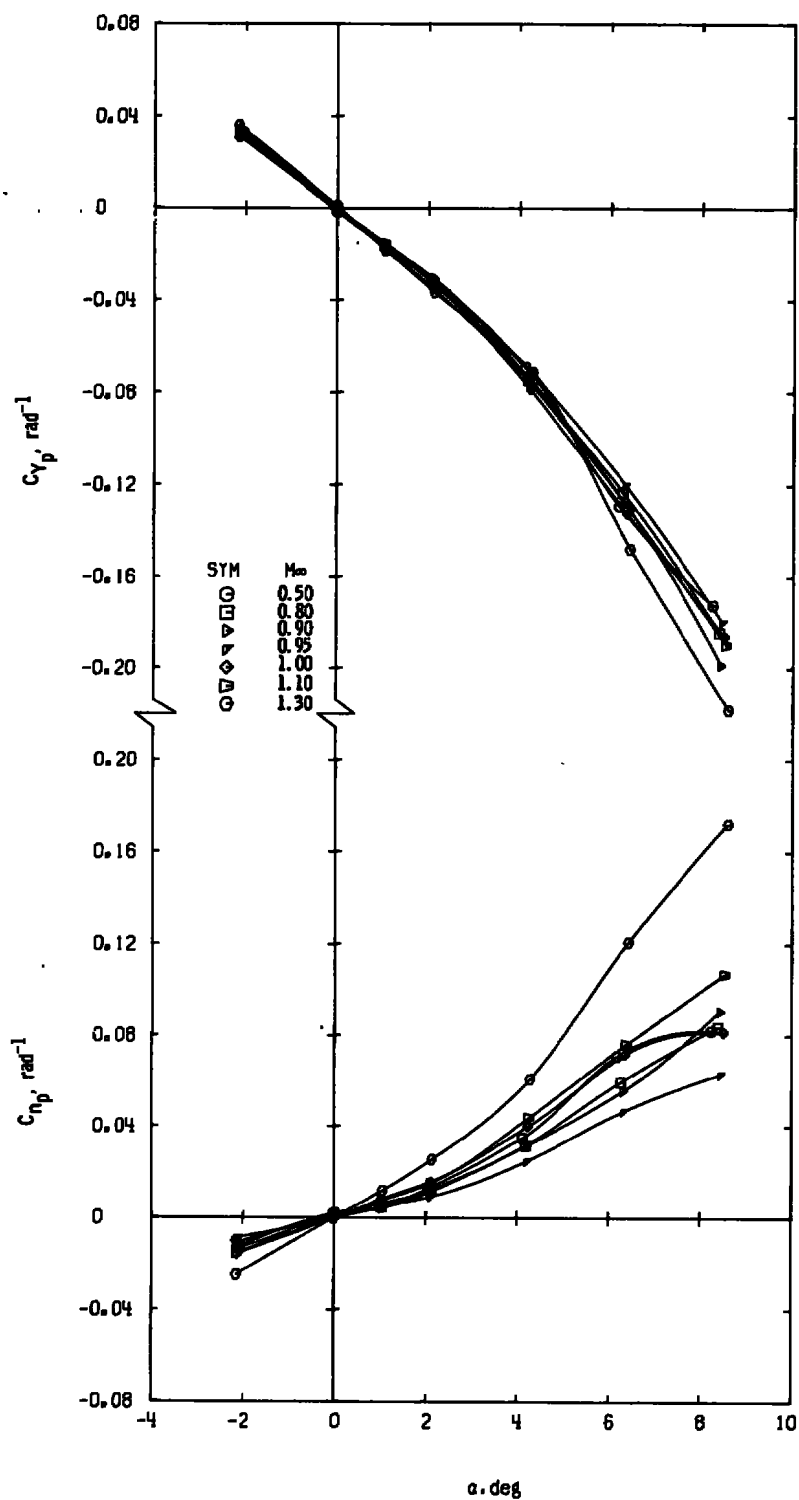
g. Configuration 6 Figure 18. Continued.
