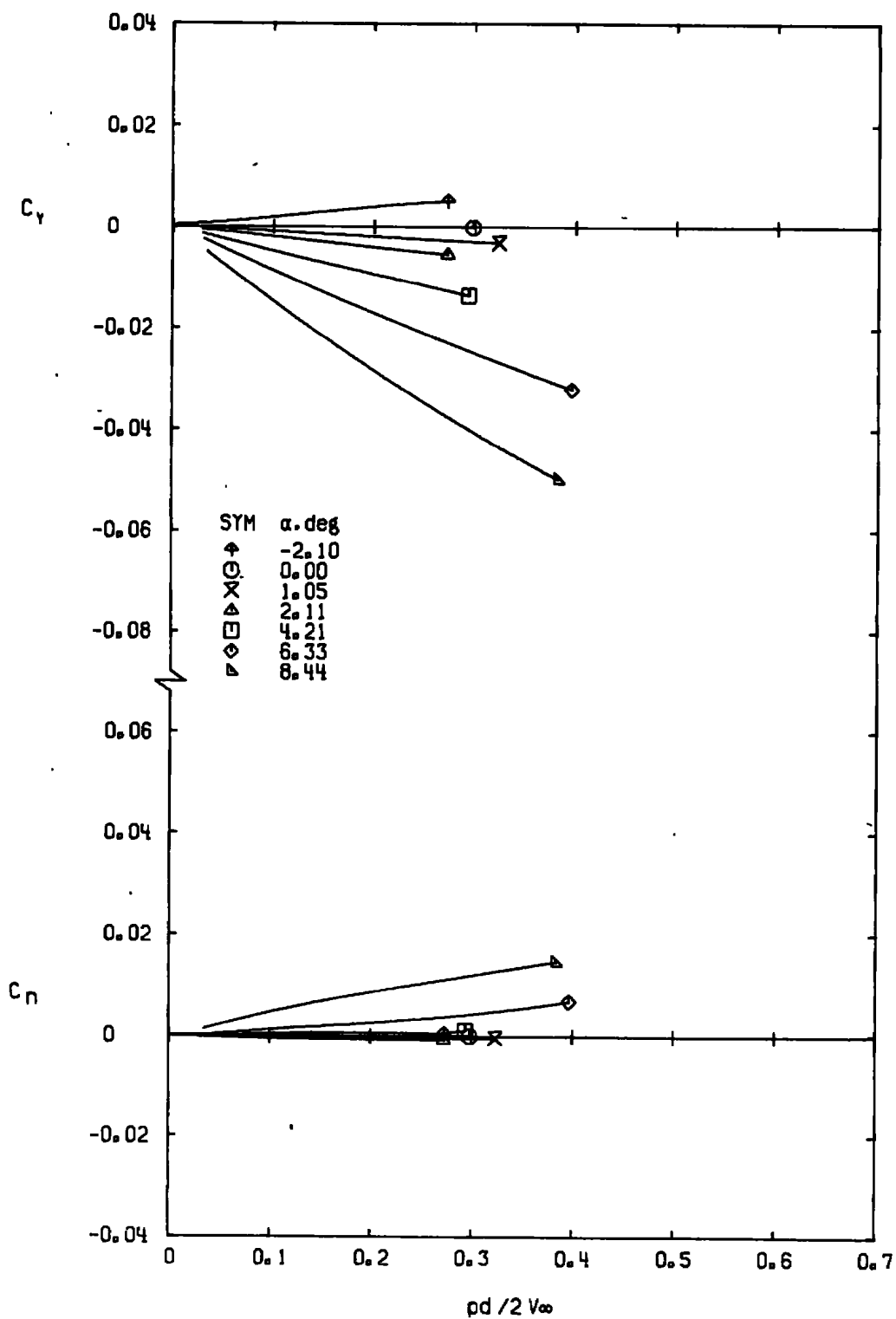
d. M_\infty = 0.95 Figure 9. Continued.
