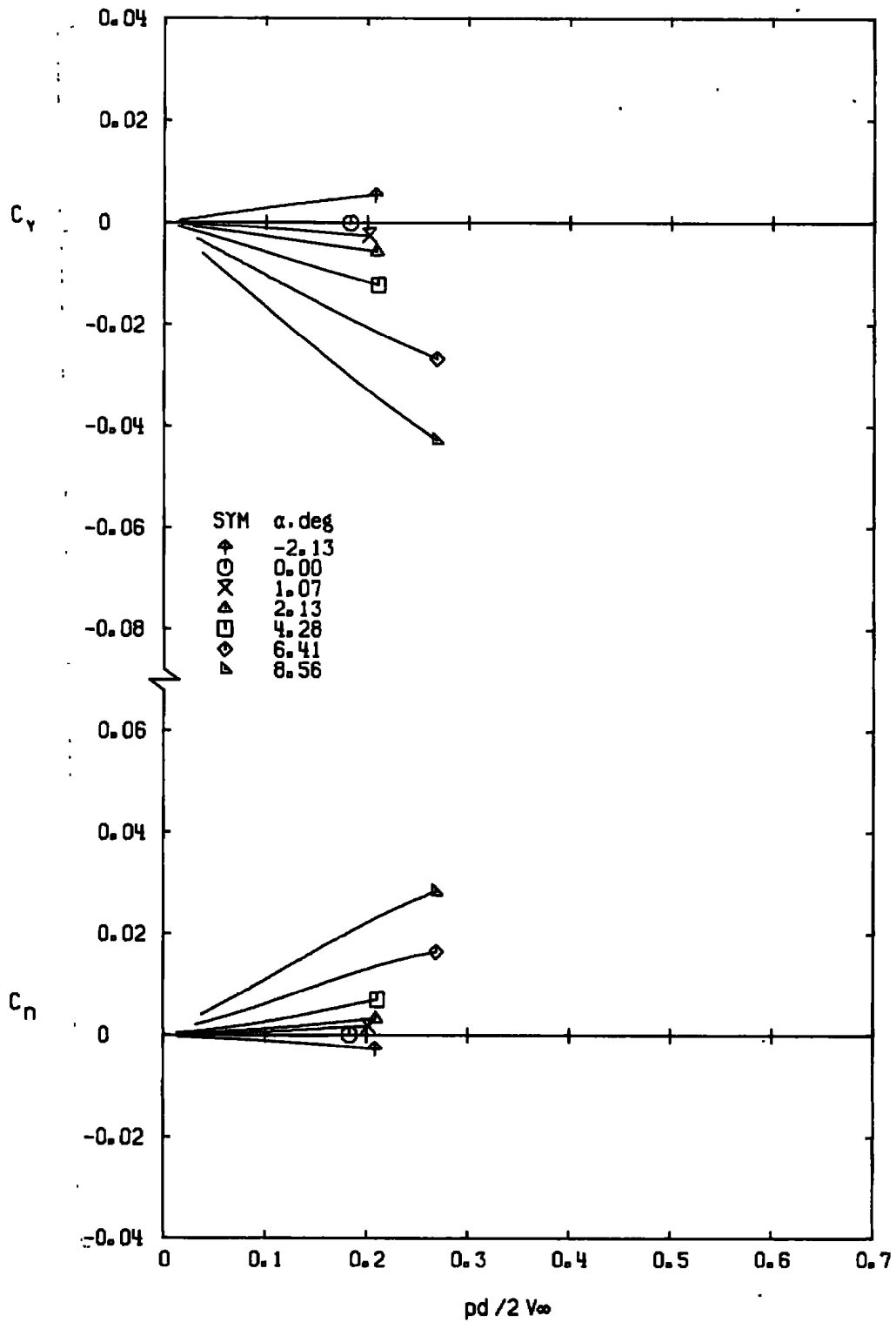
g. M_\infty = 1.30 Figure 12. Concluded.
