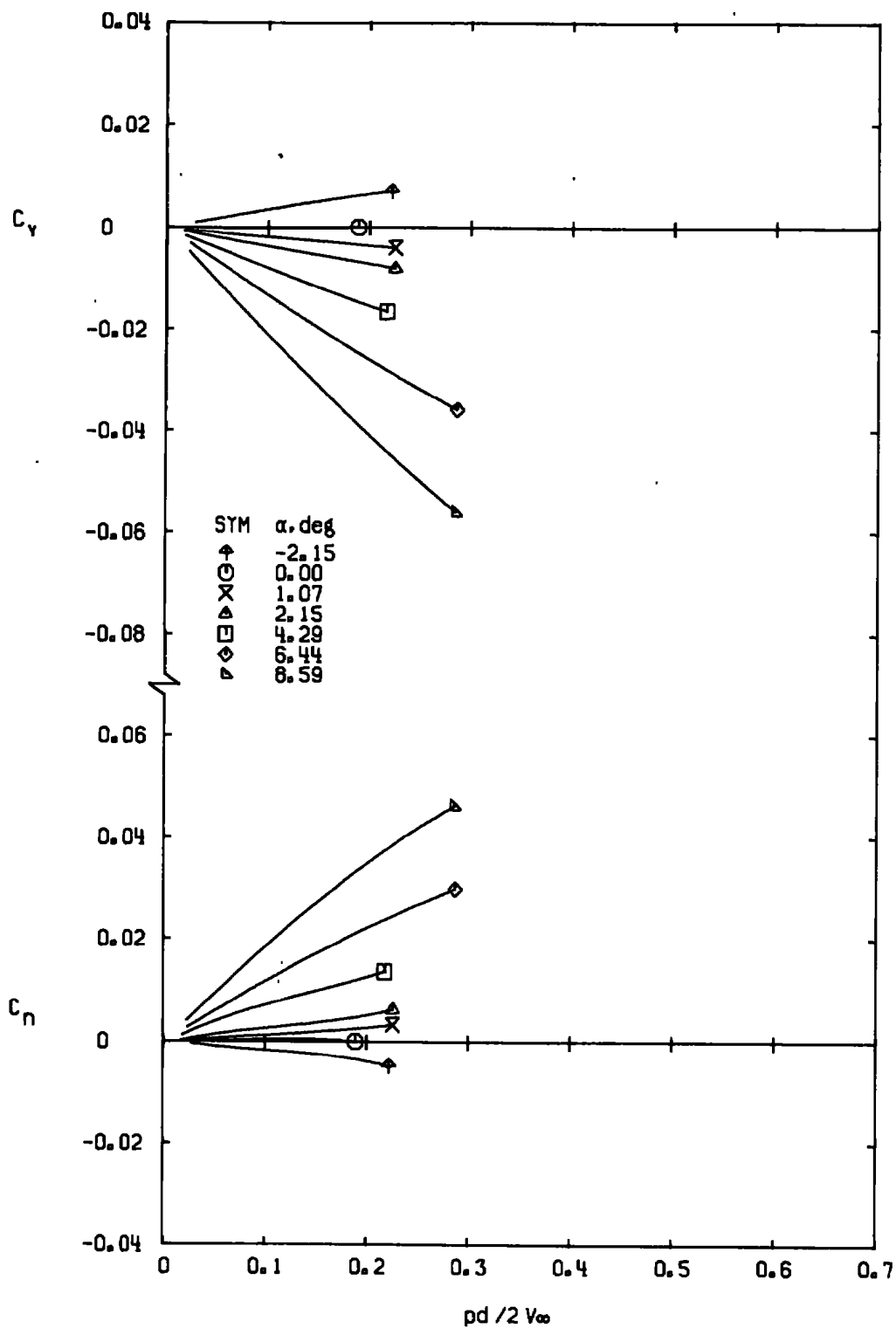
g. M_\infty = 1.30 Figure 11. Concluded.
