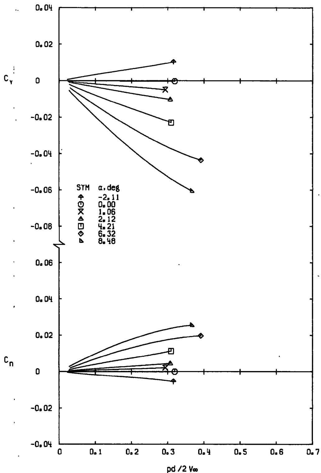
d. M_\infty = 0.95 Figure 17. Continued.
