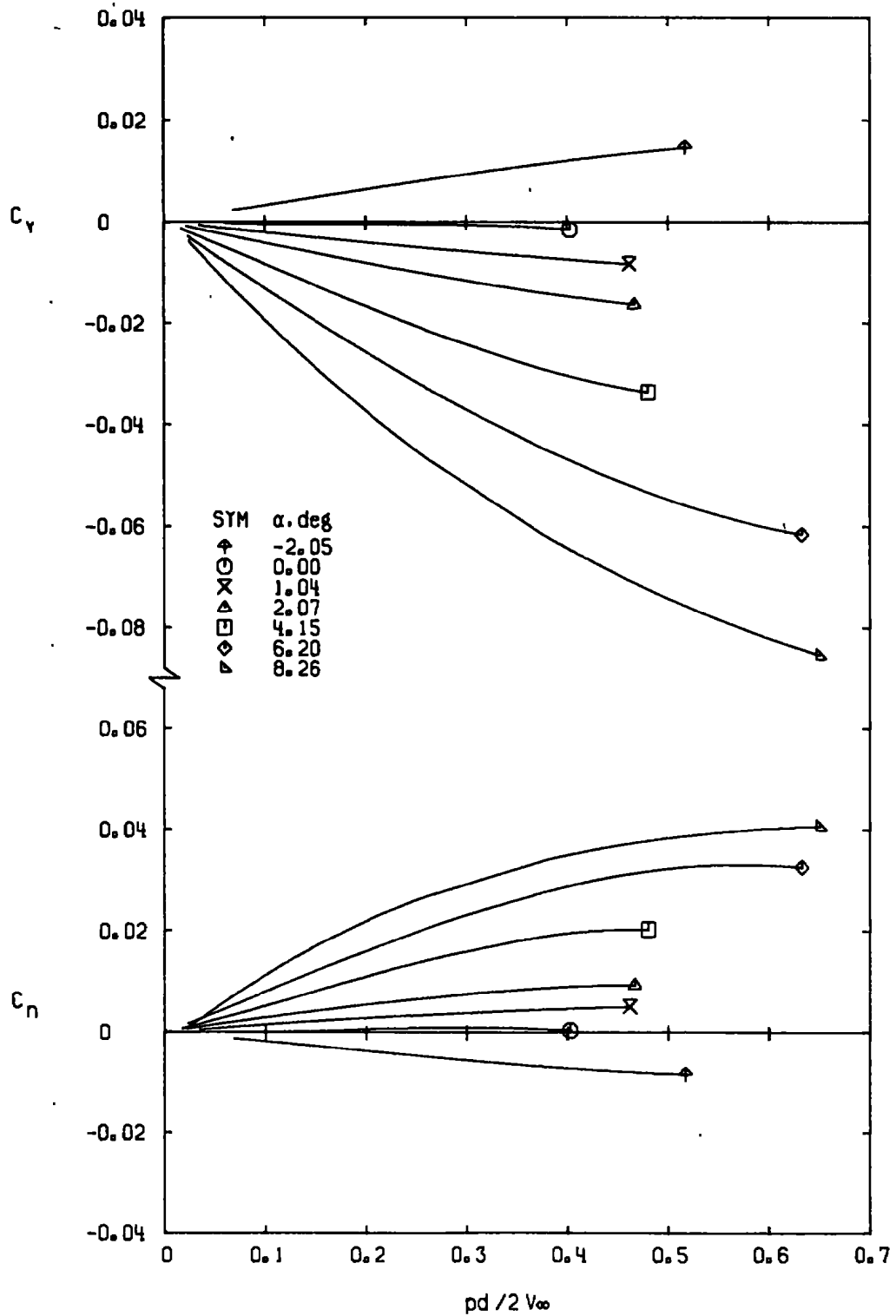
Figure 16. Variation of C_Y and C_N with pd/2V_\infty for Configuration 8.
