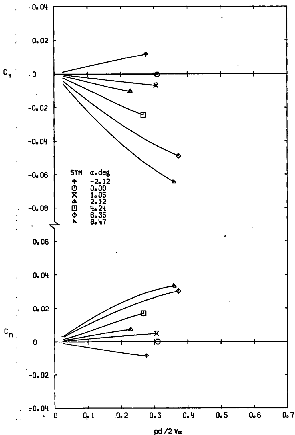
c. M_{\infty} = 0.90 Figure 16. Continued.
