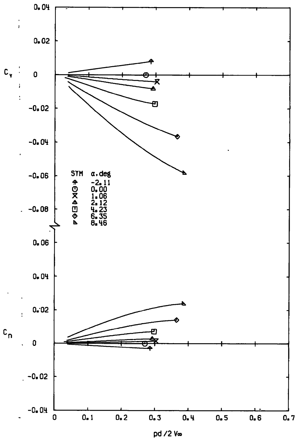
d. M_\infty = 0.95 Figure 13. Continued.
