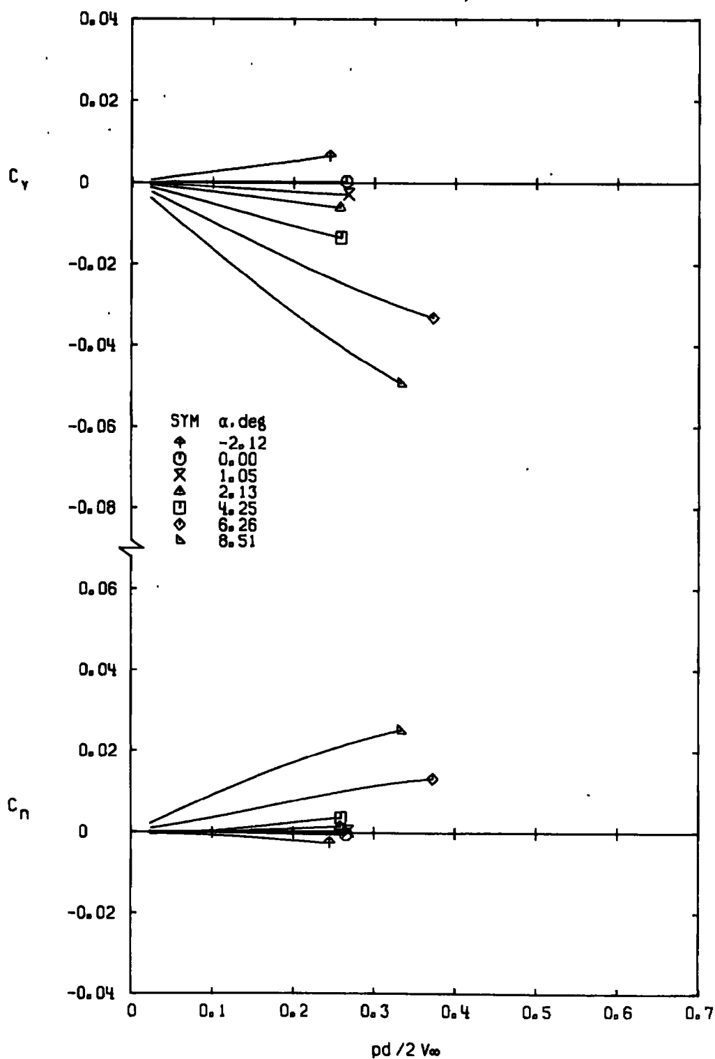
f. M_\infty = 1.10 Figure 9. Continued.
