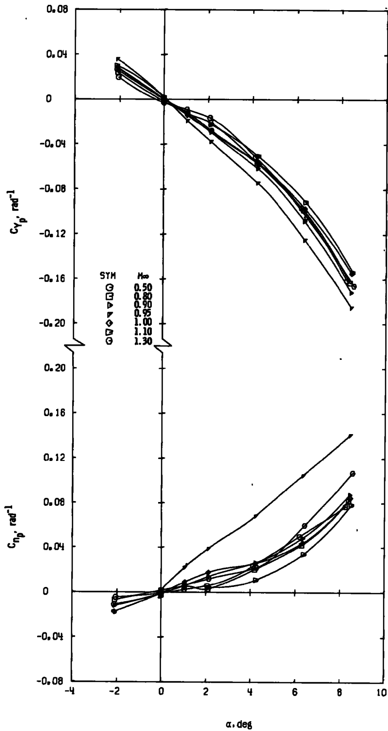
e. Configuration 4 Figure 18. Continued.
