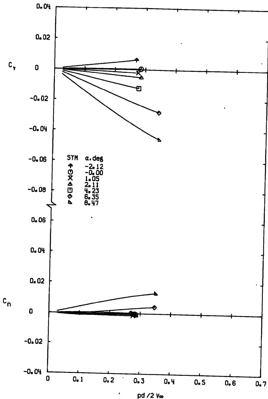
e. M_\infty = 1.00 Figure 9. Continued.
