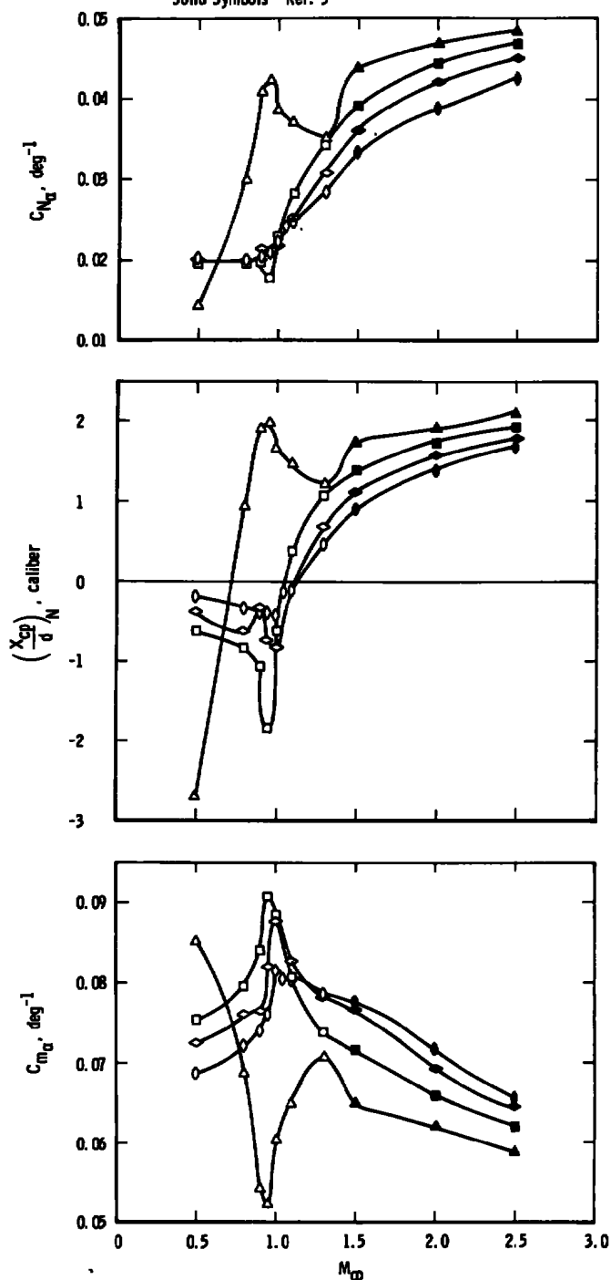
c. Effect of boattail length with a constant base diameter Figure 6. Concluded.
