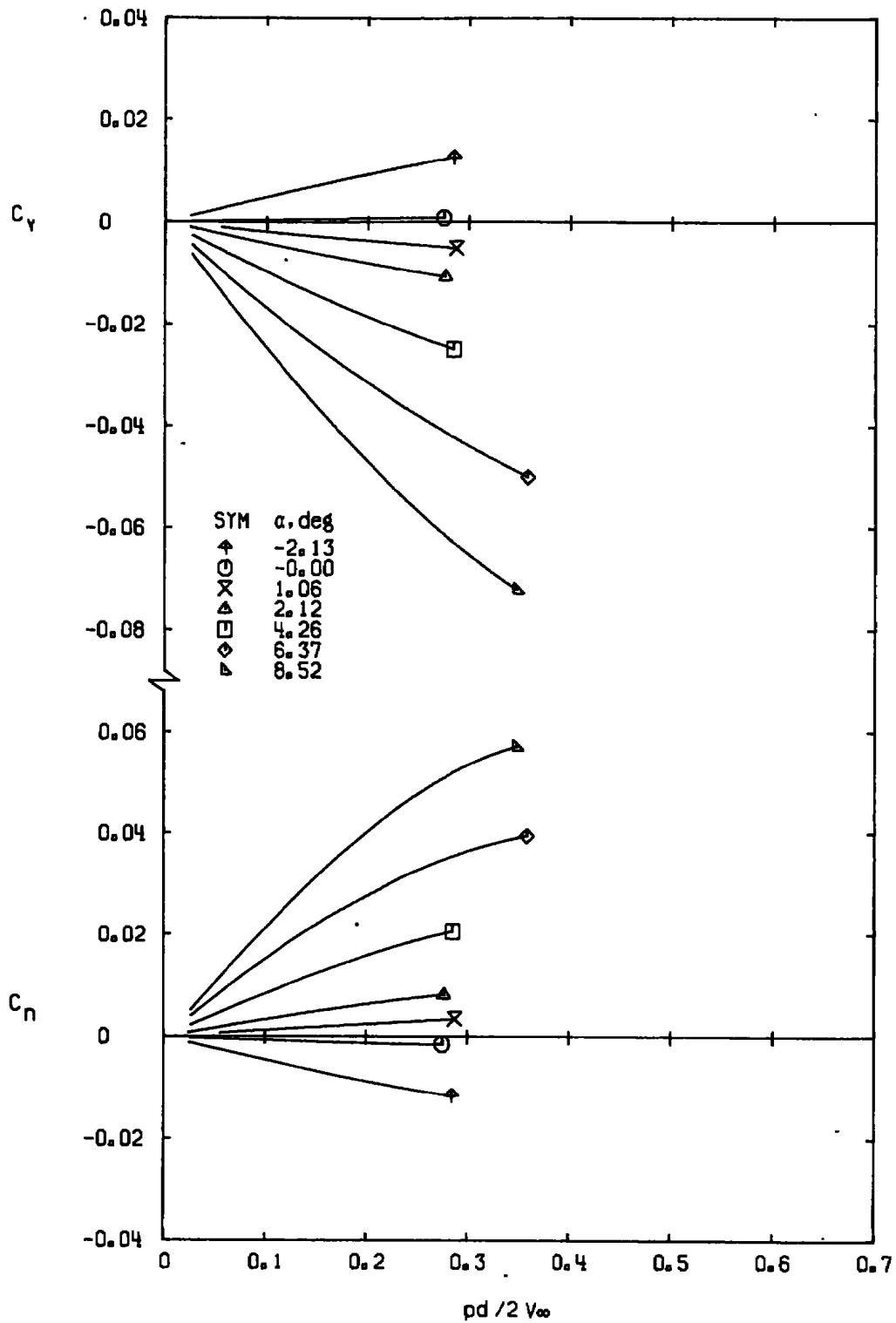
e. M_\infty = 1.00 Figure 17. Continued.
