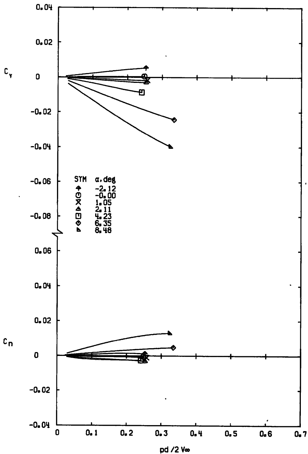
f. M_\infty = 1.10 Figure 8. Continued.
