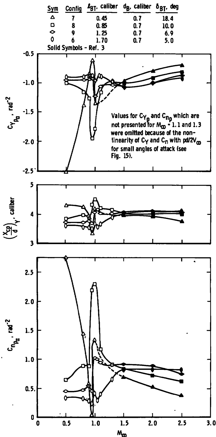
c. Effect of boattail length with a constant base diameter
