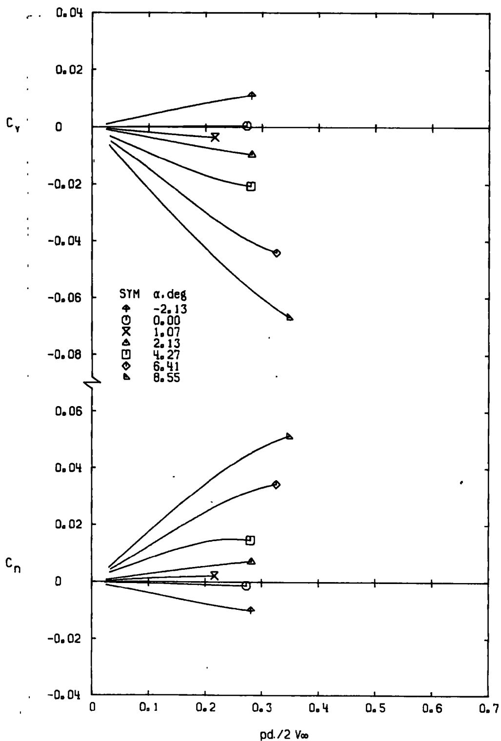
f. M_\infty = 1.10 Figure 17. Continued.
