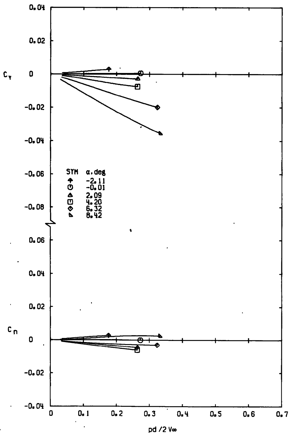
e. M_\infty = 1.00 Figure 8. Continued.
