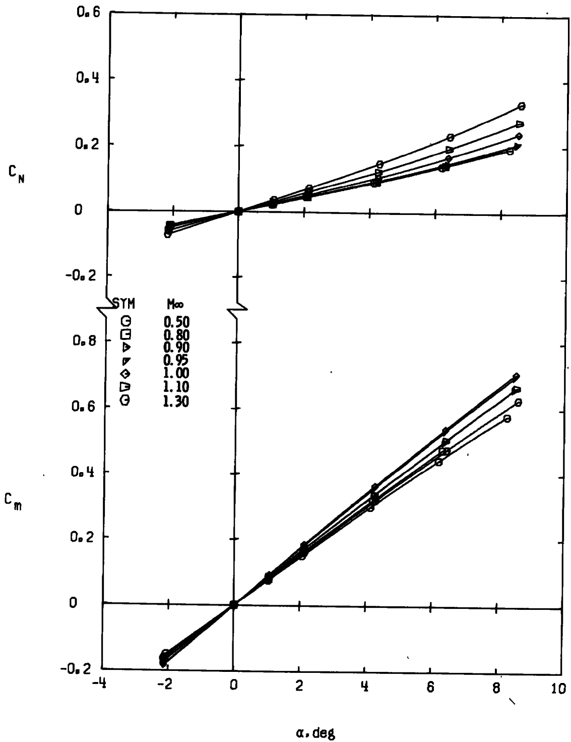
d. Configuration 3 Figure 5. Continued.
