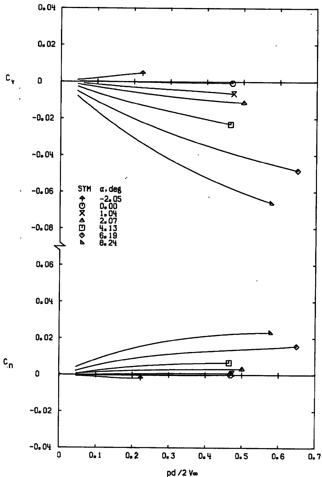
Figure 10. Variation of C_Y and C_n with pd/2V_\infty for Configuration 2.
