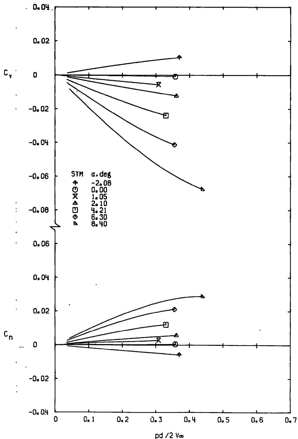
b. M_\infty = 0.80 Figure 17. Continued.
