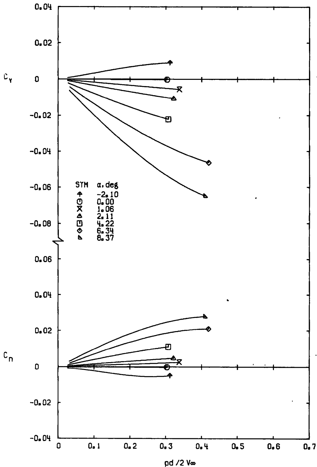
c. M_\infty = 0.90 Figure 17. Continued.
