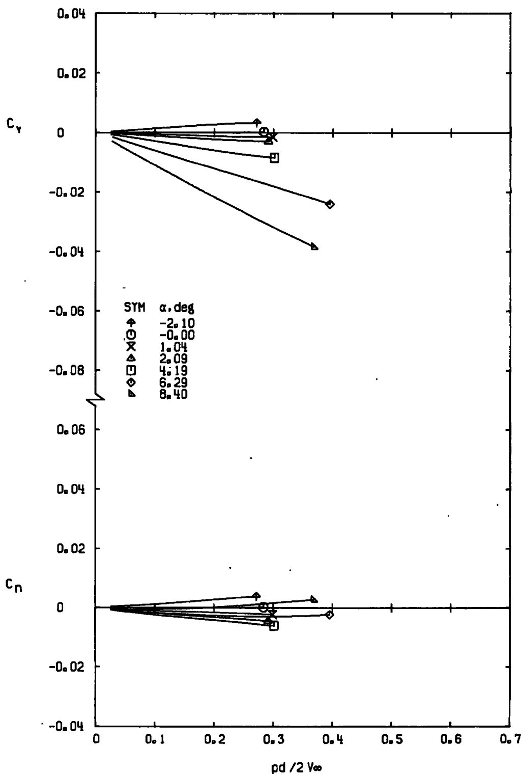
c. M_\infty = 0.90 Figure 8. Continued.
