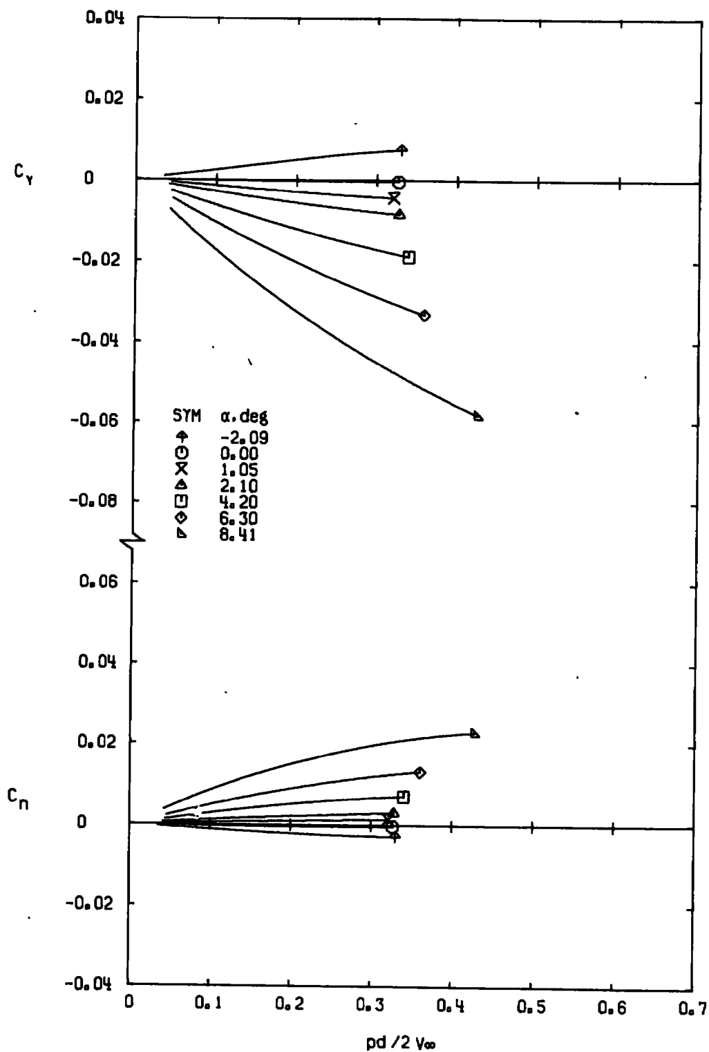
b. M_\infty = 0.80 Figure 10. Continued.
