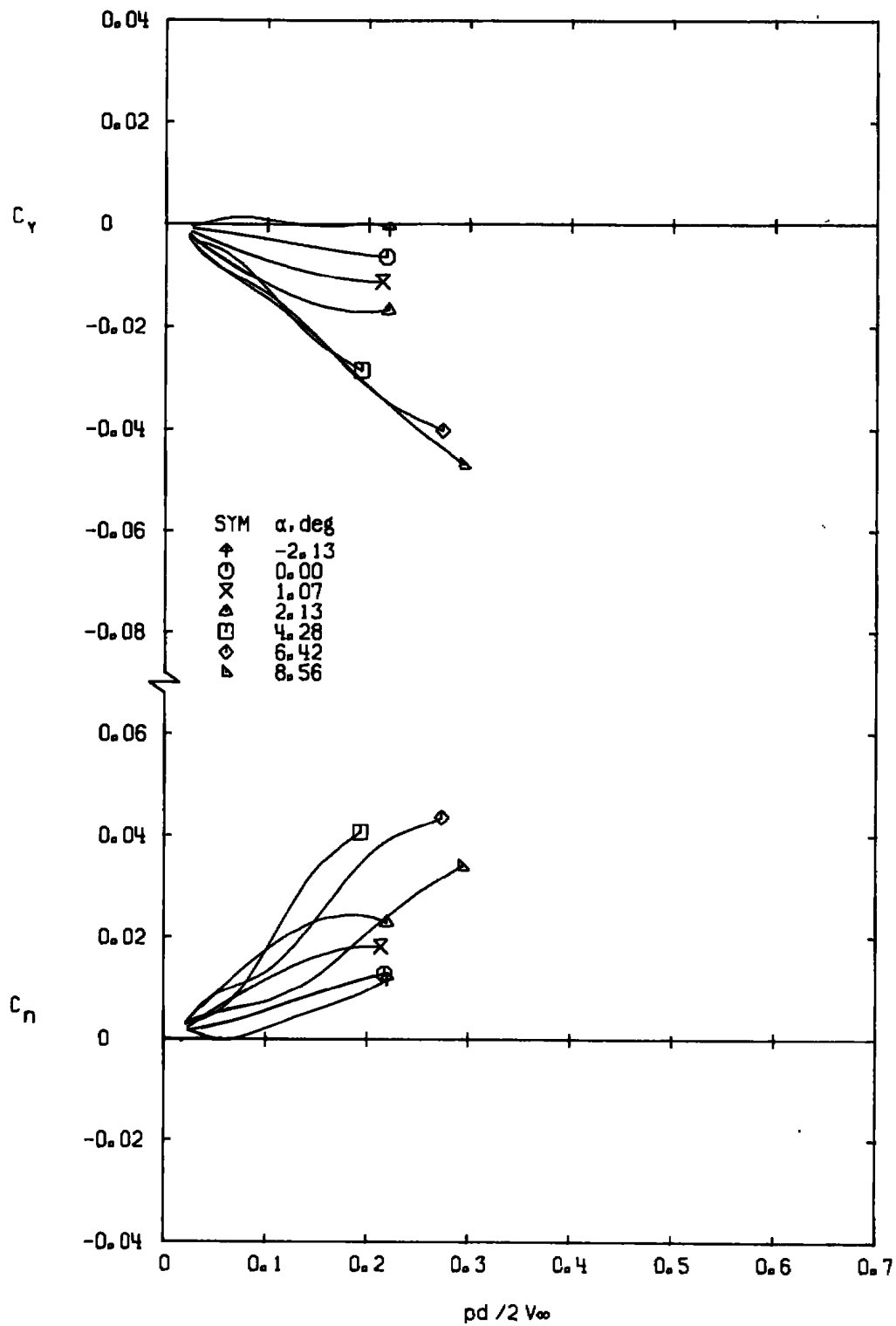
g. M_\infty = 1.30 Figure 15. Concluded.
