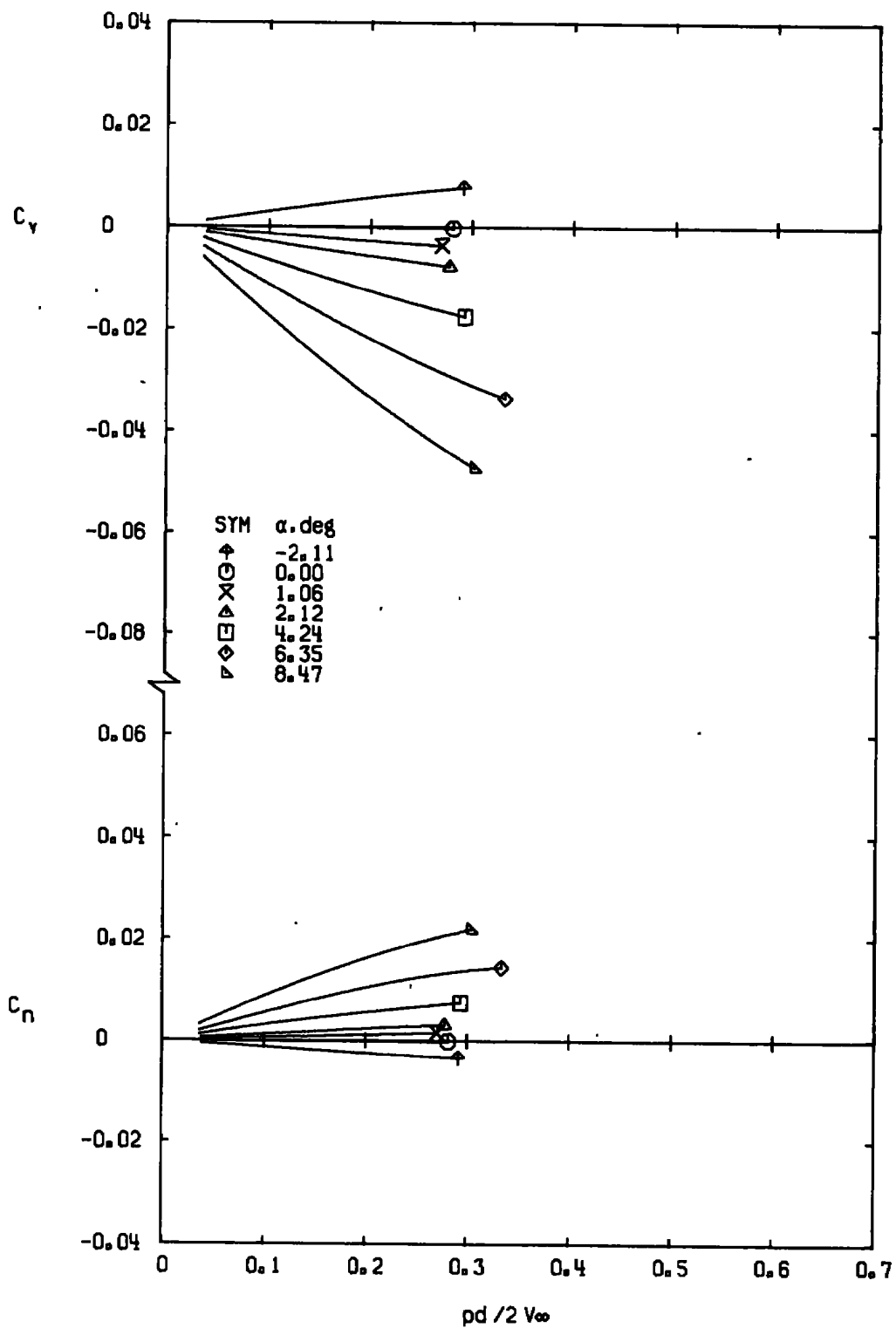
d. M_\infty = 0.95 Figure 10. Continued.
