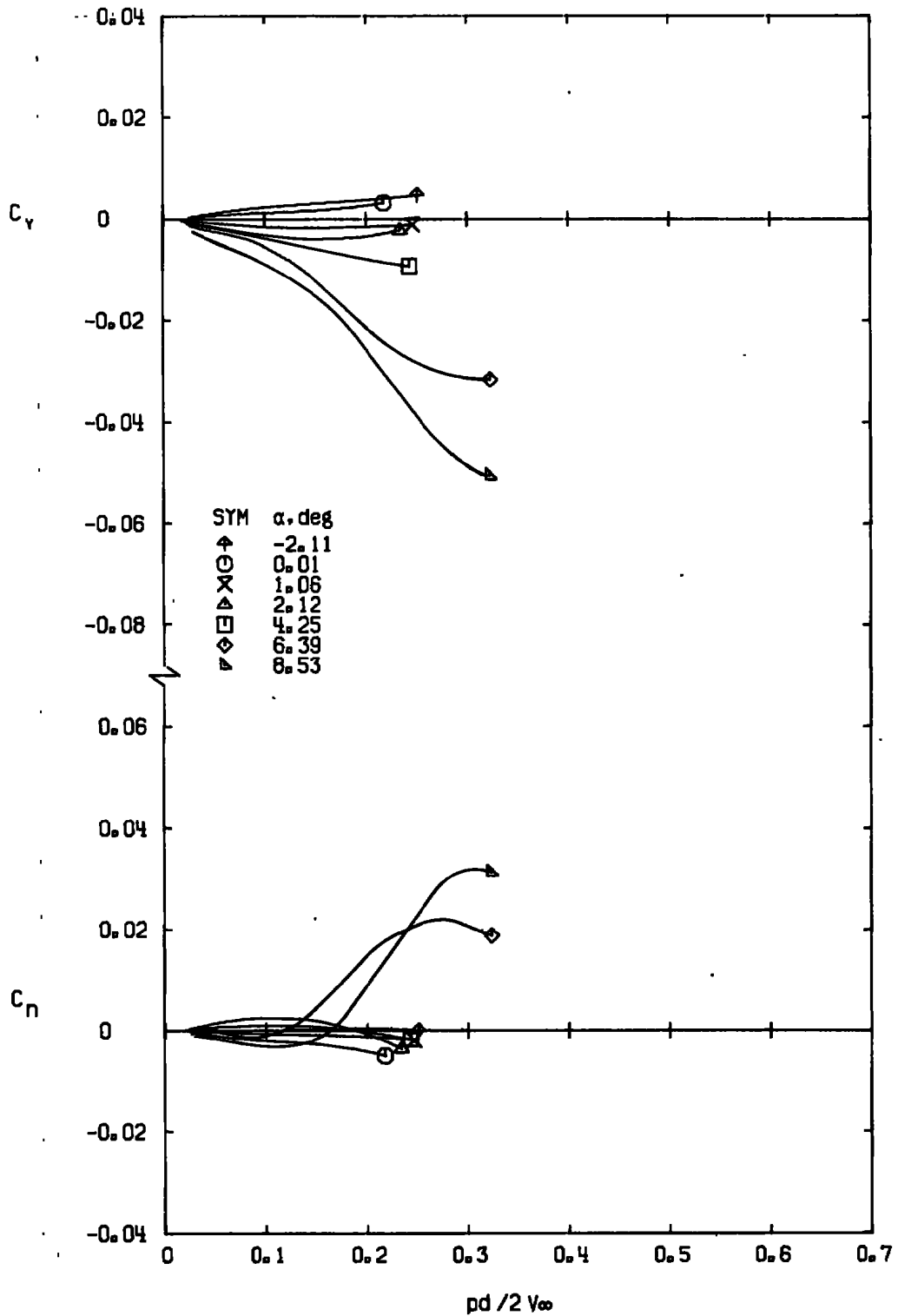
f. M_\infty = 1.10 Figure 15. Continued.
