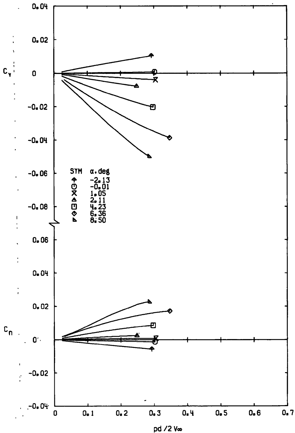
e. M_\infty = 1.00 Figure 14. Continued.
