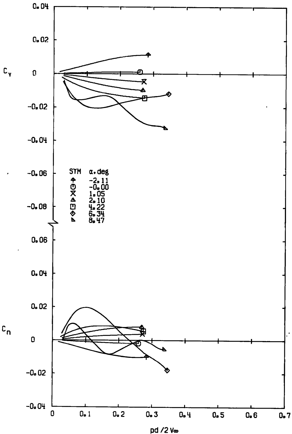
e. M_\infty = 1.00 Figure 15. Continued.
