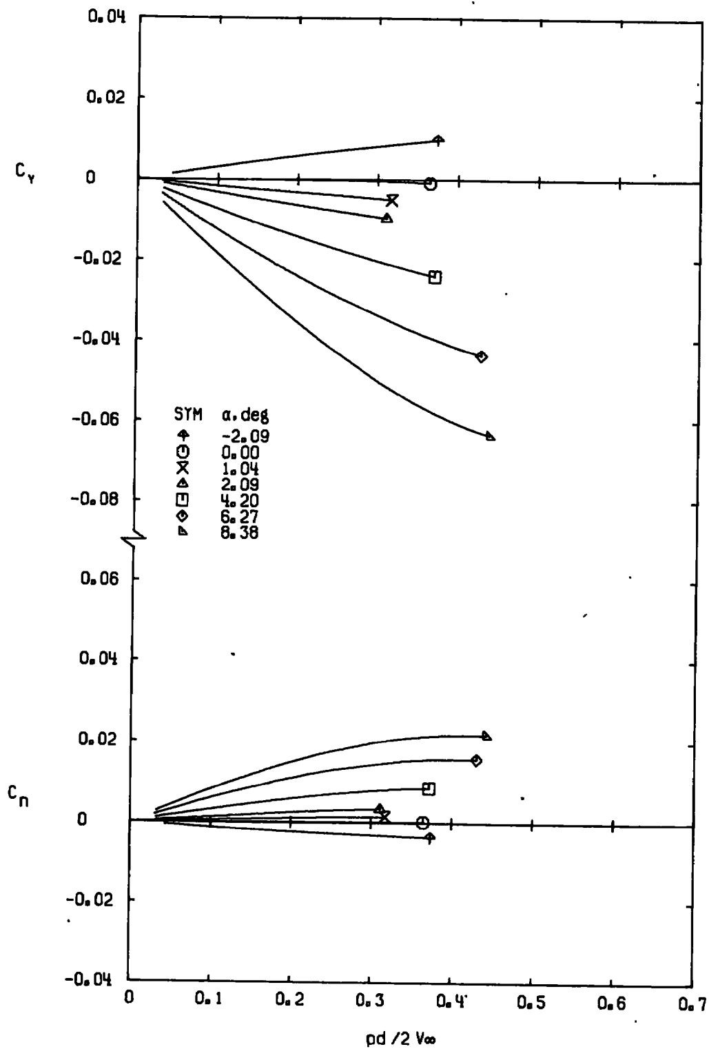
b. M_\infty = 0.80 Figure 14. Continued.
