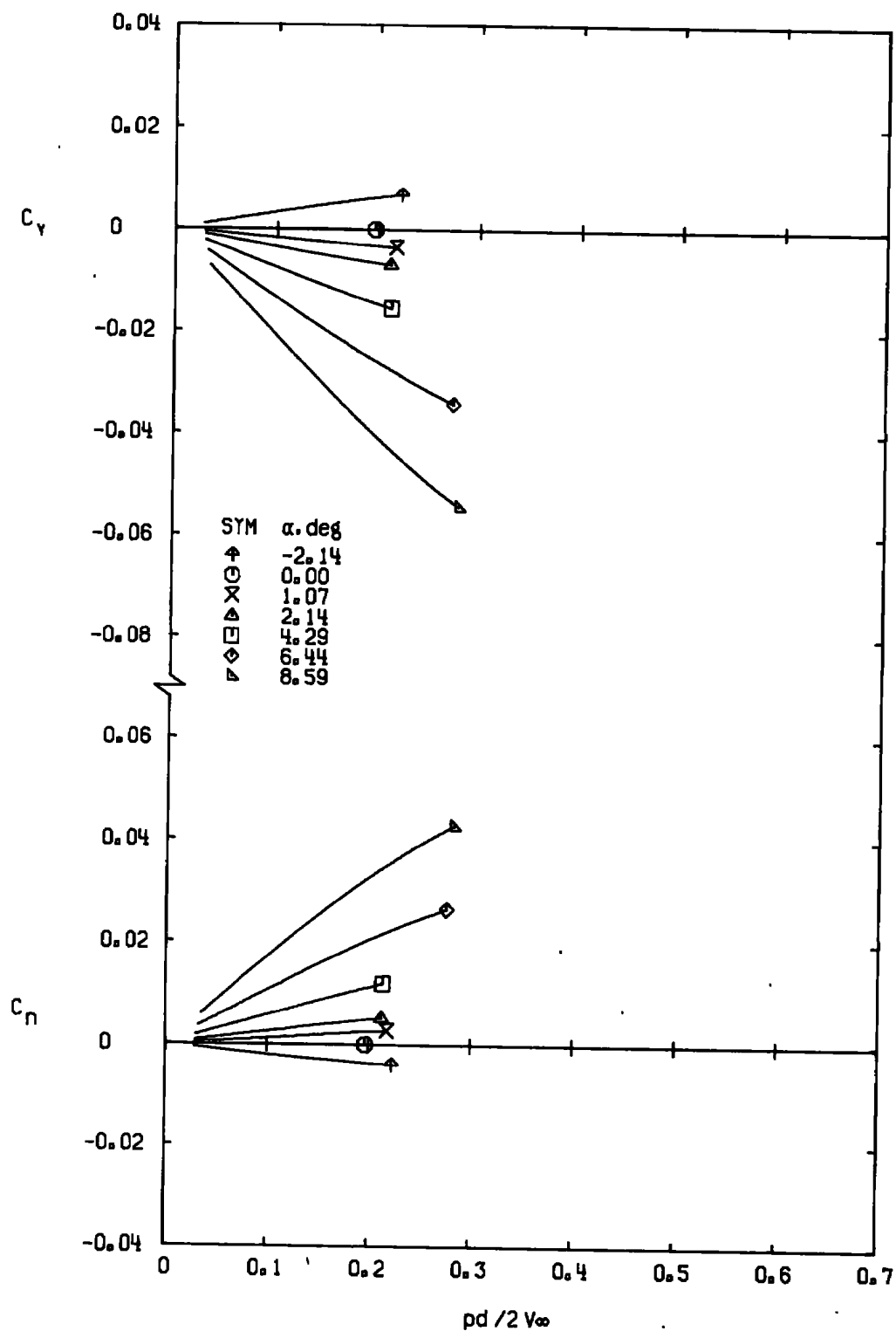
g. M_\infty = 1.30 Figure 13. Concluded.
