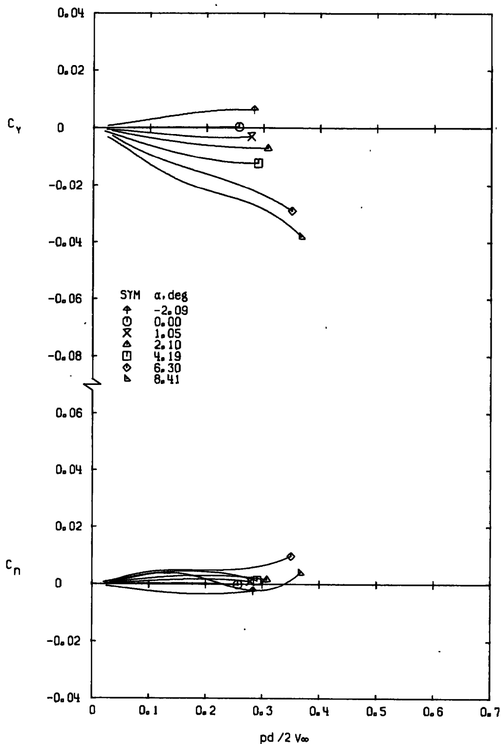
c. M_\infty = 0.90 Figure 15. Continued.
