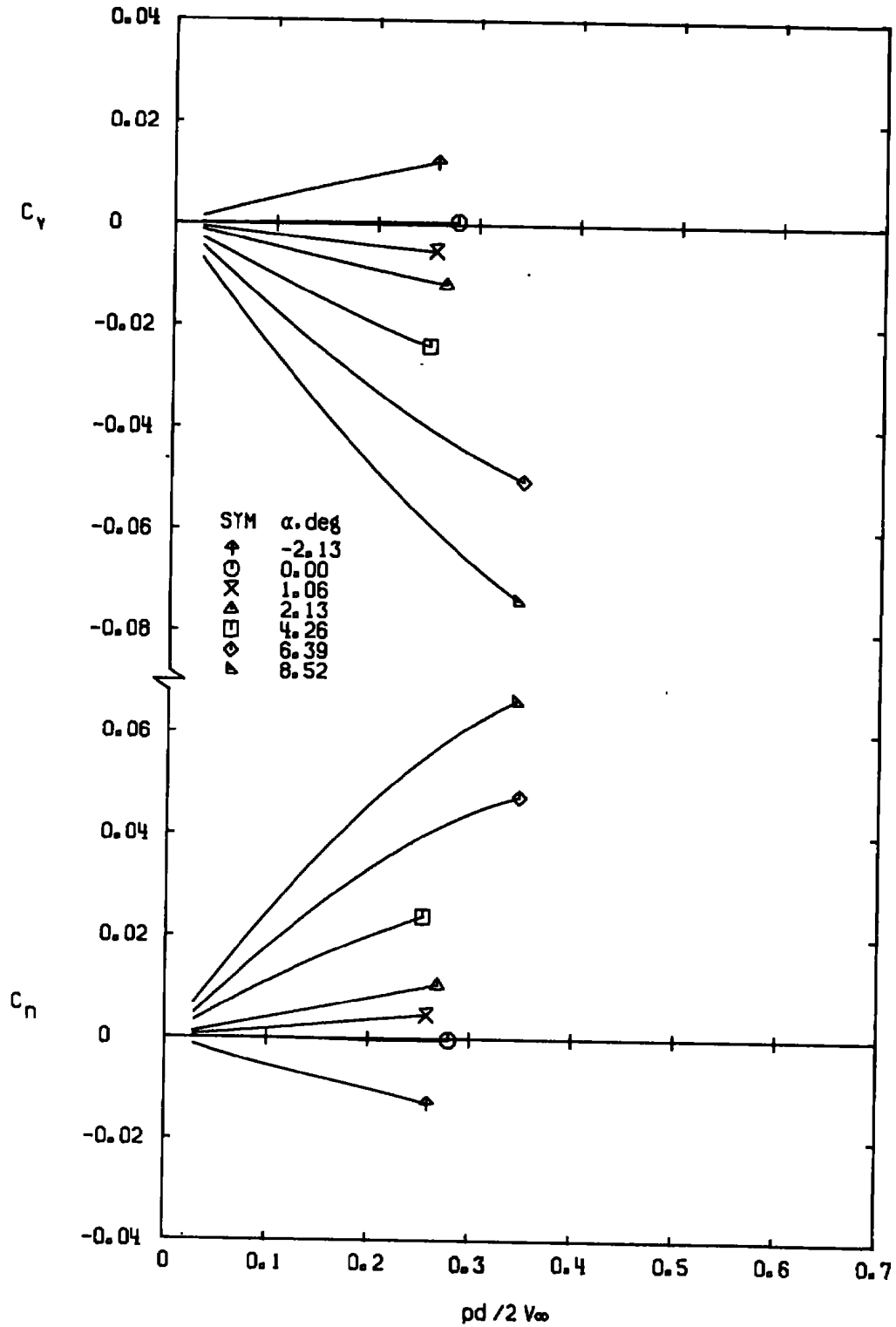
e. M_\infty = 1.00 Figure 11. Continued.
