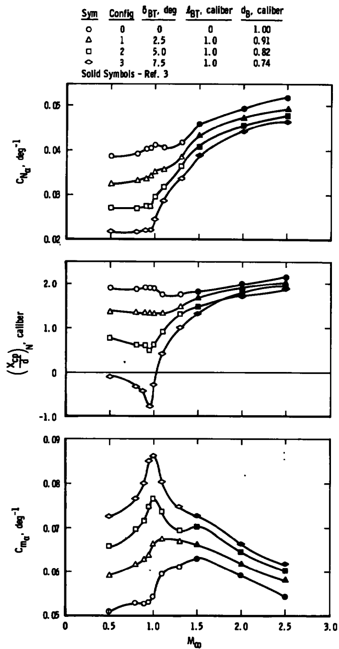
a. Effect of boattail angle with a constant boattail length Figure 6. Variation of C_{N_a} , C_{m_a} , and (X_{cp}/d)_N with Mach number, Re_x = 9.6 \times 10^6 .
