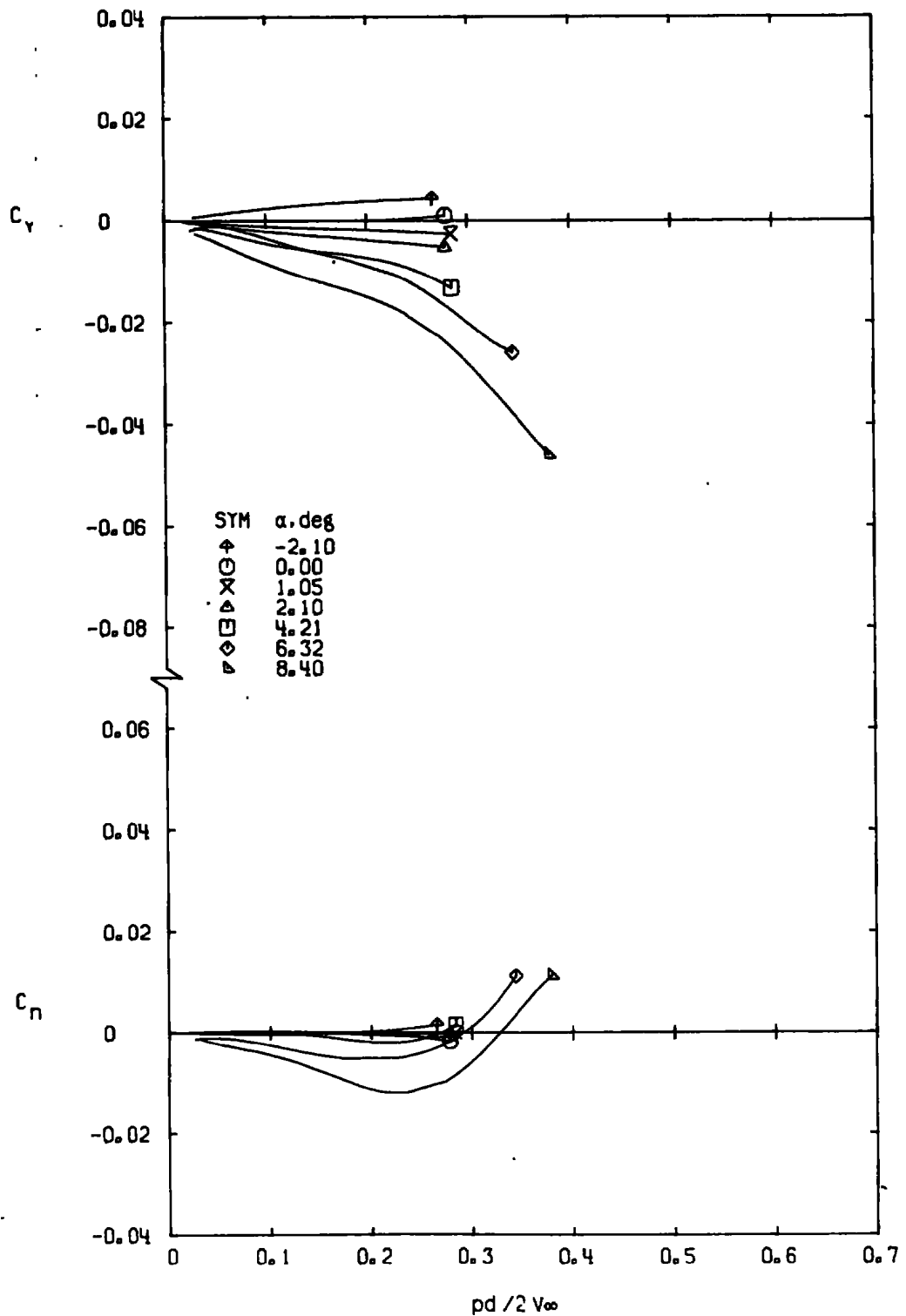
d. M_\infty = 0.95 Figure 15. Continued.
