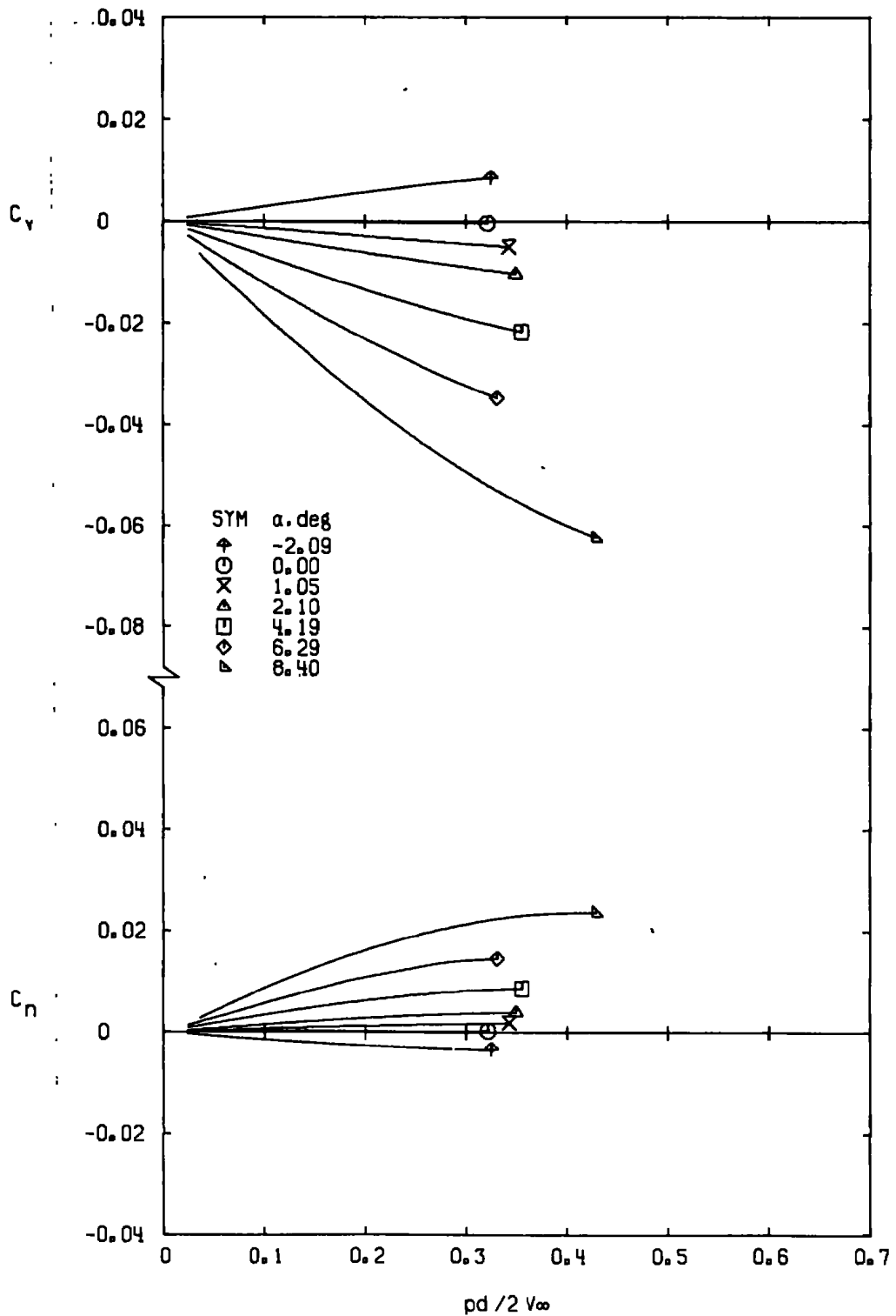
b. M_\infty = 0.80 Figure 13. Continued.
