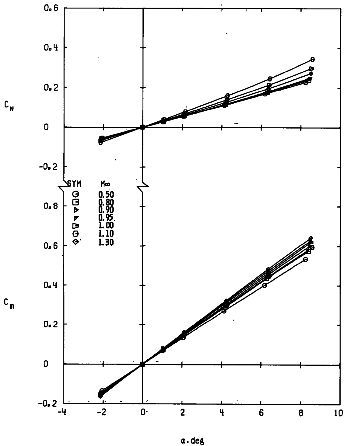
c. Configuration 2 Figure 5. Continued.
