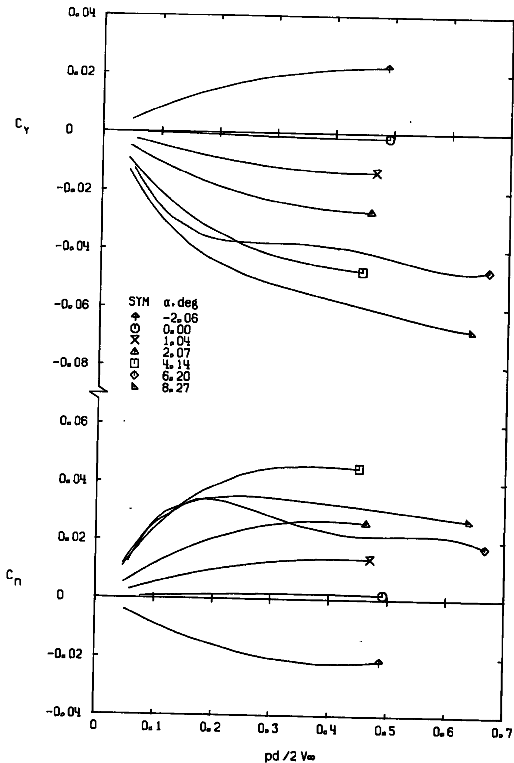
Figure 15. Variation of C_Y and C_n with pd/2V_\infty for Configuration 7.
