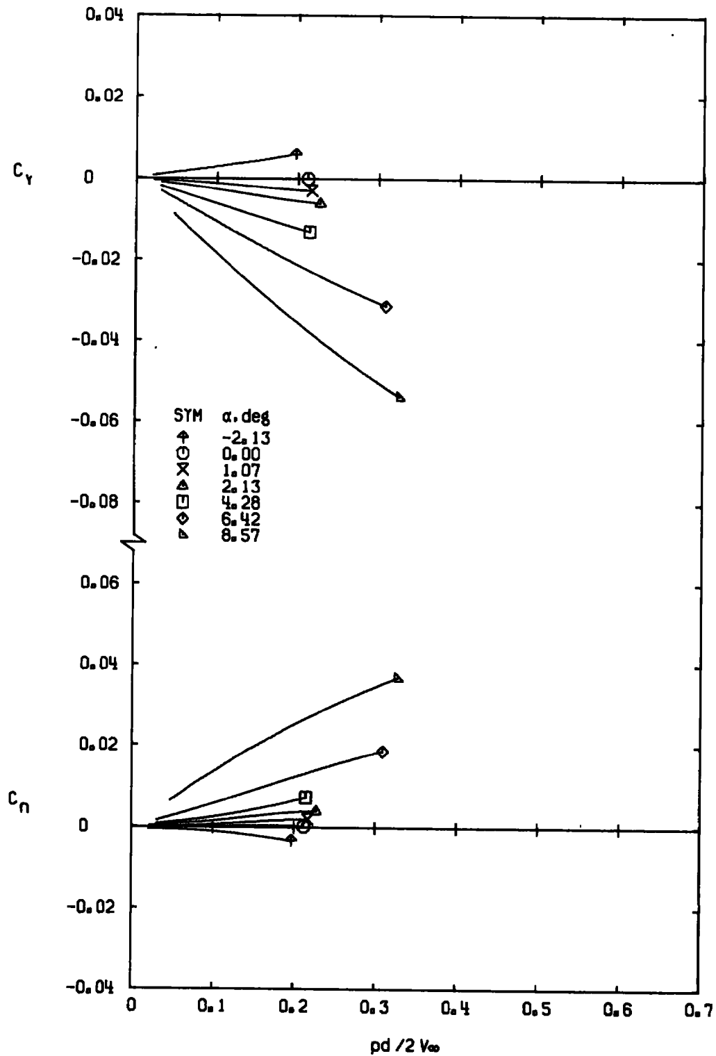
g. M_\infty = 1.30 Figure 9. Concluded.
