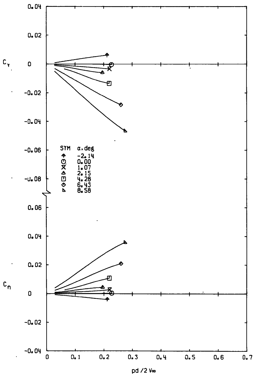
g. M_\infty = 1.30 Figure 10. Concluded.
