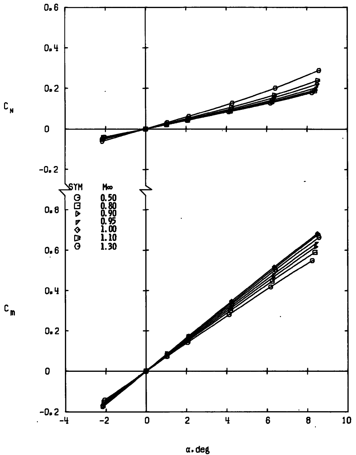
g. Configuration 6 Figure 5. Continued.
