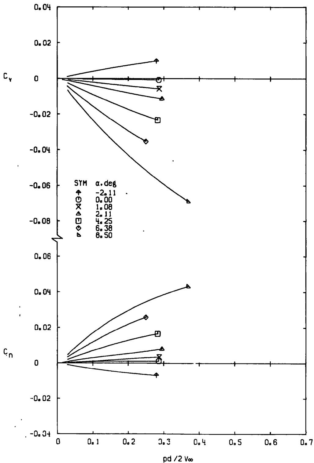
d. M_\infty = 0.95 Figure 11. Continued.
