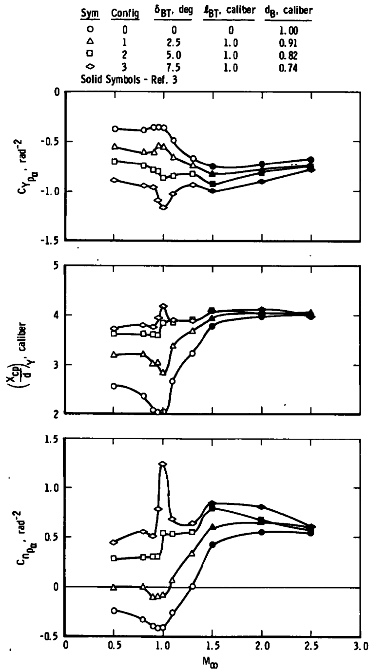
a. Effect of boattail angle with a constant boattail length Figure 19. Variation of C_{Y p_a} , C_{m p_a} , and (X_{cp}/d)_Y with Mach number, Re_\ell = 9.6 \times 10^6 .
