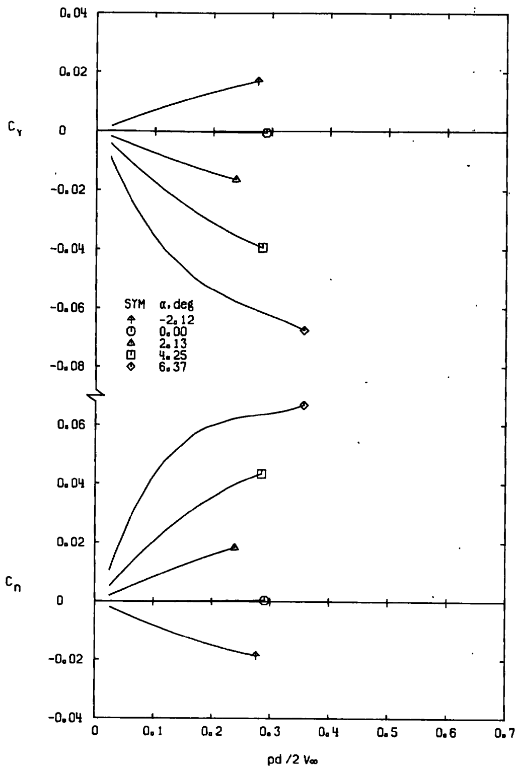
d. M_\infty = 0.95 Figure 16. Continued.
