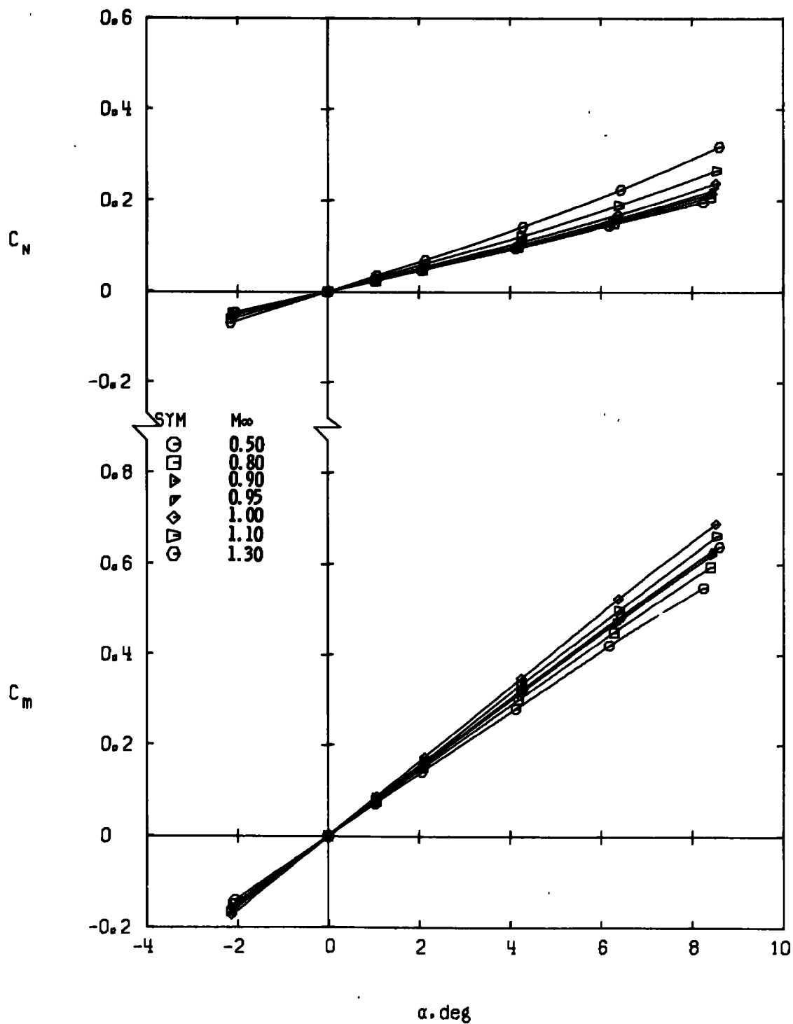
f. Configuration 5 Figure 5. Continued.
