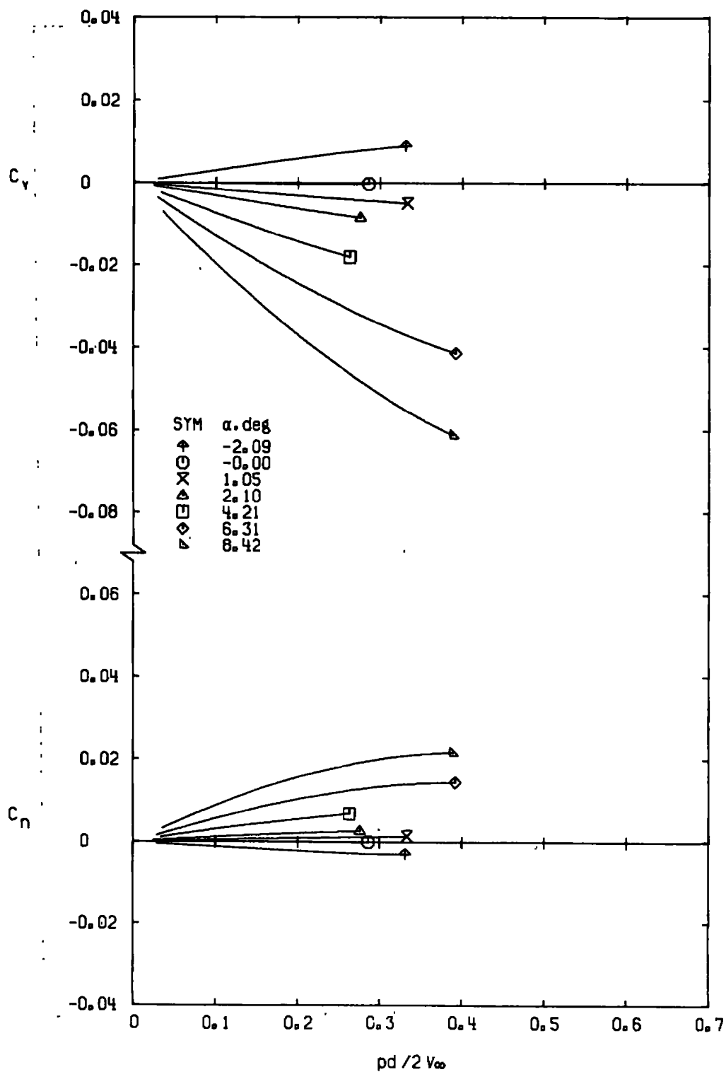
c. M_\infty = 0.90 Figure 14. Continued.
