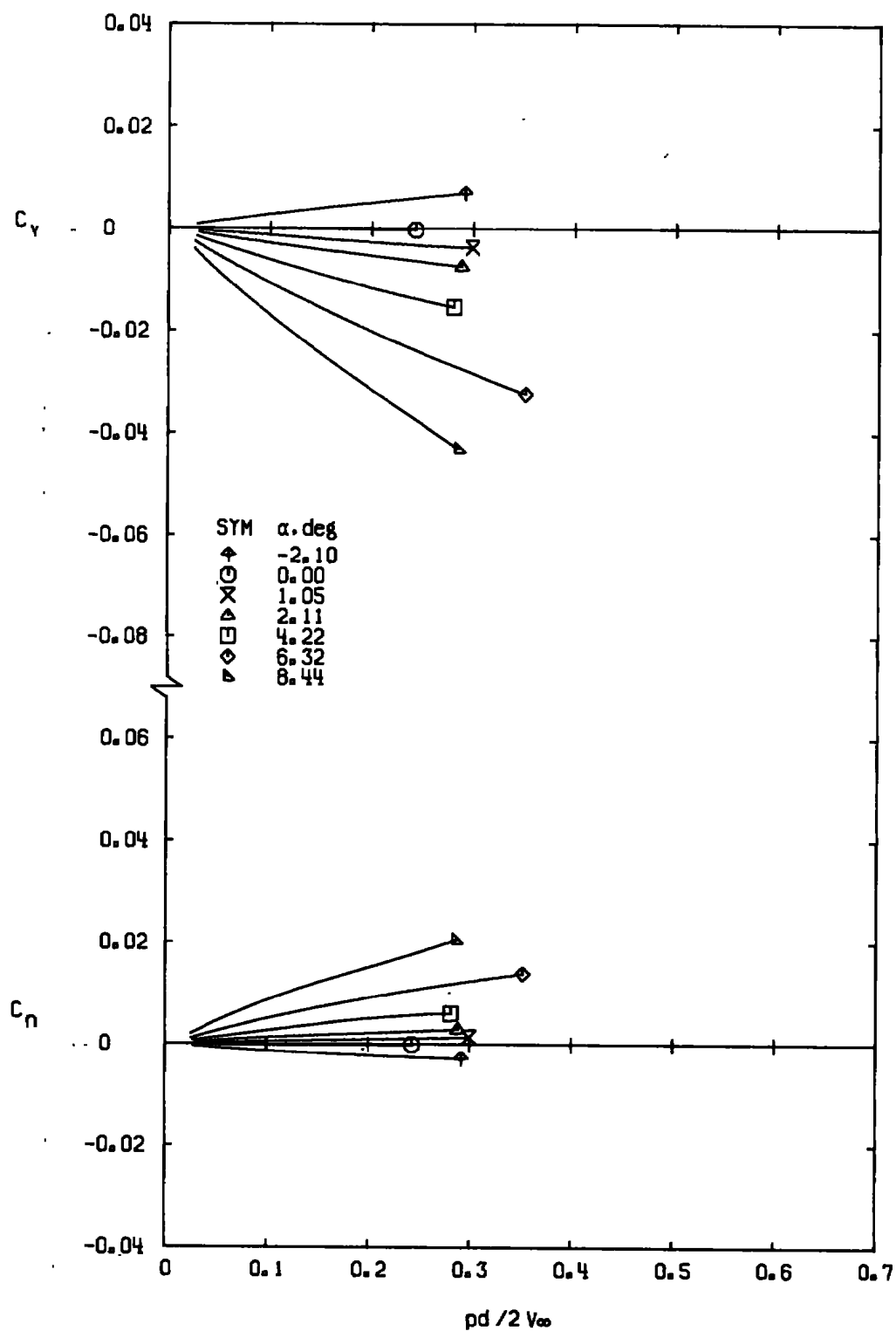
c. M_\infty = 0.90 Figure 12. Continued.
