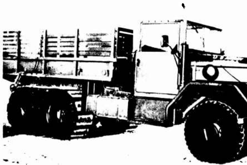
Figure 1. Tyr-Trac mounted on the M35-A2, 6x6 2½-ton truck.
