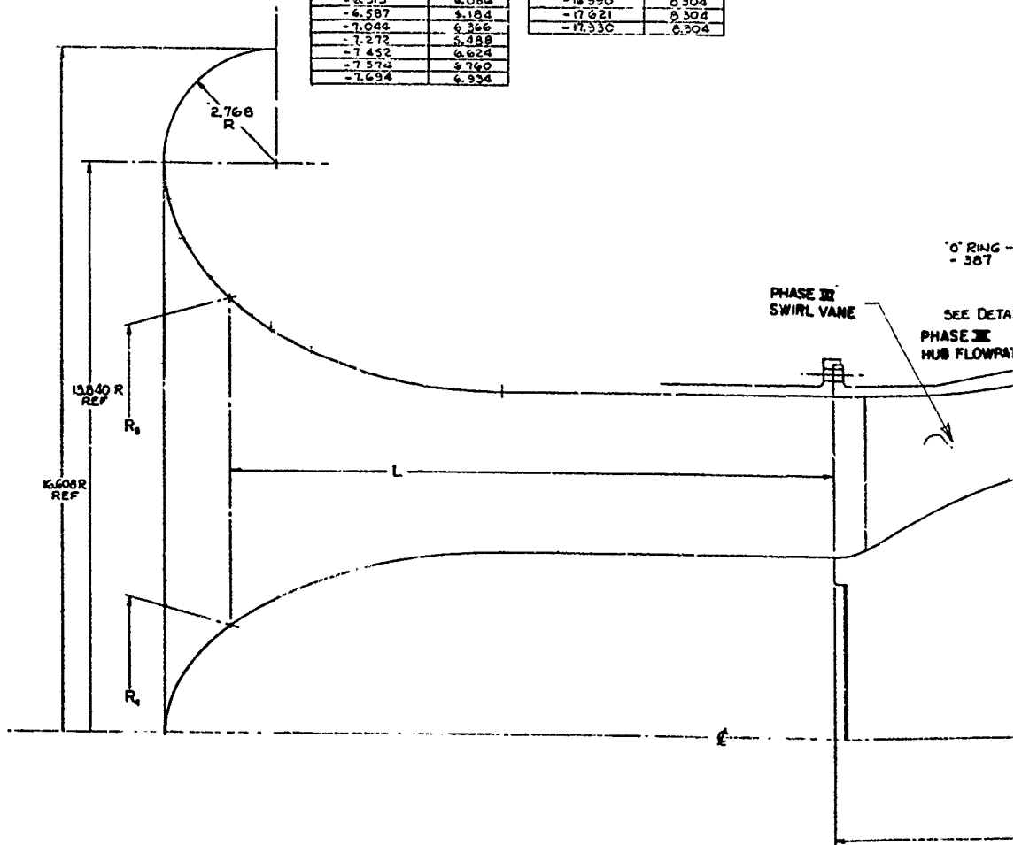
Figure 24. 15 Lb/Sec Separator Model.
