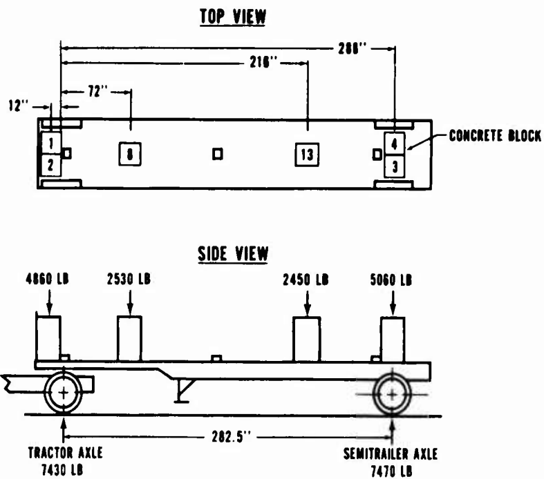
Figure 46. Static Test, Three-Fifths Load, Truck Type III.
