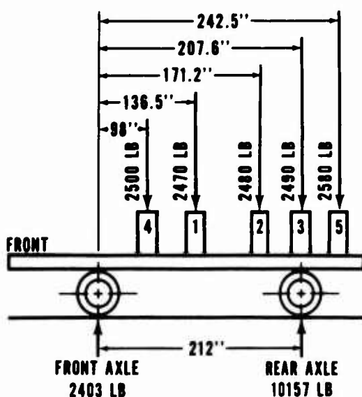
Figure 35. Static Test, Full Load, Center of Gravity, Truck Type I.
