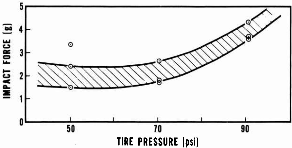
Figure 26. Impact Forces Versus Tire Pressure on Tractor Axle of Truck Type II at Full- and One-Half Axle Loads.
