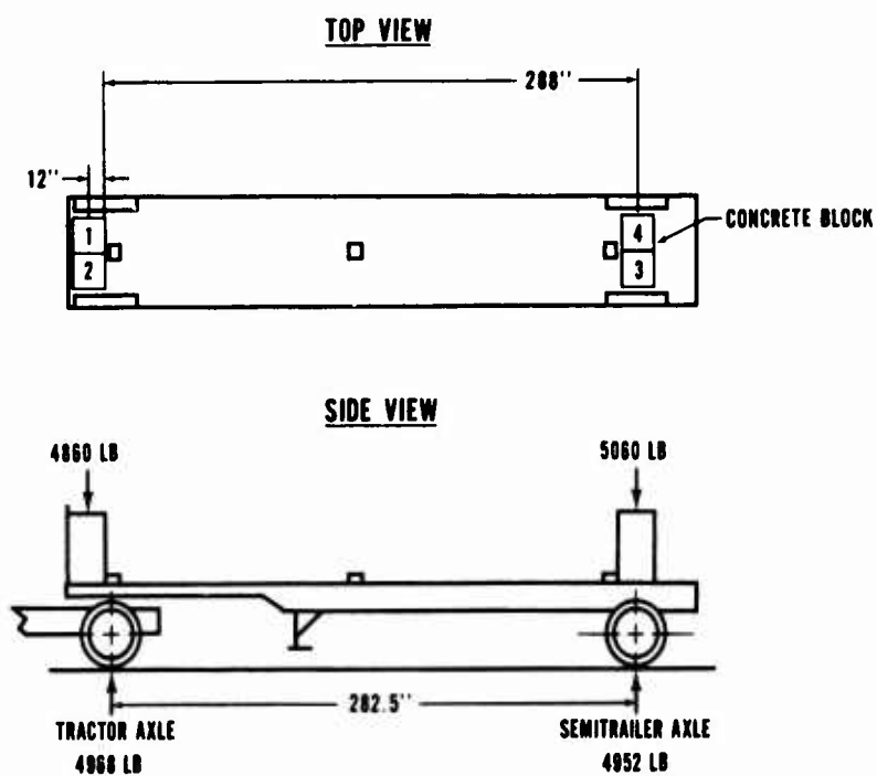
Figure 47. Static Test, Two-Fifths Load, Truck Type III.
