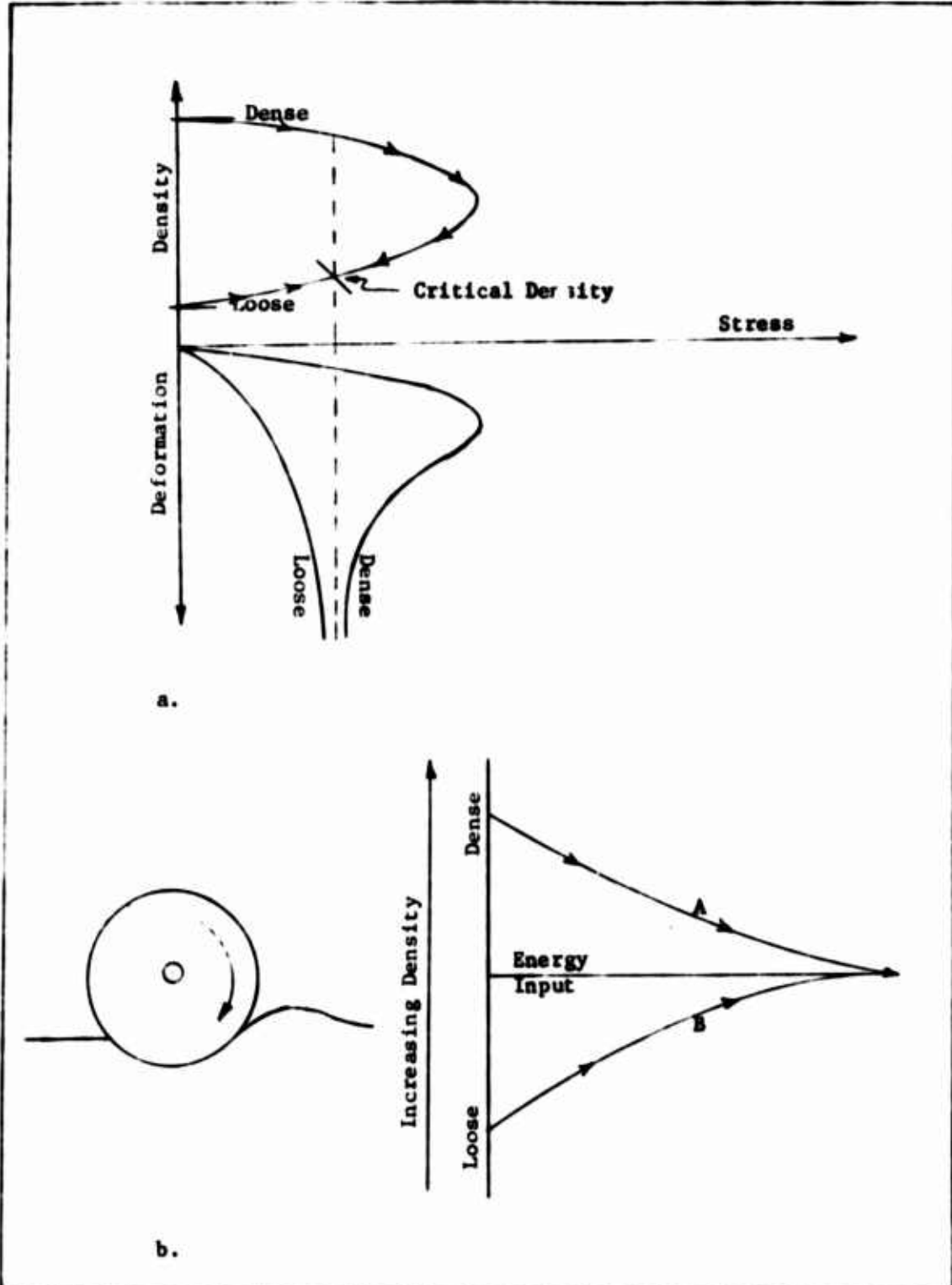
Figure 20. Critical Density
