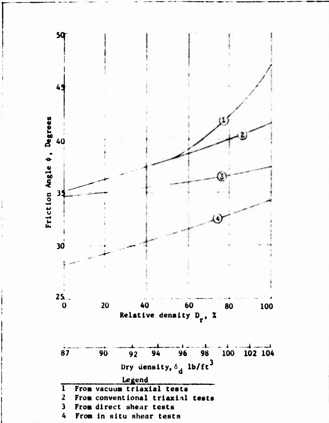
Figure 22. Friction angles of Yuma sand from various test methods as function of density (data from reference 24)
