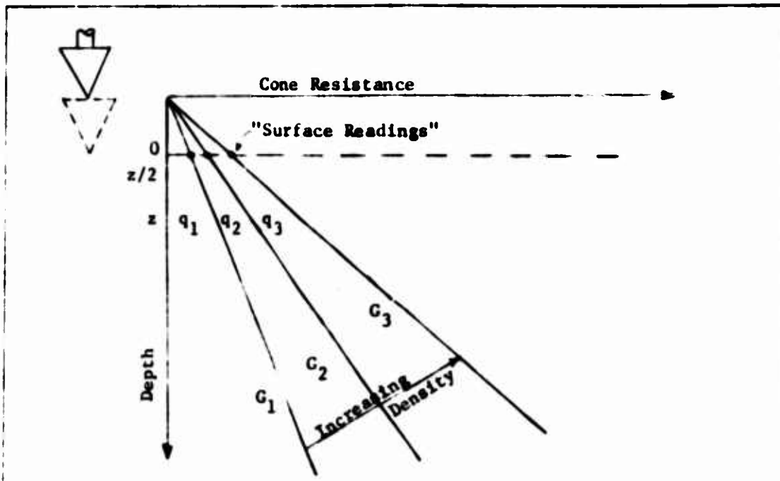
a. Influence of sand density on cone penetration resistance
