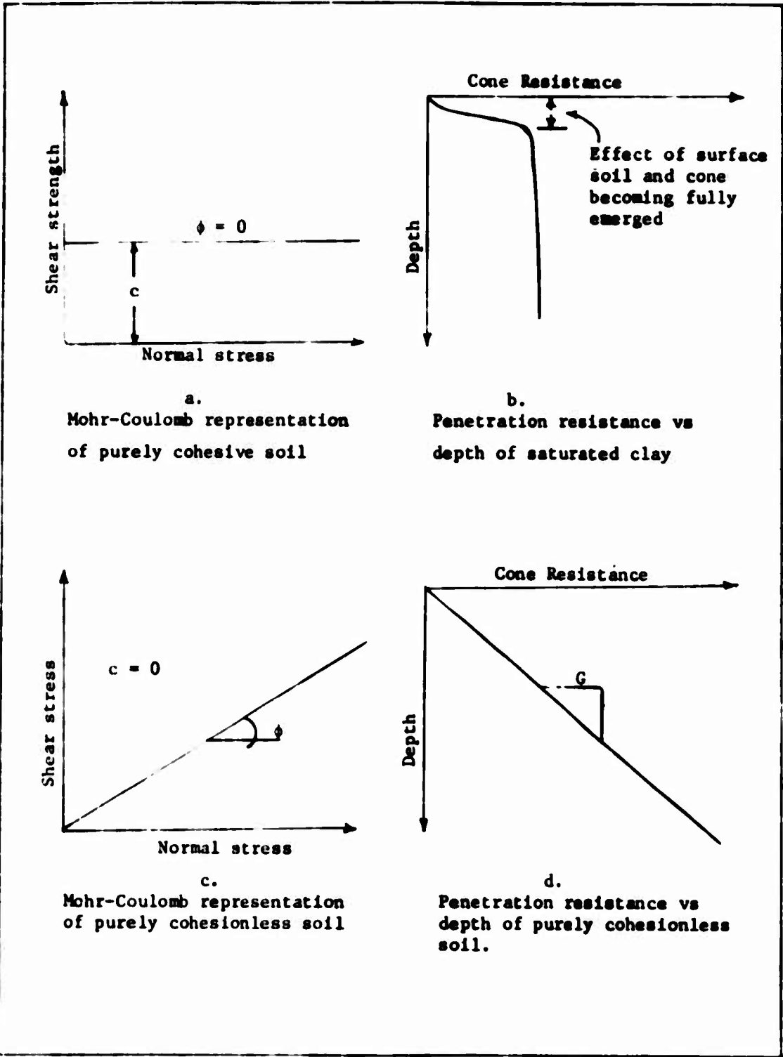
Figure 23. Cone penetration of soils
