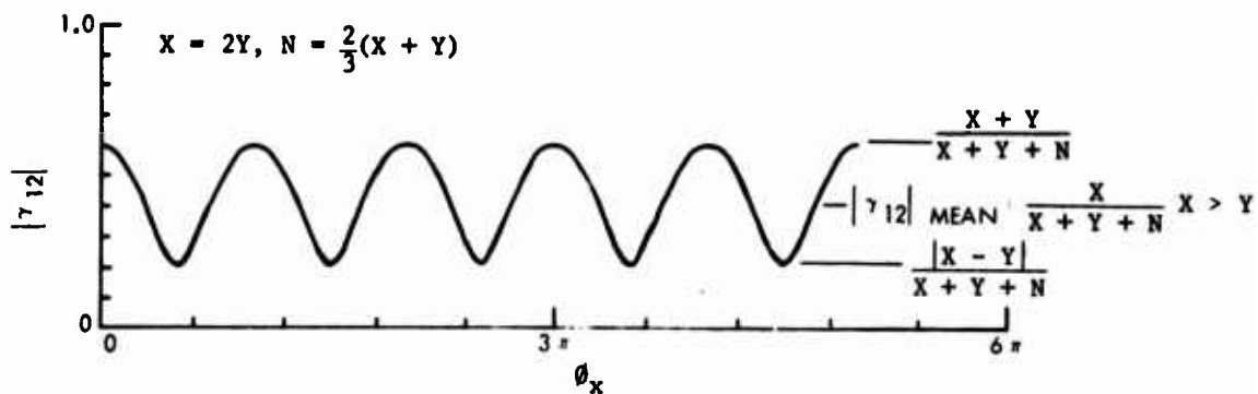
Figure 12. |\gamma_{12}| for Two Waves With \phi_y = -\phi_x ; Maxima, Minima, and Mean
