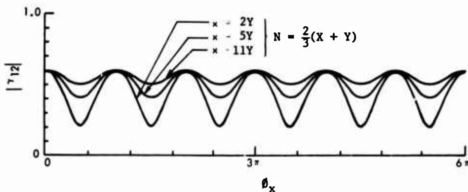
Figure 13. |\gamma_{12}| for Two Waves With \phi_y = -\phi_x ; Effect of Relative Wave Magnitudes
