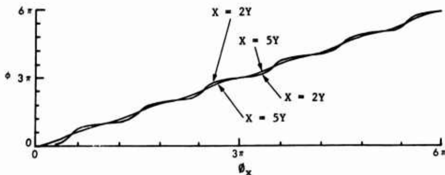
Figure 14. \phi for Two Waves With \phi_y = -\phi_x ; Effect of Relative Wave Magnitudes
