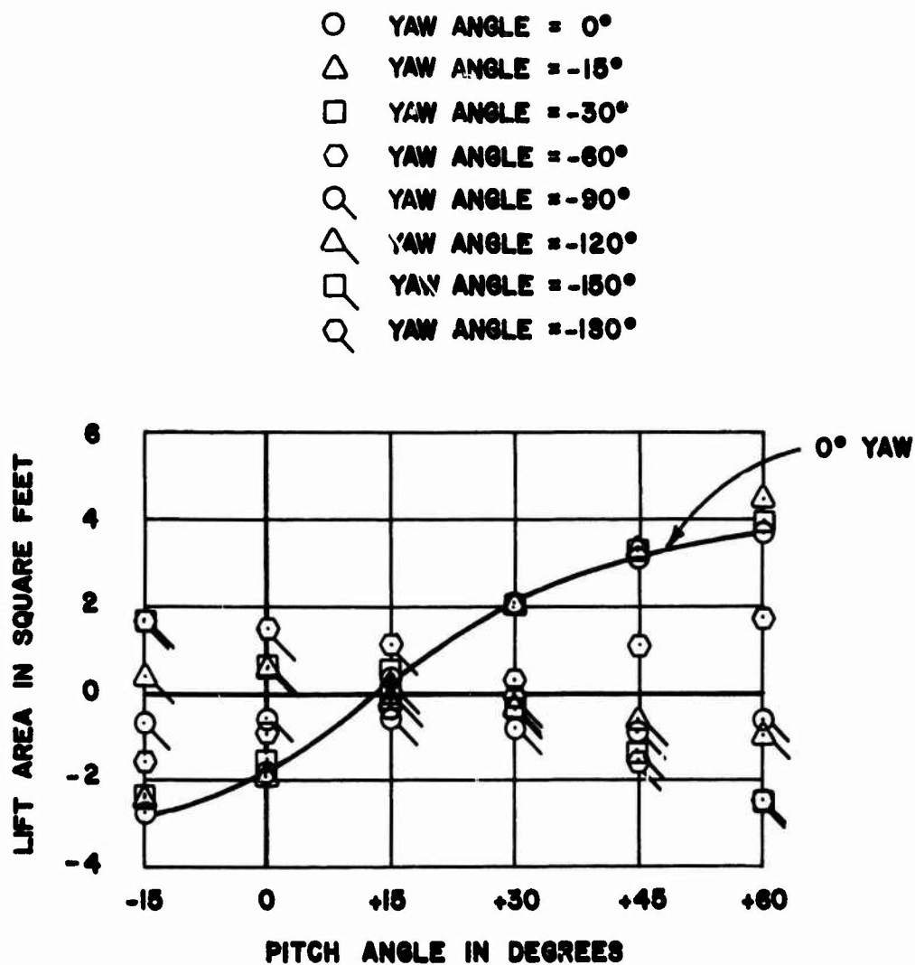
FIGURE 25 ACES II SEAT LIFT FORCE AREA AS A FUNCTION OF PITCH ANGLE FOR VARIOUS YAW ANGLES.
