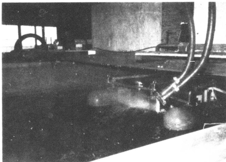
FIGURE 3.15: PHOTOGRAPH OF THE REAR OF THE CONTROL/RECOVERY DEVICE IN OPERATION
