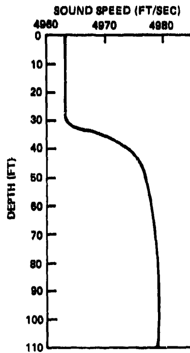
FIG. 6 CHESAPEAKE BAY SOUND SPEED PROFILE
