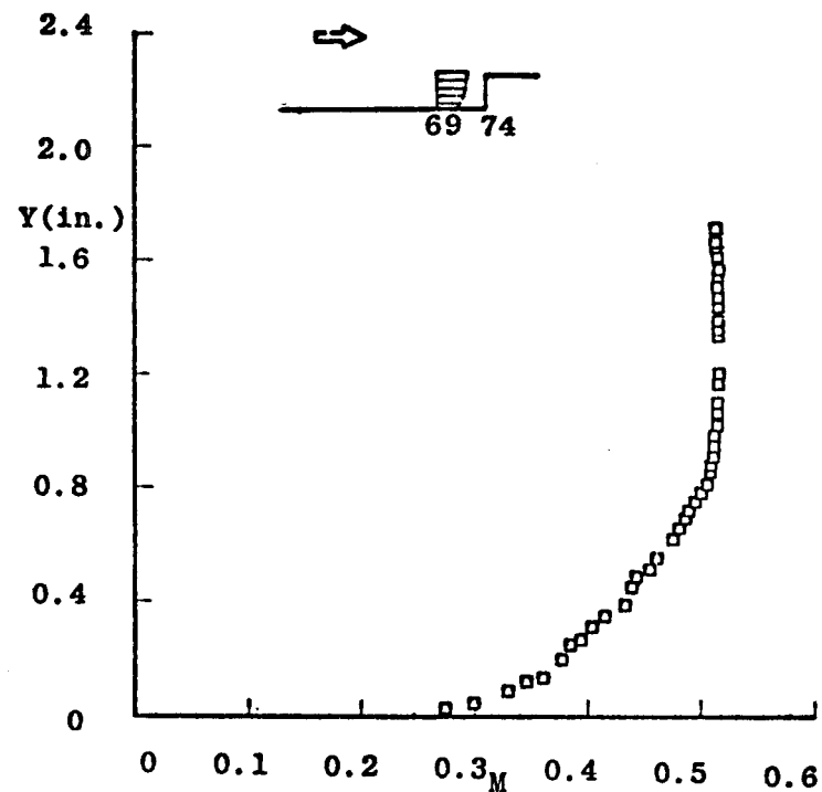
d. 69-inch Station, M_e = 0.52 , Re_L = 32.5 \times 10^6
