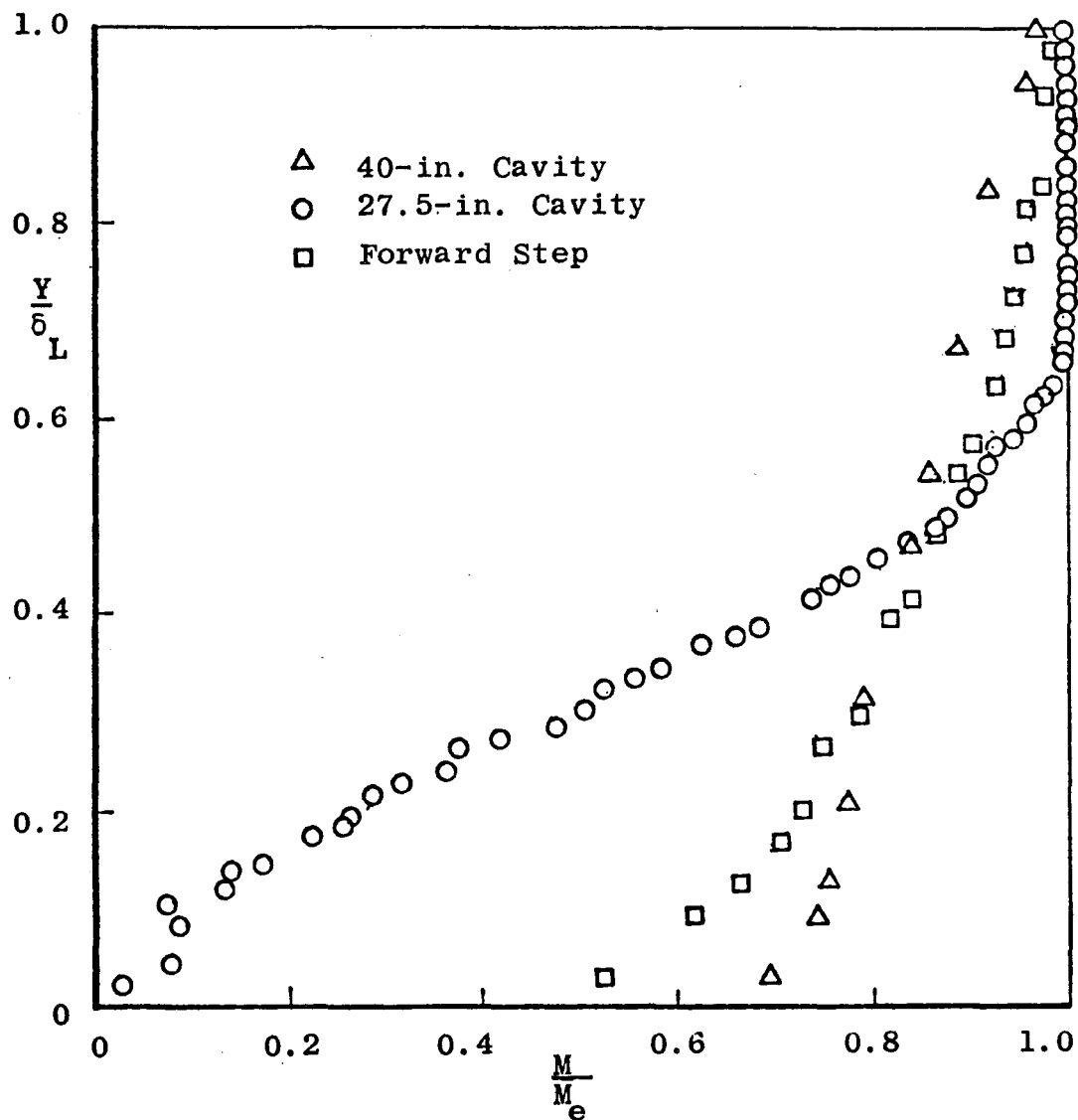
Figure 22. Effect of model configuration on the velocity profile
