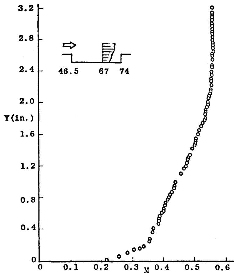
c. 67-inch Station, M_e = 0.56 , Re_L = 32.5 \times 10^6
