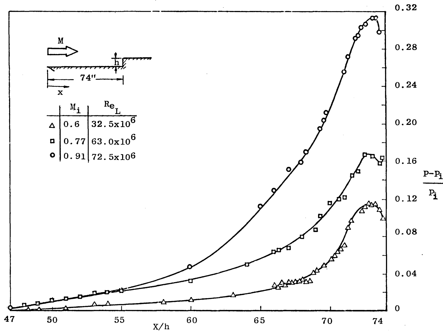
Figure 26. Mach number effect on the wall pressure distribution
