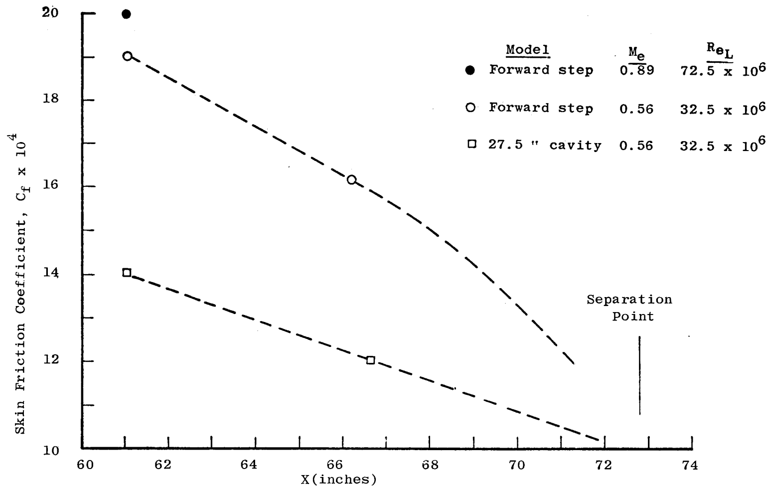
Figure 30. Mach number, model configuration and station effects on skin friction
