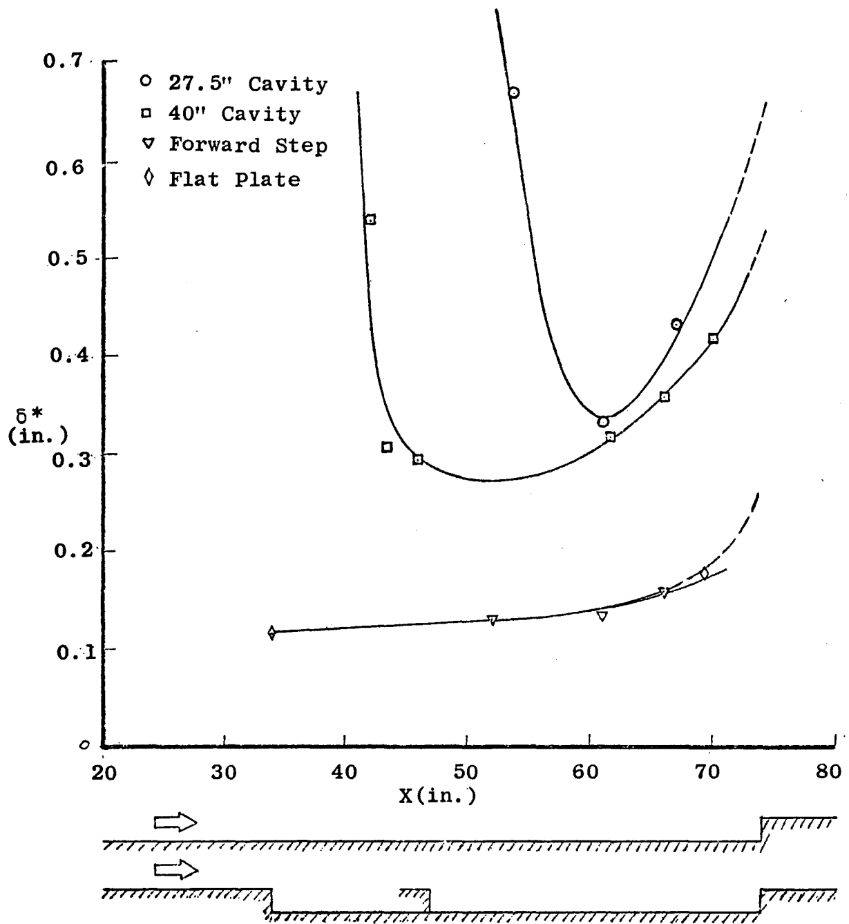
Figure 31. Development of shear layer displacement thickness along the models
