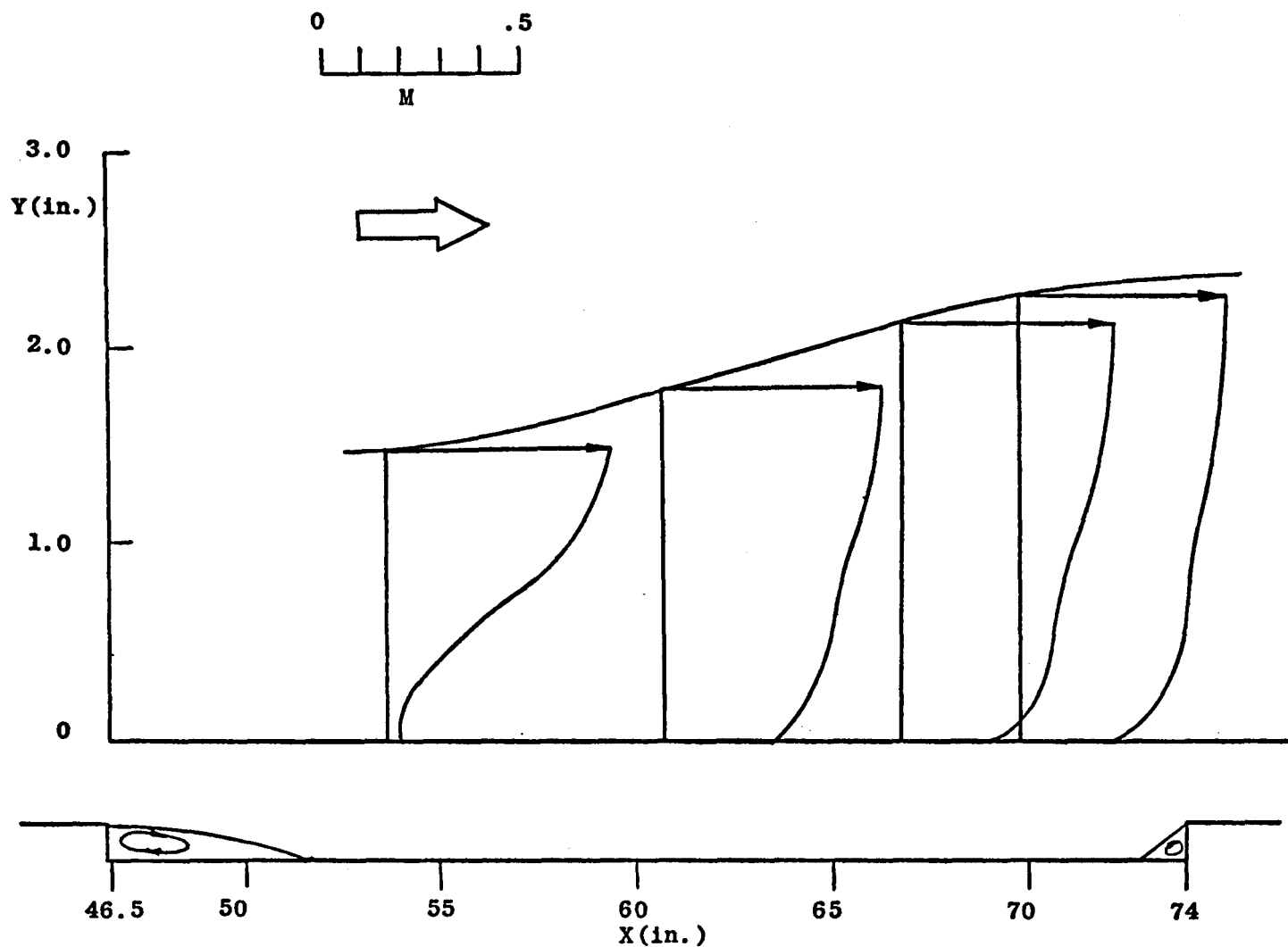
Figure 20. Flow variation along the 27.5 inch long cavity model. M_e = 0.6 , Re_L = 32.5 \times 10^6
