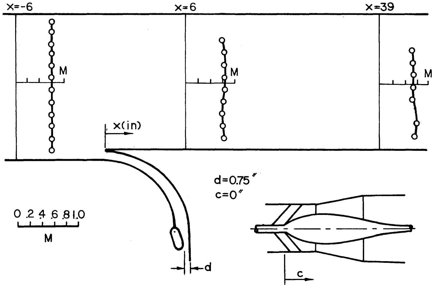
Figure A-4. Vertical Mach number distribution across the test-section.
