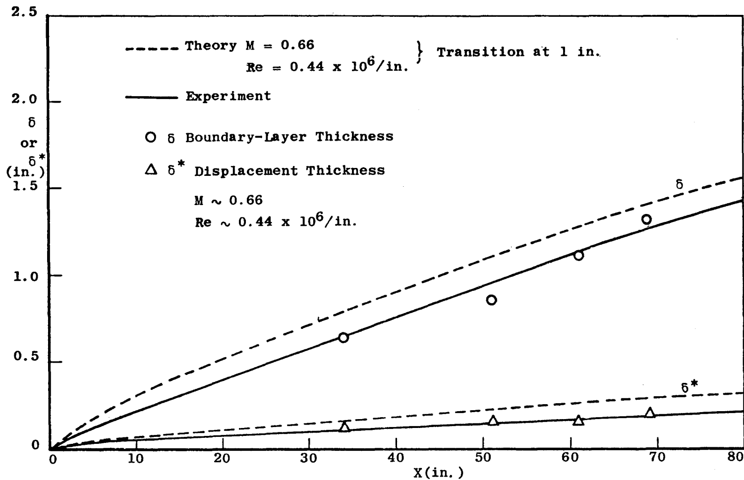
Figure 36. Comparisons of experimental data and theoretical computations for boundary layer thickness and displacement thickness
