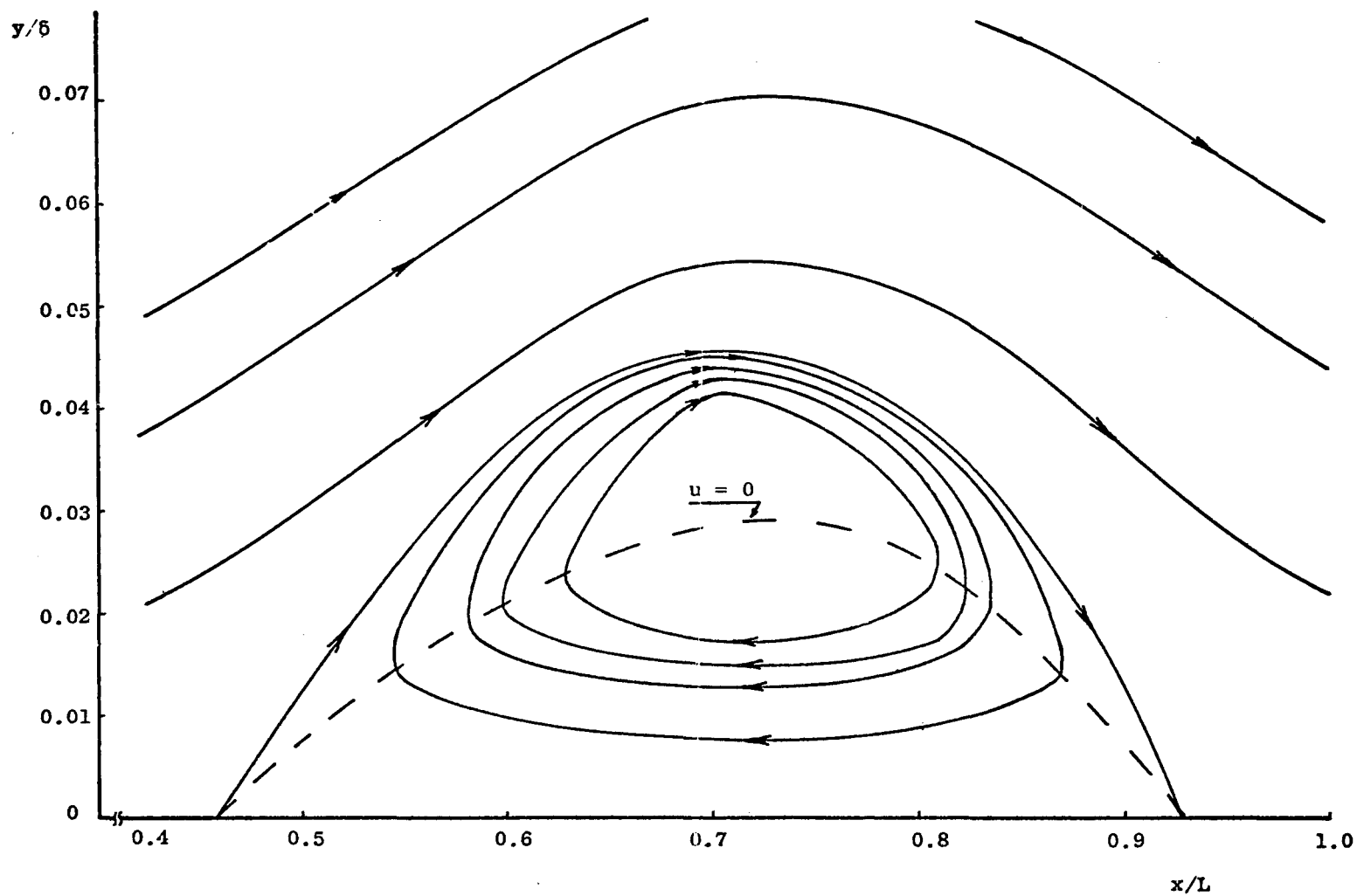
Figure 37. Streamline pattern for a flow with separation linearized equation model
