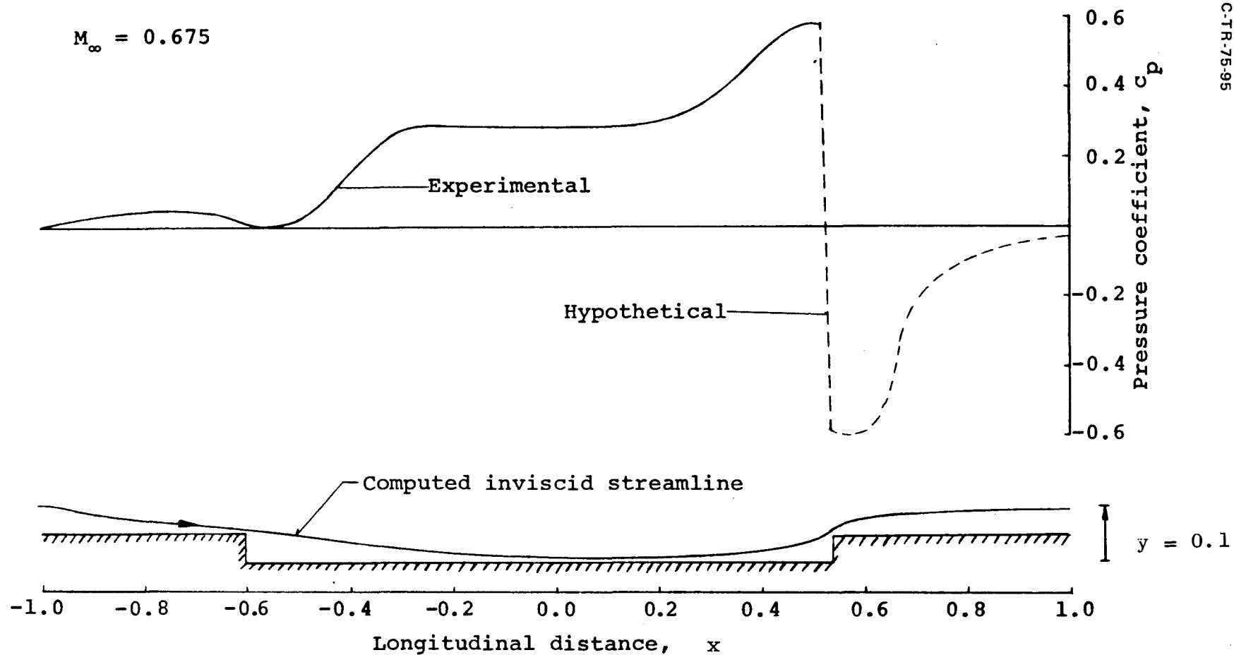
Figure 32. Computer inviscid streamline corresponding to an extended experimental pressure coefficient distribution
