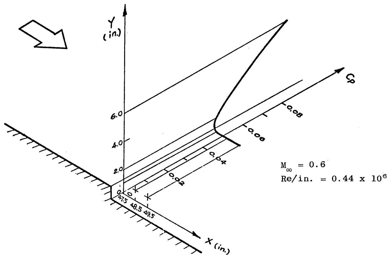
Figure 21b. Static pressure distribution on the side wall near the rearward facing step region.
