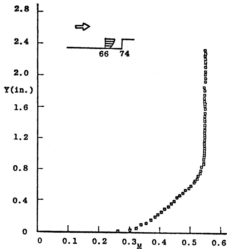
c. 66-inch Station, M_e = 0.55 , Re_L = 32.5 \times 10^6
