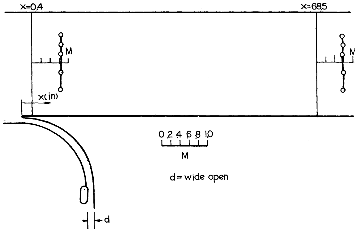
Figure A-5. Vertical Mach number distribution across the test-section for a long range.
