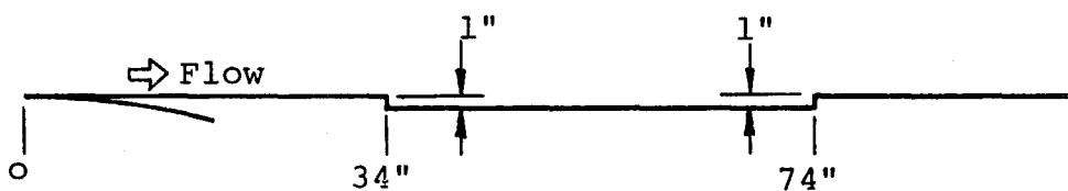
(c) 40-inch long shallow-cavity model
