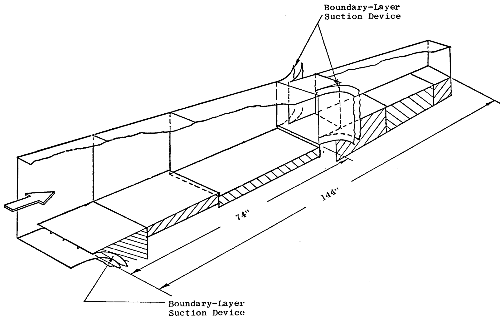
a. Pictorial View of Model Installation
