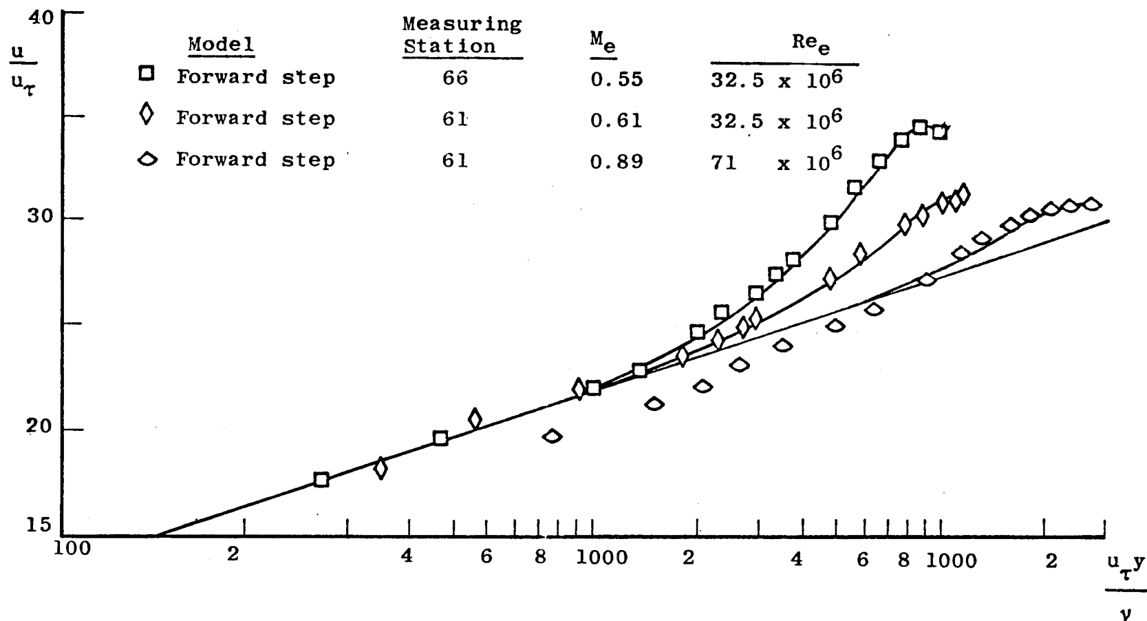
Figure 29. Velocity profile by law of wall and law of wake
