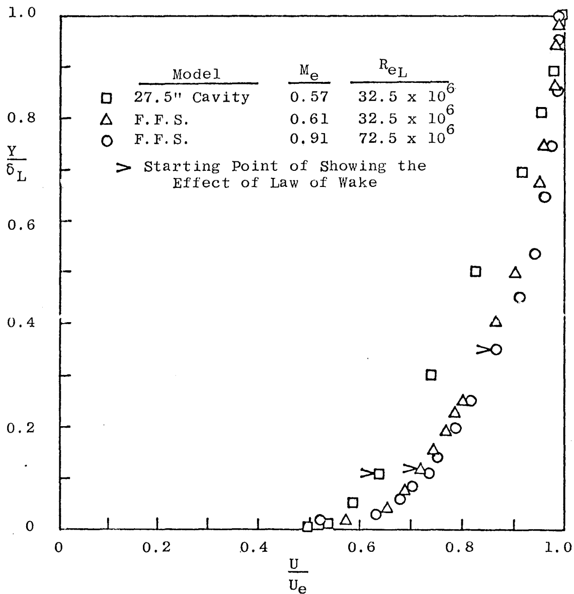
a. Station 61-in. on the Forward-Facing Step and 27.5-in. Cavity Models.
