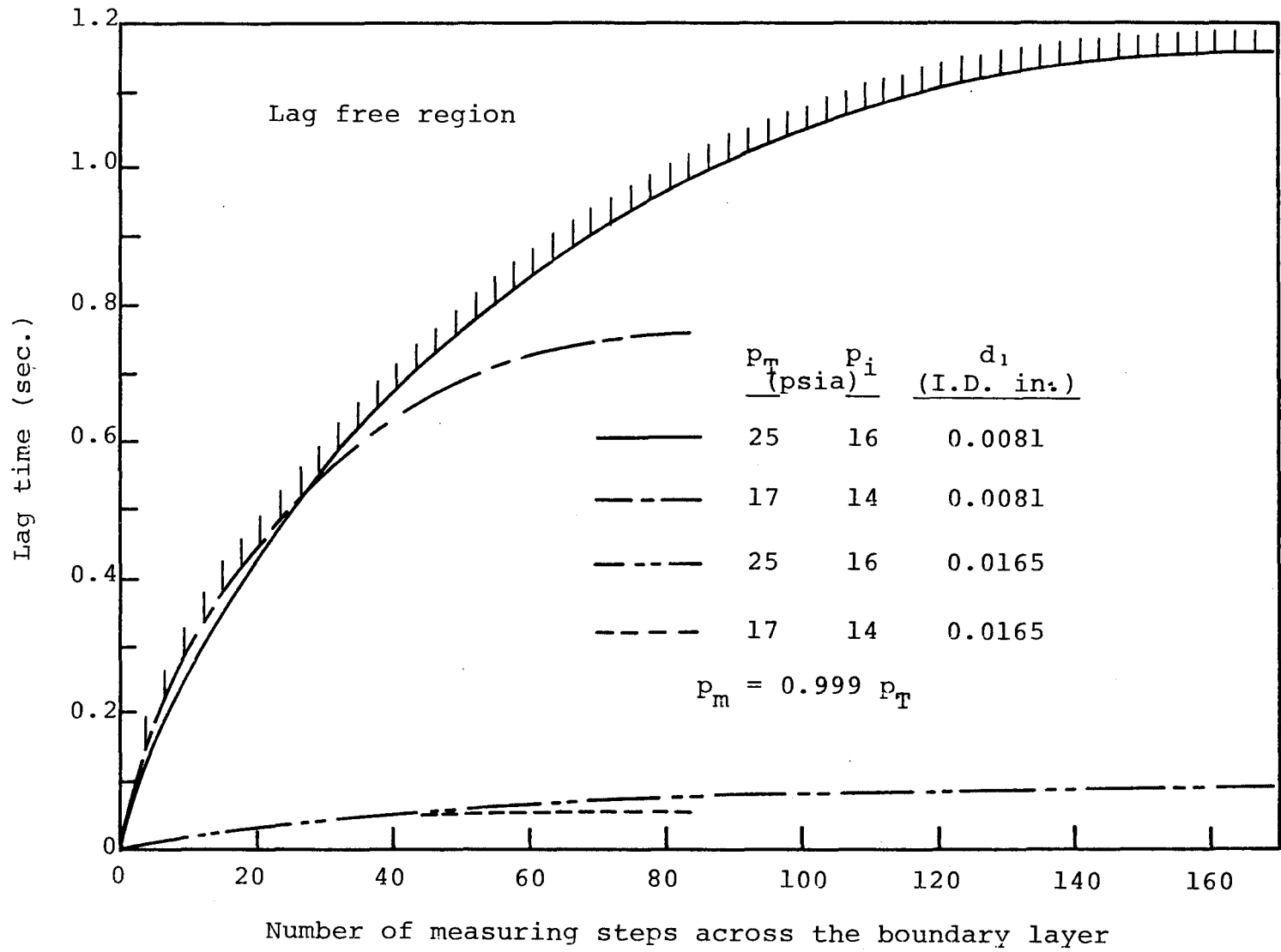
Figure 11. Theoretical values of pitot-probe lag time.
