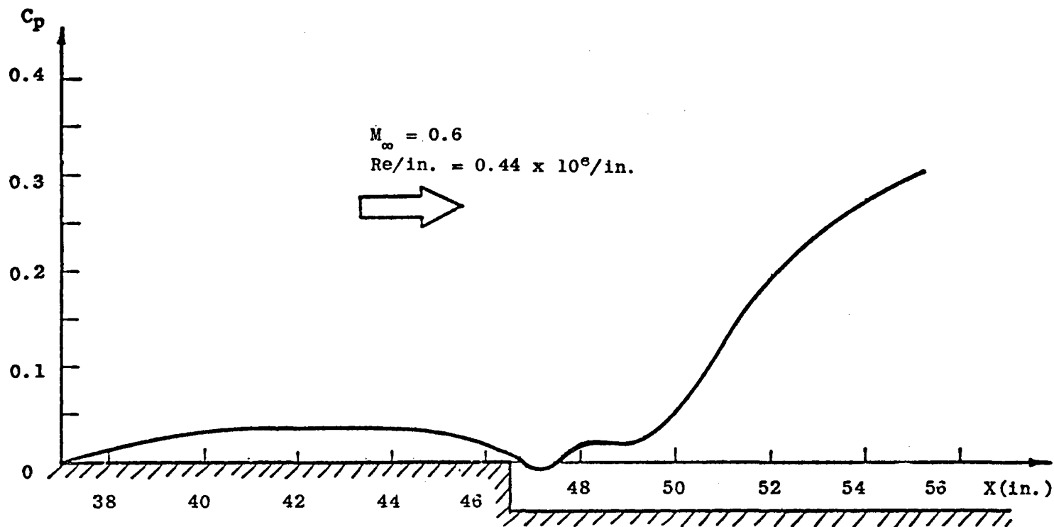
Figure 21a. Static pressure distribution on the model surface near the rearward facing step region.
