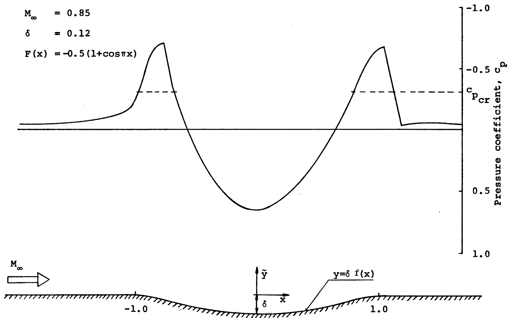
Figure 33. Computed pressure coefficient distribution for a flow over an assumed cavity.
