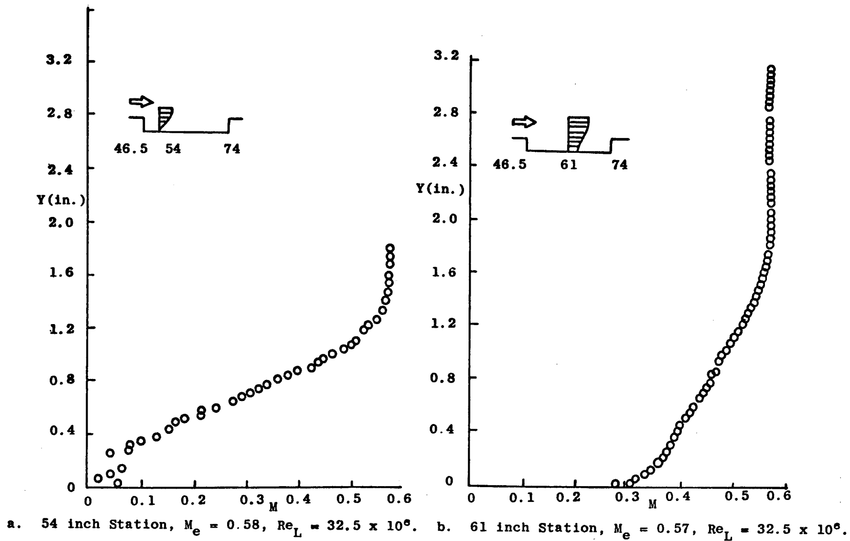
Figure 16. Velocity profiles on 27.5 inch long cavity like model
