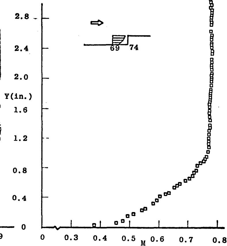
f. 69-inch Station, M_e = 0.79 , Re_L = 72.5 \times 10^6
