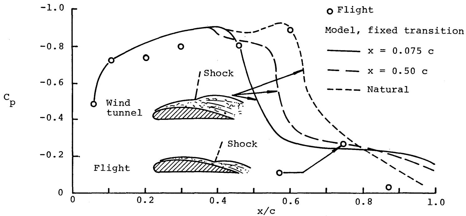
Figure 4. Surface pressure distribution showing strong influence of Reynolds number
