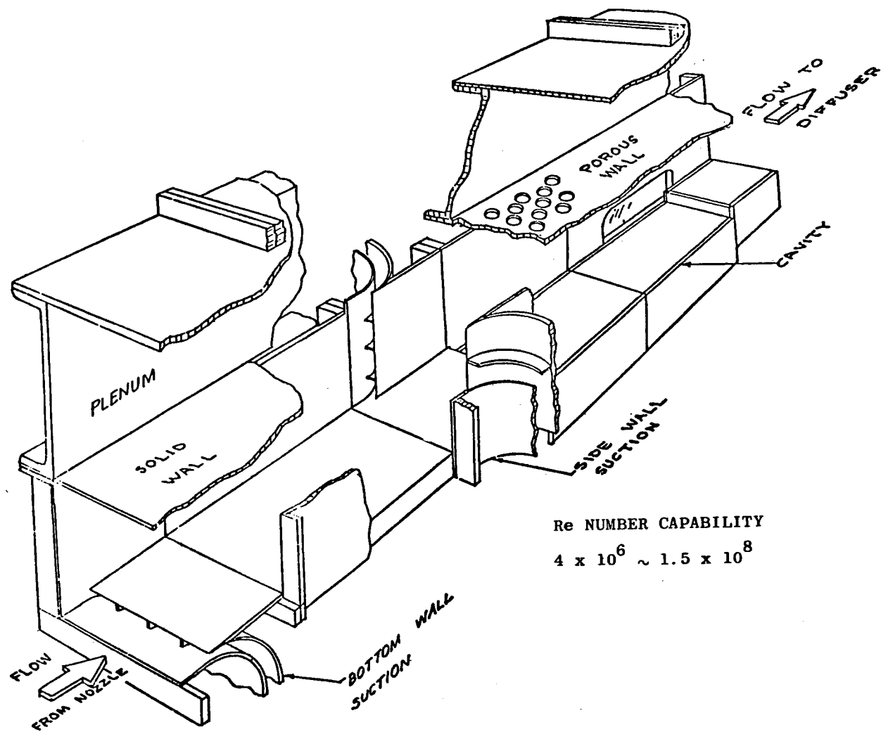
Figure 6. Pictorial view of test section.
