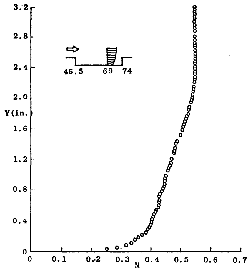
d. 69-inch Station, M_e = 0.55 , Re_L = 32.5 \times 10^6
