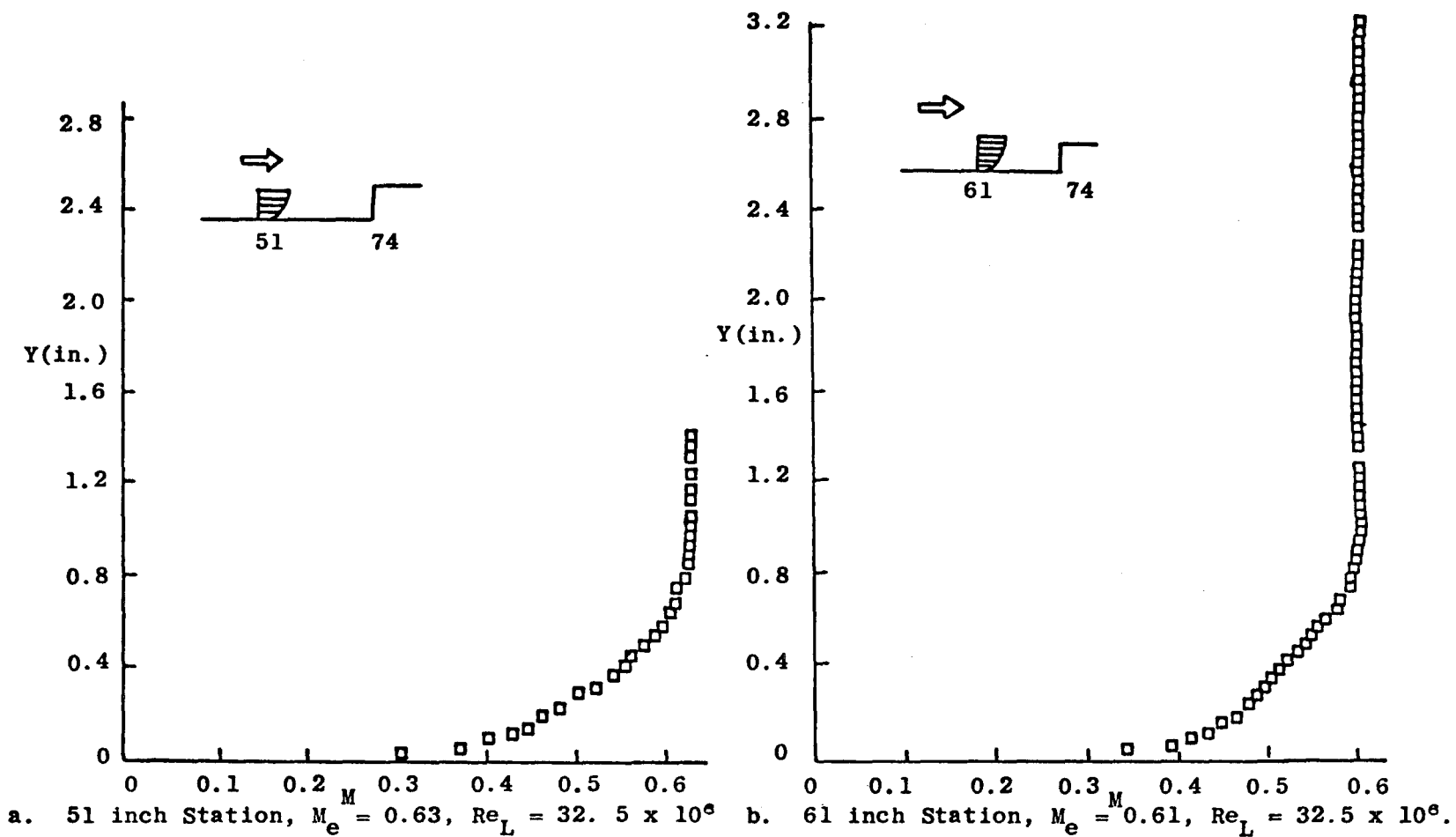
Figure 14. Velocity profiles on forward facing step model
