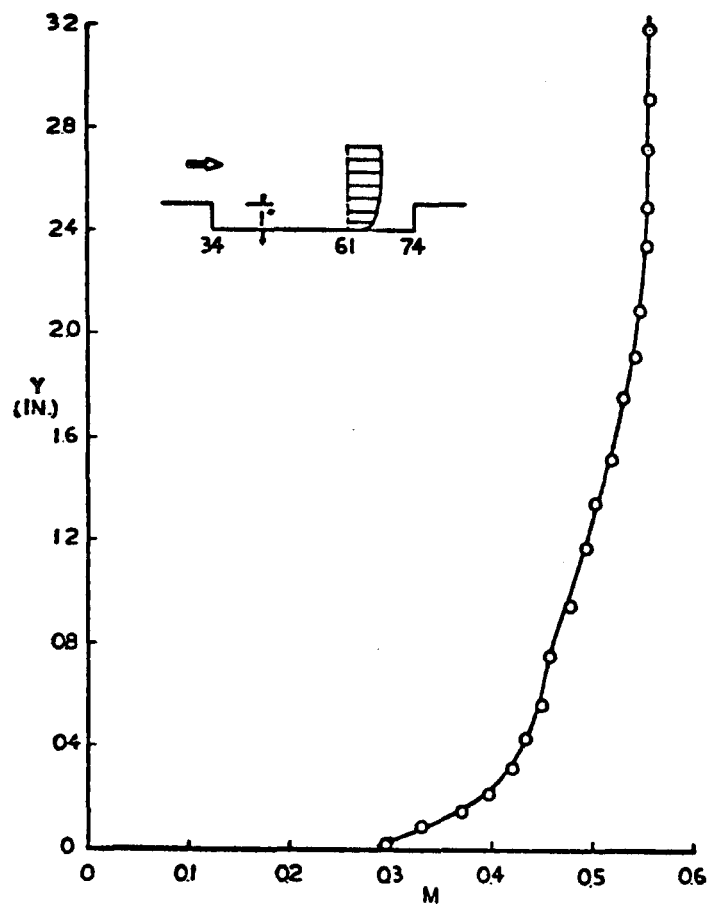
e. 61-inch Station, M_e = 0.56 , Re_\gamma = 32.5 \times 10^6
