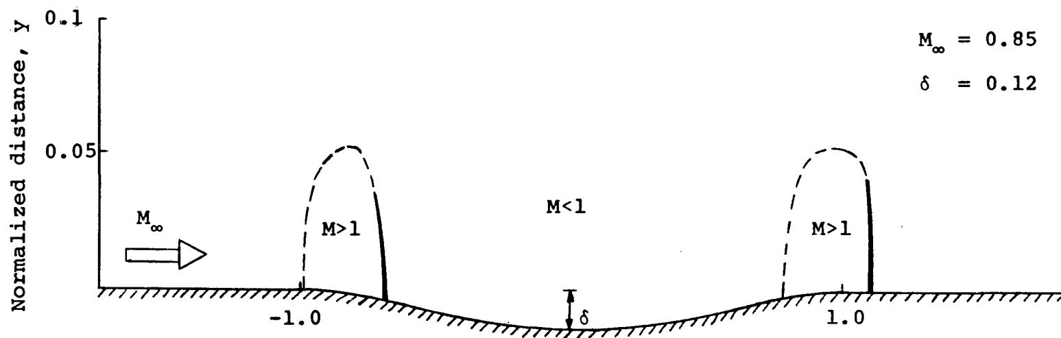
Figure 34. Extension of supersonic pockets for a cavity flow.
