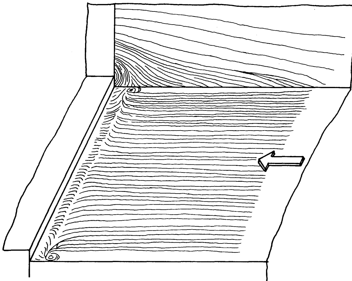
Figure 27 Three-dimensional sketch of oil flow pattern on the forward-facing step model and the side wall.
