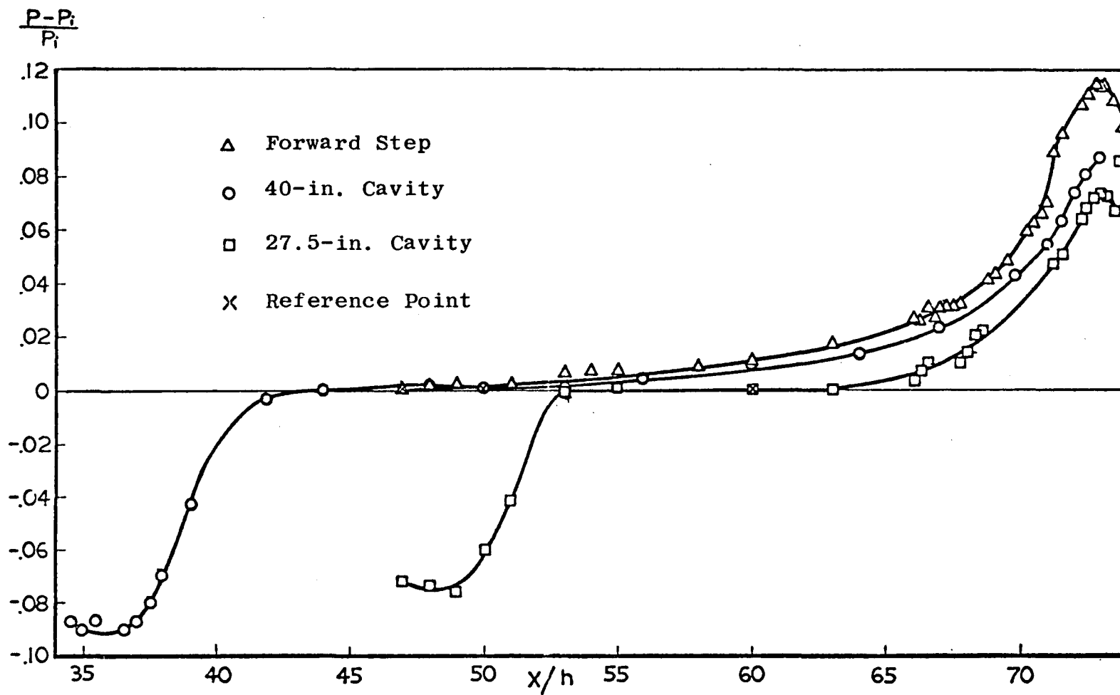
Figure 25. Comparison of wall static pressure distribution on different models
