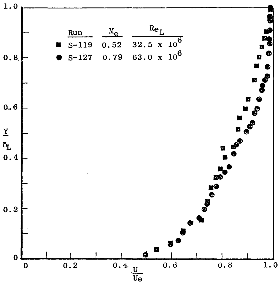
b. Station 69 in. on the Forward-Facing Step Model
