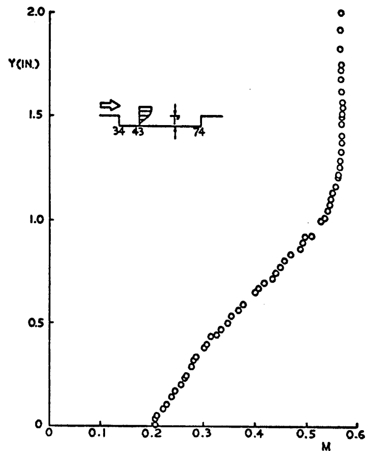
b. 43-inch Station, M_e = 0.55 , Re_L = 32.5 \times 10^6
