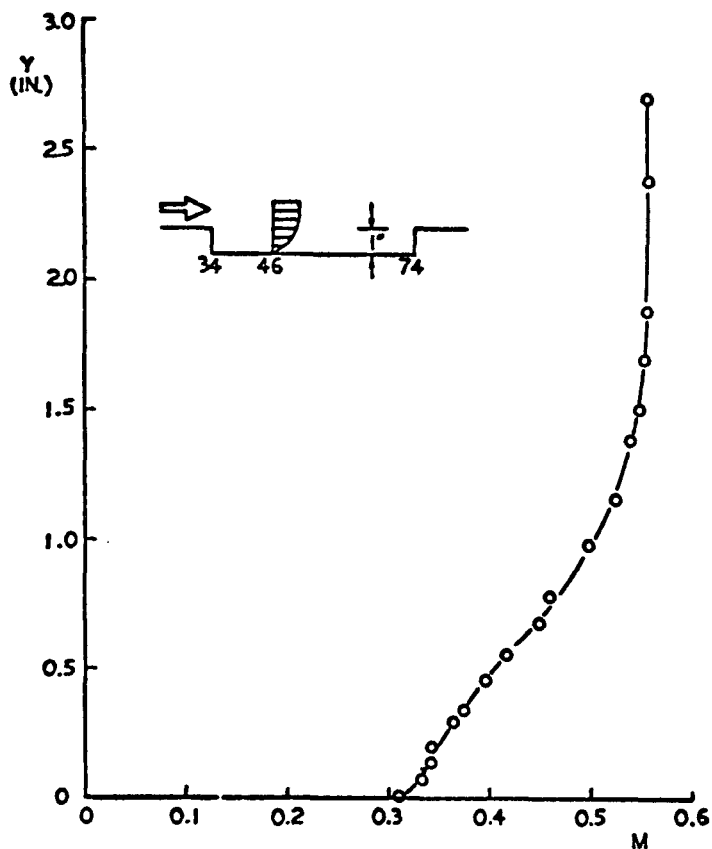
c. 46-inch Station, M_e = 0.56 , Re_L = 32.5 \times 10^6
