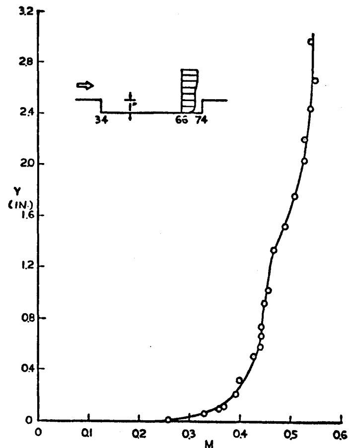
f. 66-inch Station, M_e = 0.54 , Re_L = 32.5 \times 10^6
