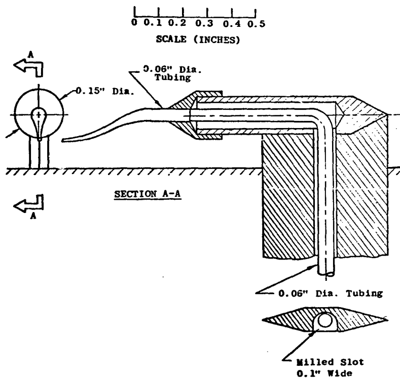
a. Cross-Sectional View
