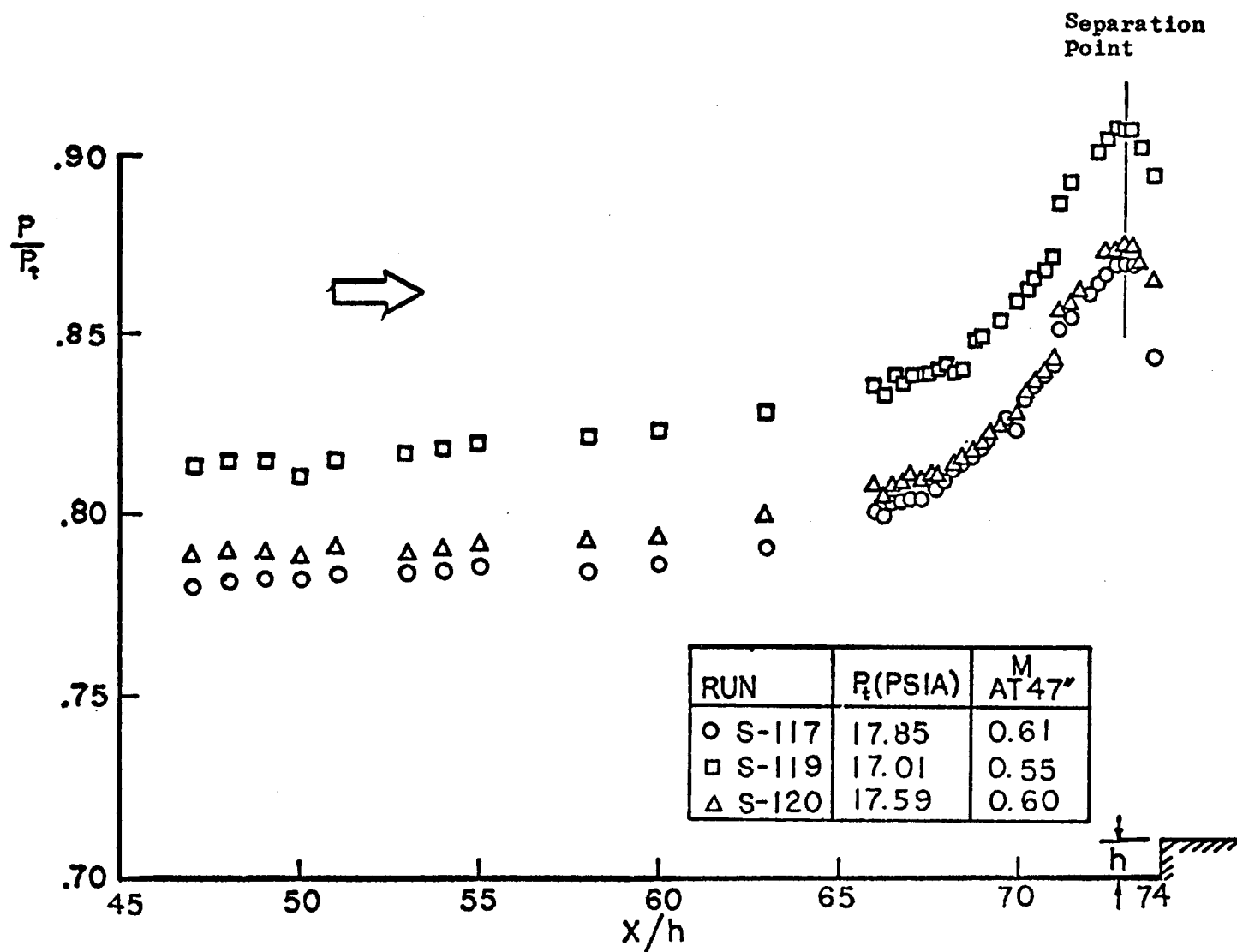
Figure 24. Forward Facing Step Model
