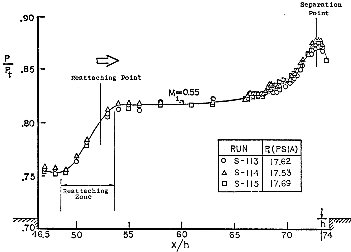
Figure 24d. 27.5 inch long cavity like model, M_i = 0.56 , Re_L = 32.5 \times 10^6
