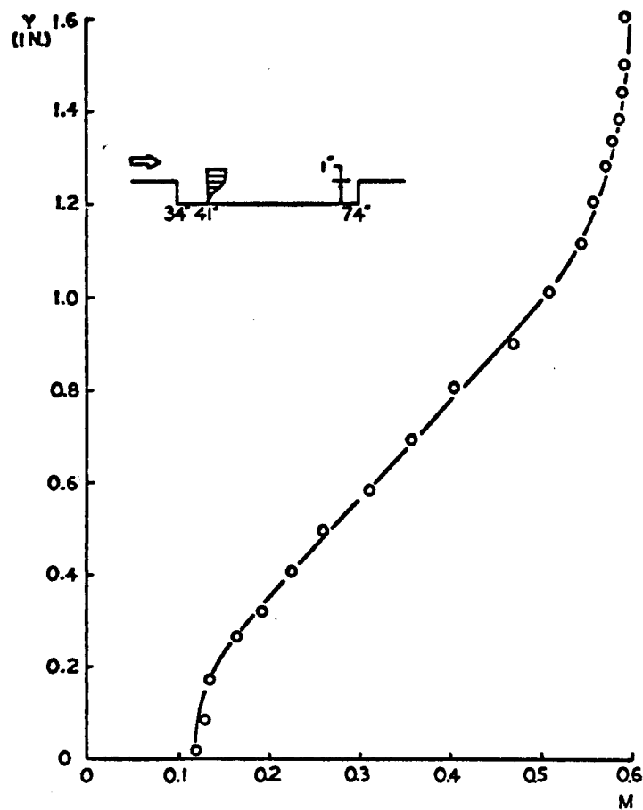
a. 41-inch Station, M_e = 0.60 , Re_L = 32.5 \times 10^6
