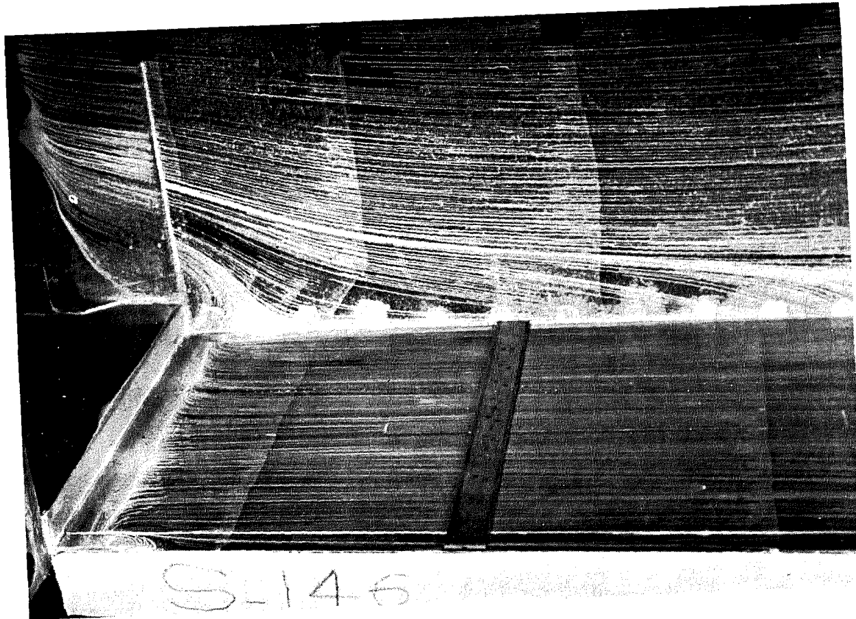
Figure 28. Surface oil photographs, M_e = 0.6 , Re_L = 32.5 \times 10^6
