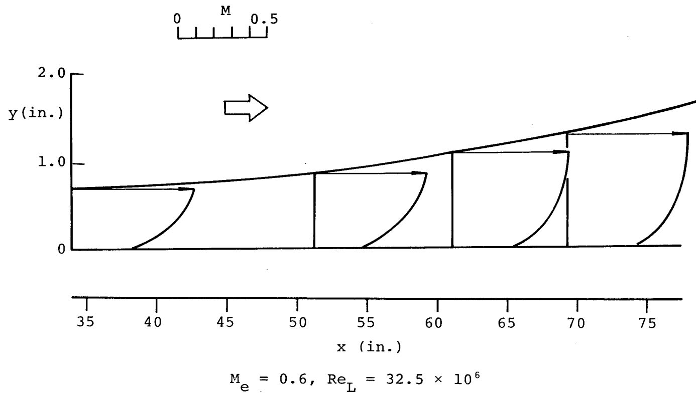
Figure 17. Flow variation along the flat-plate model.
