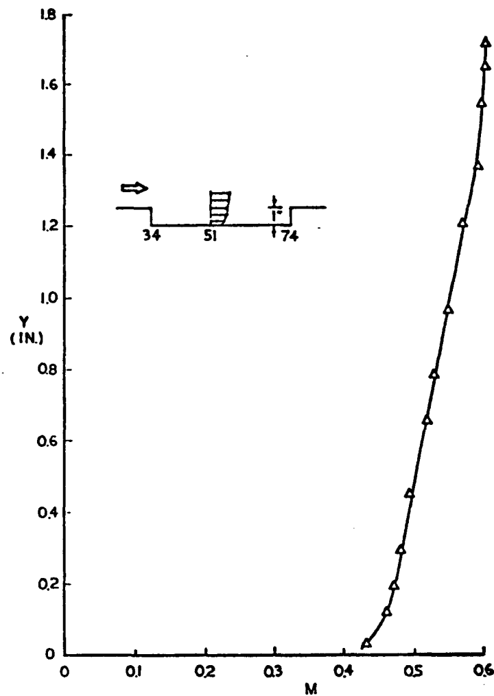
d. 51-inch Station, M_e = 0.60 , Re_L = 32.5 \times 10^6
