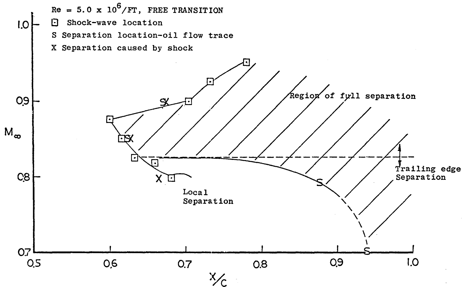
Figure 3. Variation of shock wave location with Mach number for C141 airfoil--from Ref. (7).
