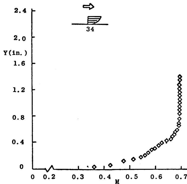
a. 34 Inch Station, M_e = 0.70 , Re_L = 32.5 \times 10^6 b. 51 Inch Station, M_e = 0.63 , Re_L = 32.5 \times 10^6
