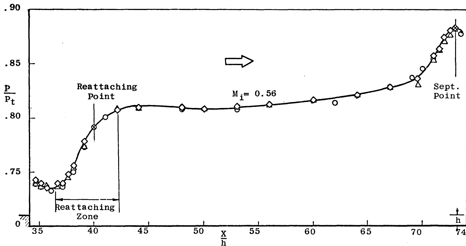
Figure 24c. 40 inch long cavity like model, M_i = 0.56 , Re_L = 32.5 \times 10^6 .
