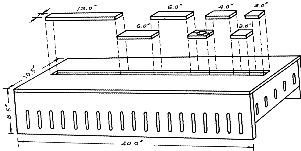
Figure 8. Typical slotted model block.
