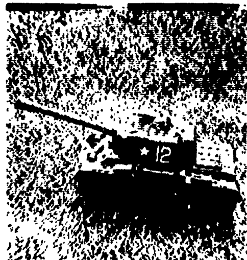
d) k = 3
