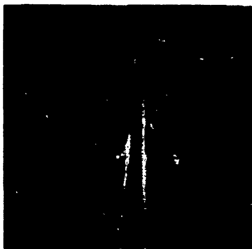
a) N = 1
