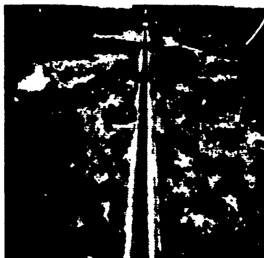
c) N = 4
