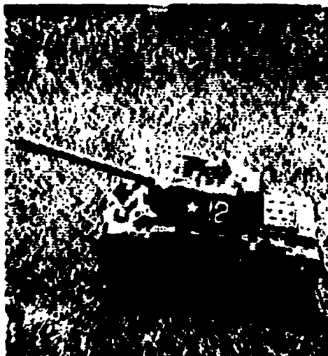
c) k = 2
