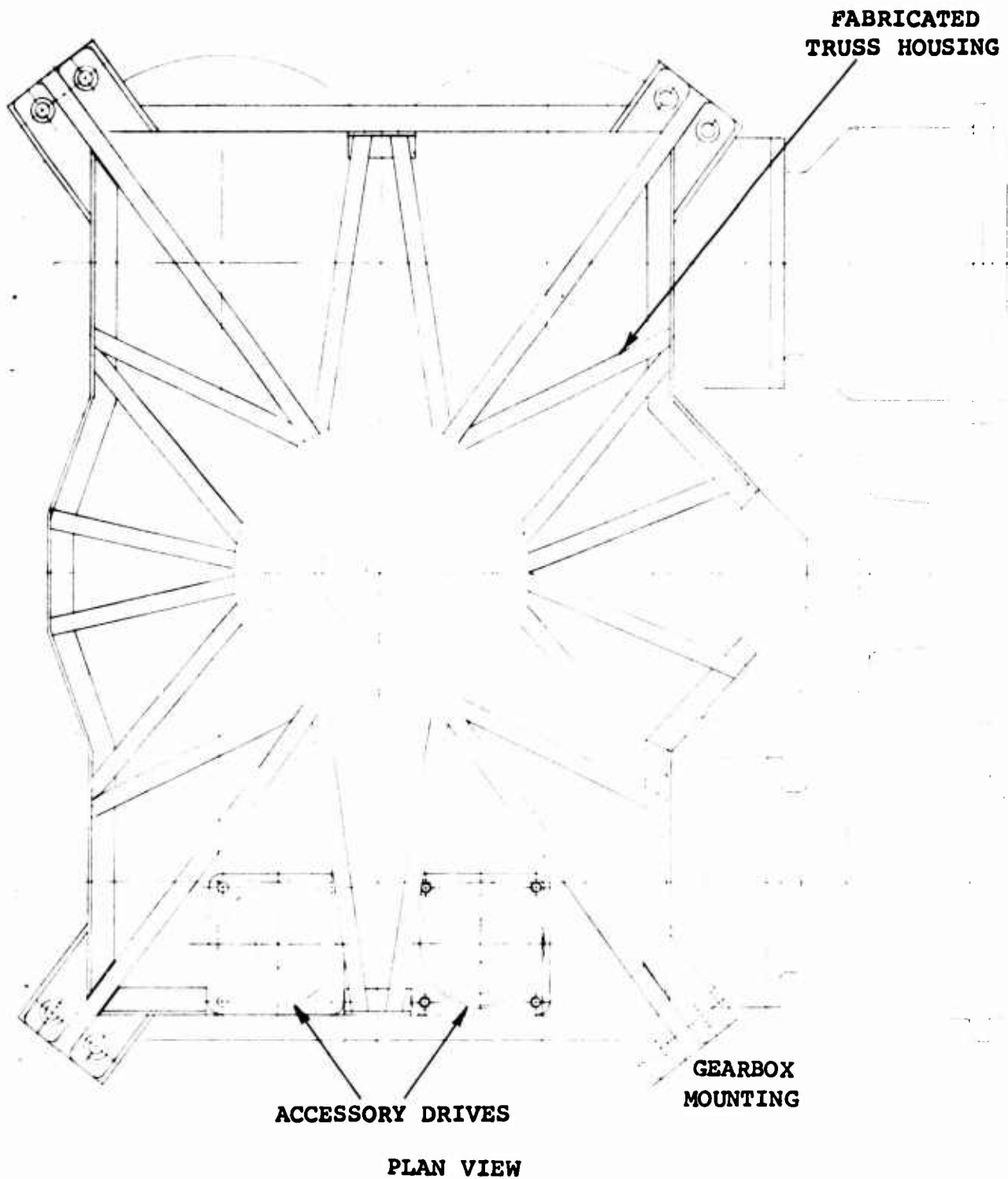
Figure 28. Split Power Transmission Layout.
