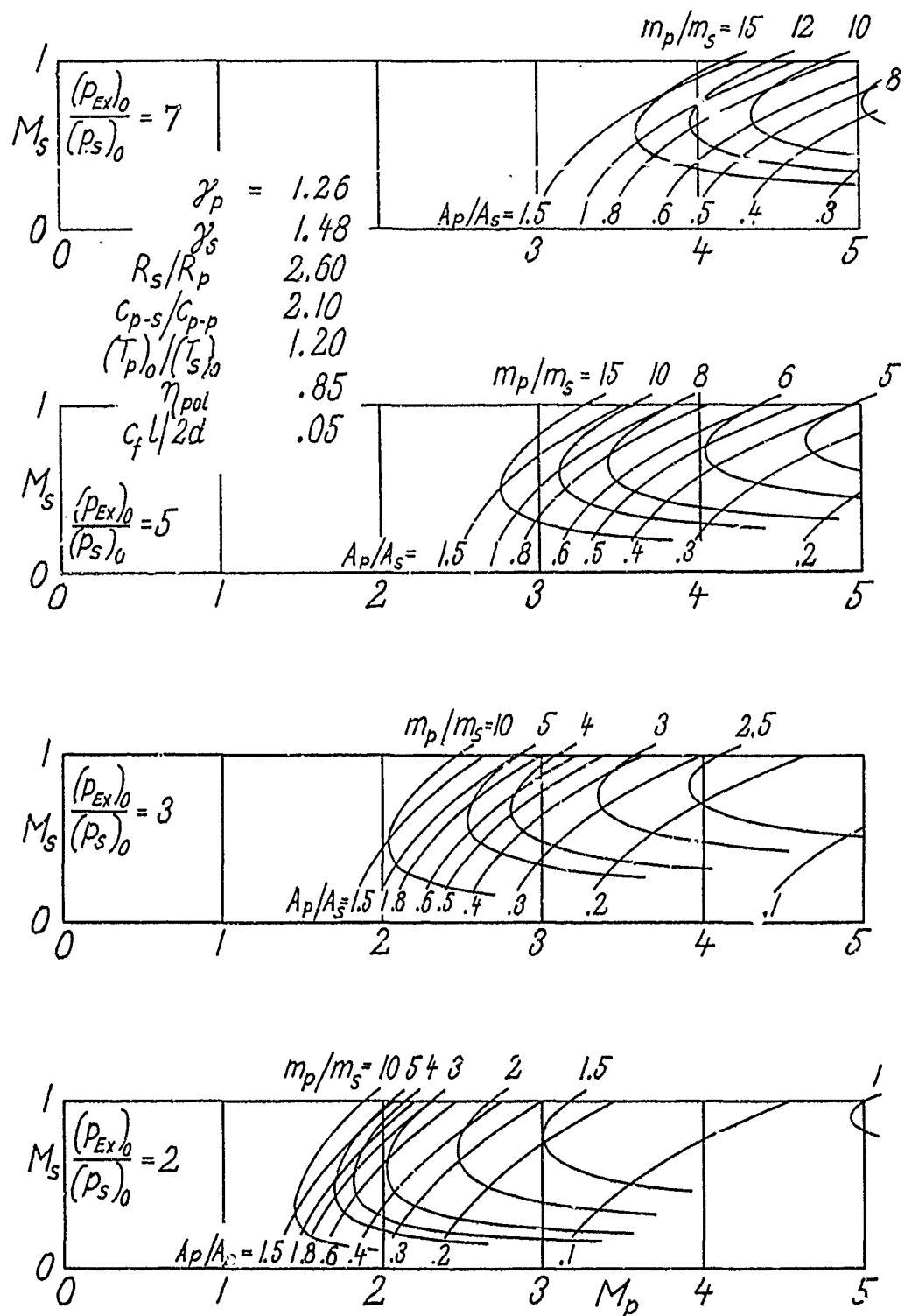
Figure 23. Performance Optimization for Constant Area Mixing for Four Different Total Ejector Pressure Ratio .
