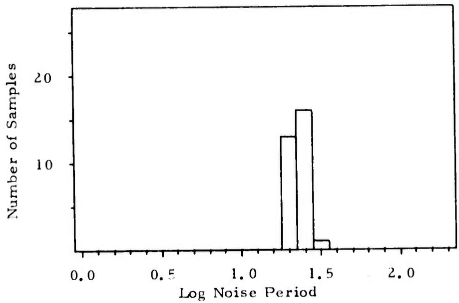
FIGURE B-5 LOG NOISE PERIOD DISTRIBUTION: STATION ALQ
