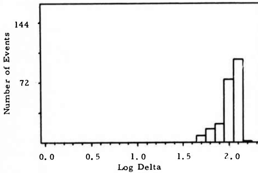
FIGURE A-20 LOG \Delta DISTRIBUTION, \Lambda \geq 50^\circ : STATION KIP
