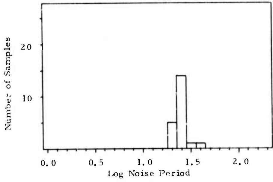
FIGURE B-6 LOG NOISE PERIOD DISTRIBUTION: STATION ZLP
