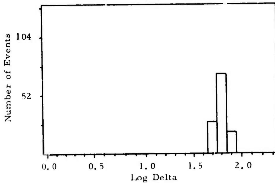
FIGURE A-14 LOG Δ DISTRIBUTION, Δ ≥ 50°: STATION CHG
