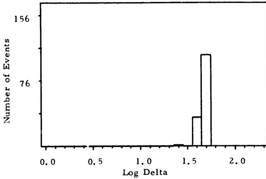
FIGURE A-19 LOG \Delta DISTRIBUTION, \Lambda < 50^\circ : STATION KIP
