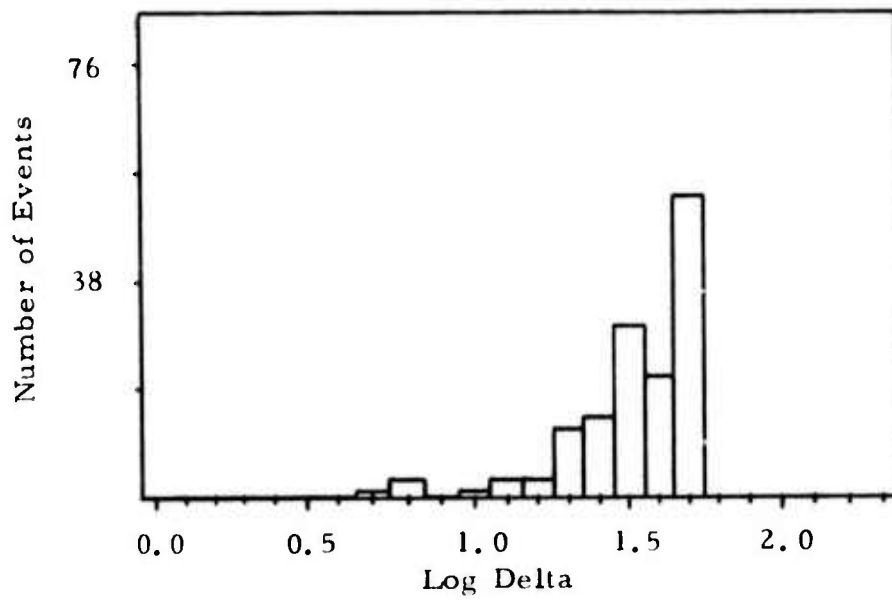
FIGURE A-13 LOG Δ DISTRIBUTION, Δ < 50°: STATION CHG
