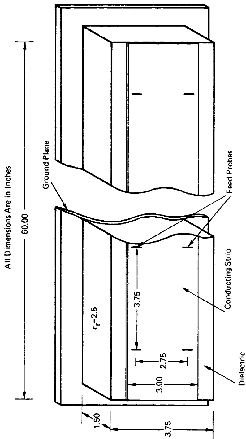
Fig. 30 Dimensions of the 16-Element Linear Array Aperture
