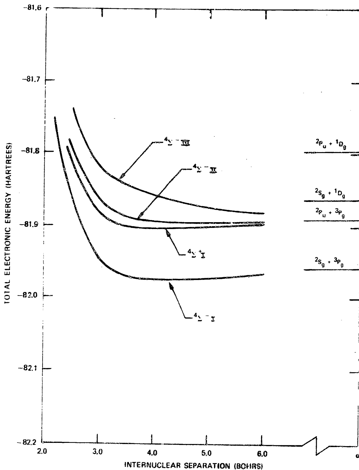
FIGURE 7. THE CALCULATED 4\Sigma^+, - STATES OF LiO
