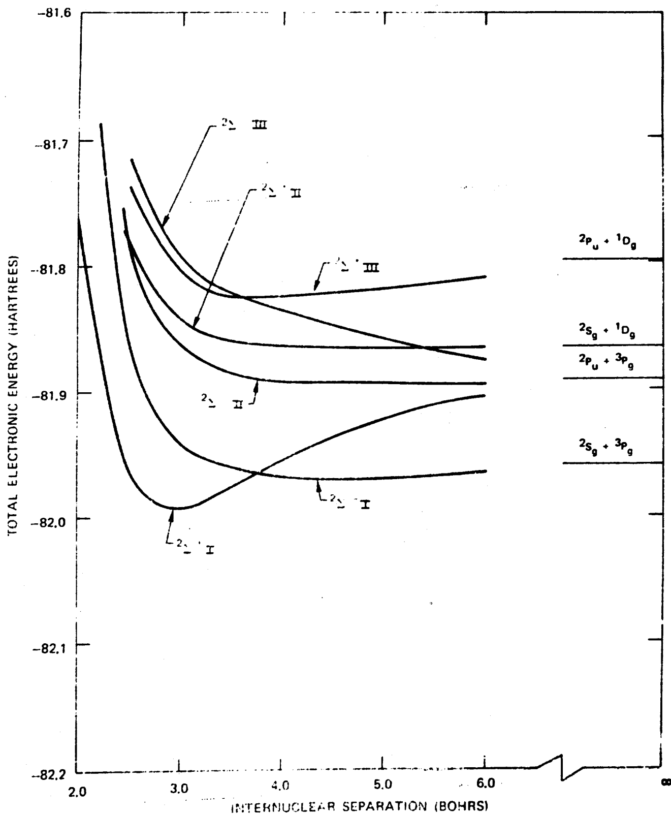
FIGURE 6. THE CALCULATED 2\Sigma^+ , 2\Sigma^- STATES OF LiO
