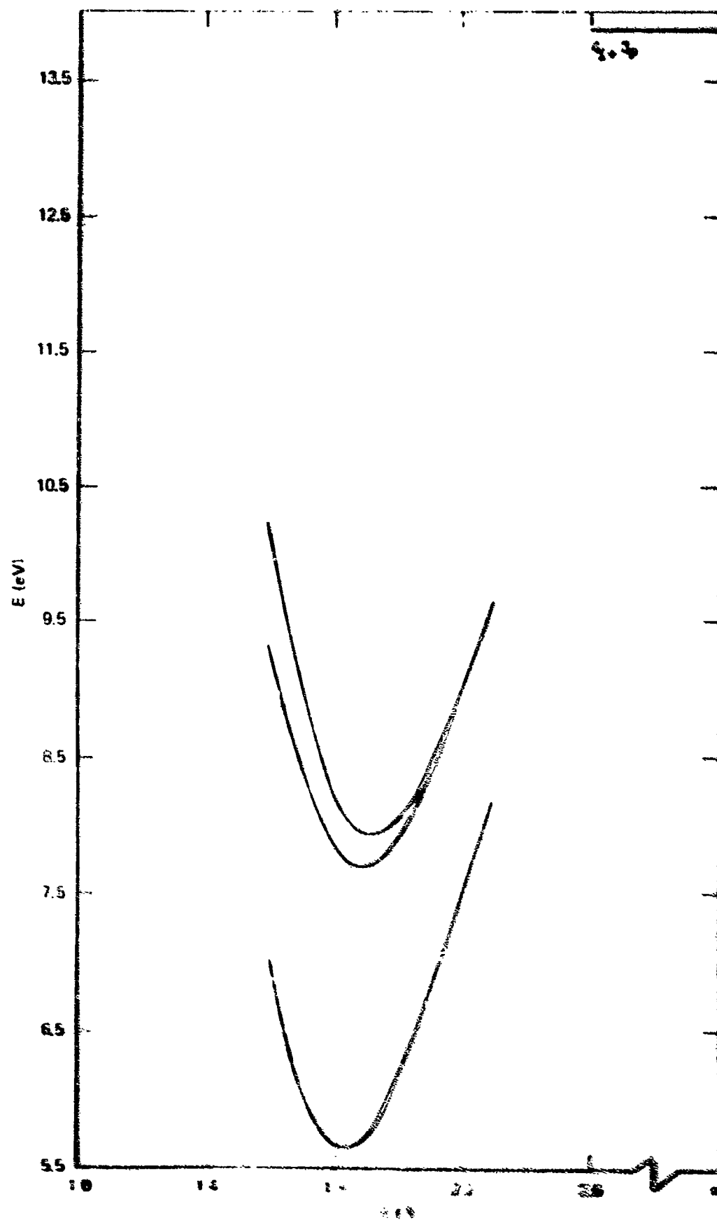
FIGURE 17 THE 6^{\text{th}} STATE OF \text{Fe}^{2+}
