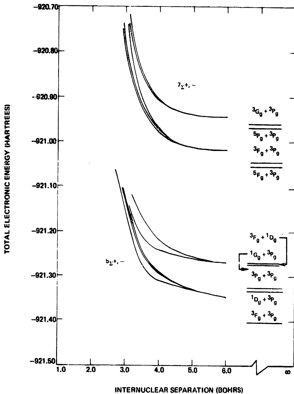
Figure 37. The calculated 5\Sigma^{+,-} and 7\Sigma^{+,-} states of \text{TiO}
