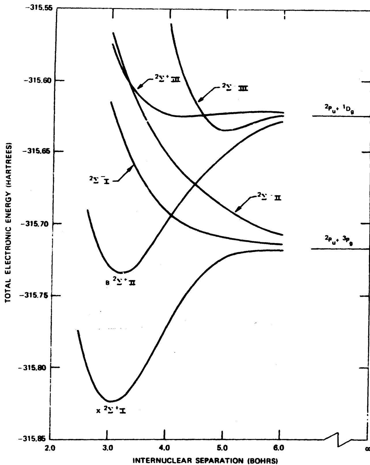
FIGURE 1. THE CALCULATED 2\Sigma^+, - STATES OF \text{AlO}
