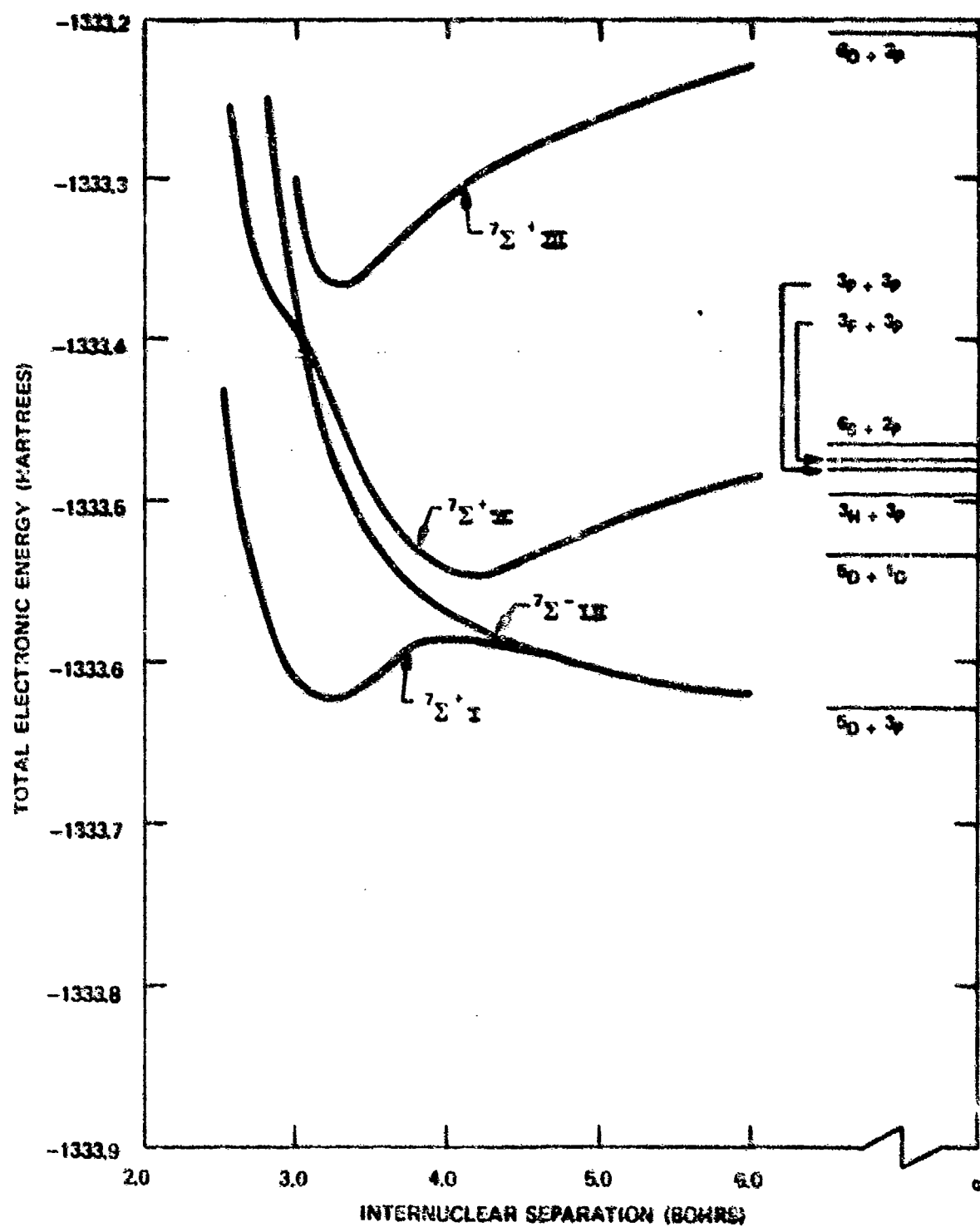
FIGURE 14. THE CALCULATED 7\Sigma^+ \text{ -- } 7\Sigma^- STATES OF FeO
