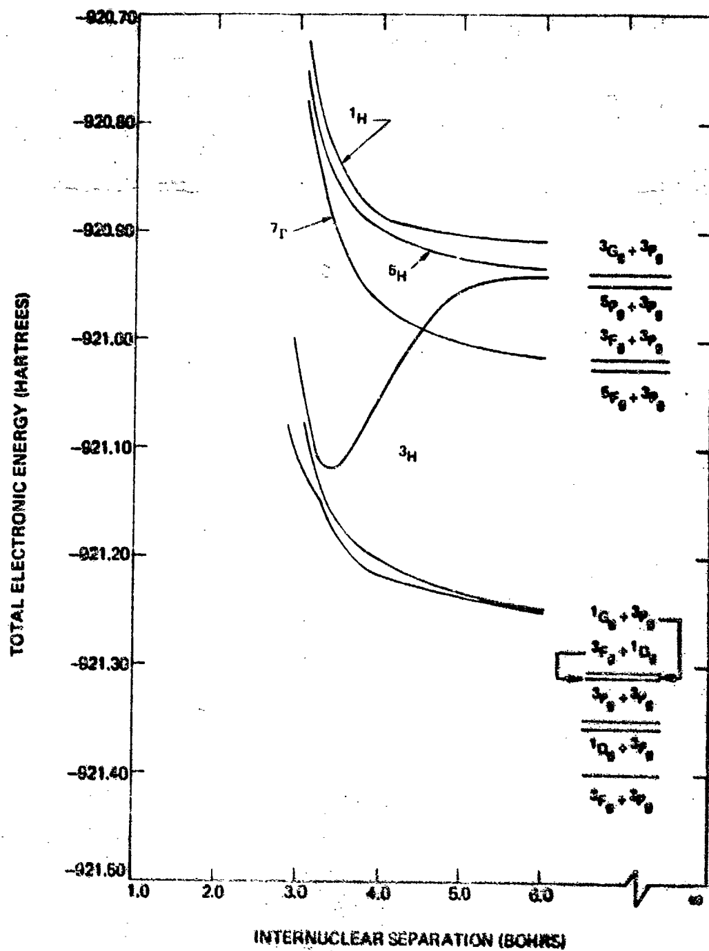
Figure 52. The calculated 7\Gamma , 1H , 3H and 5H states of TiO
