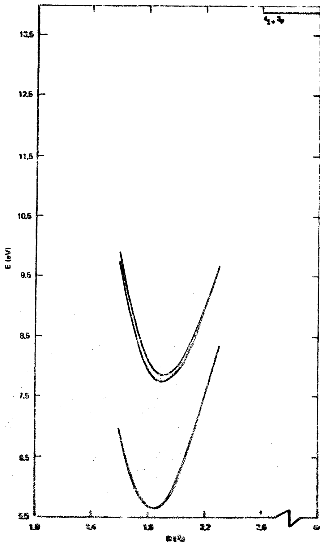
FIGURE 11. THE 1s STATE OF U^{2+}
