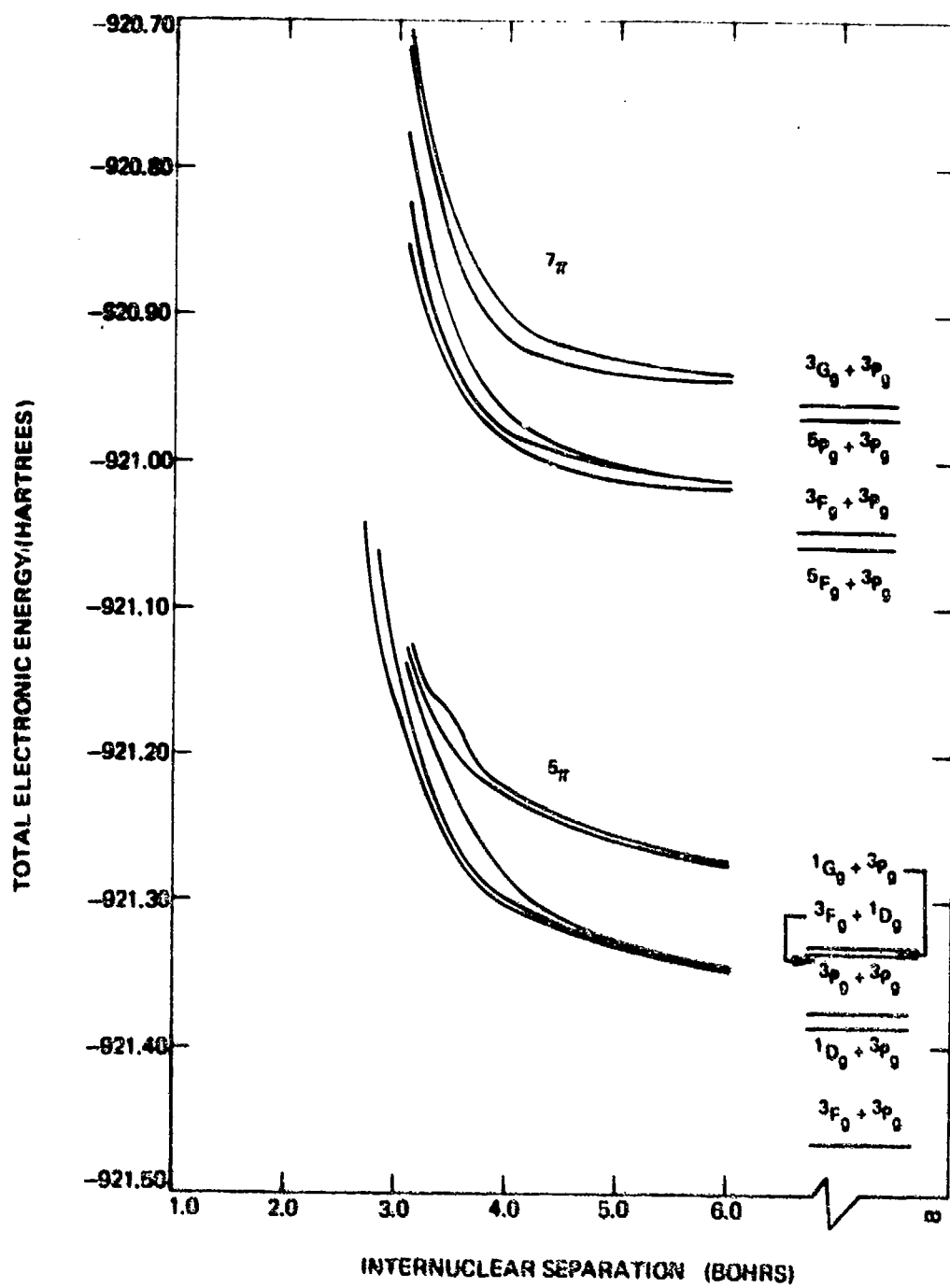
Figure 40. The calculated 5\Pi and 7\Pi states of \text{TiO}
