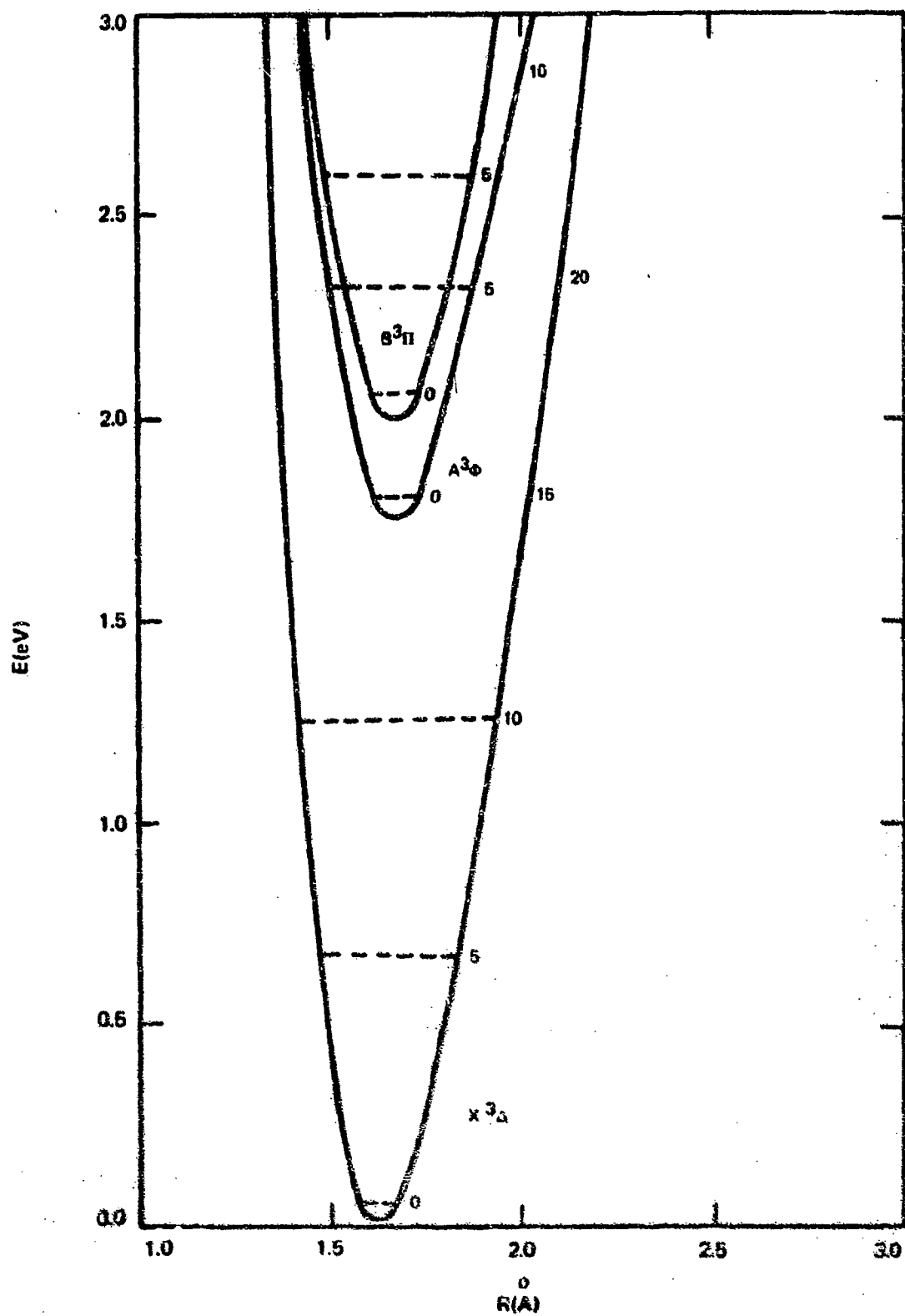
FIGURE 53. RKR POTENTIAL ENERGY CURVES FOR TiO
