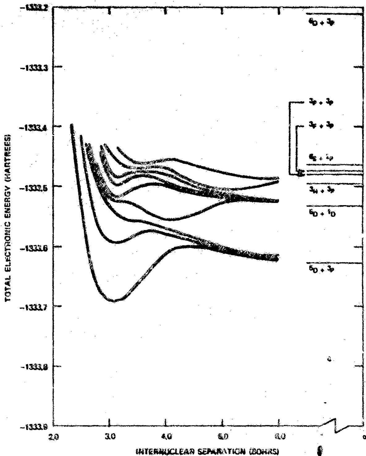
FIGURE 15. THE CALCULATED 5 \Pi STATES OF FeO
