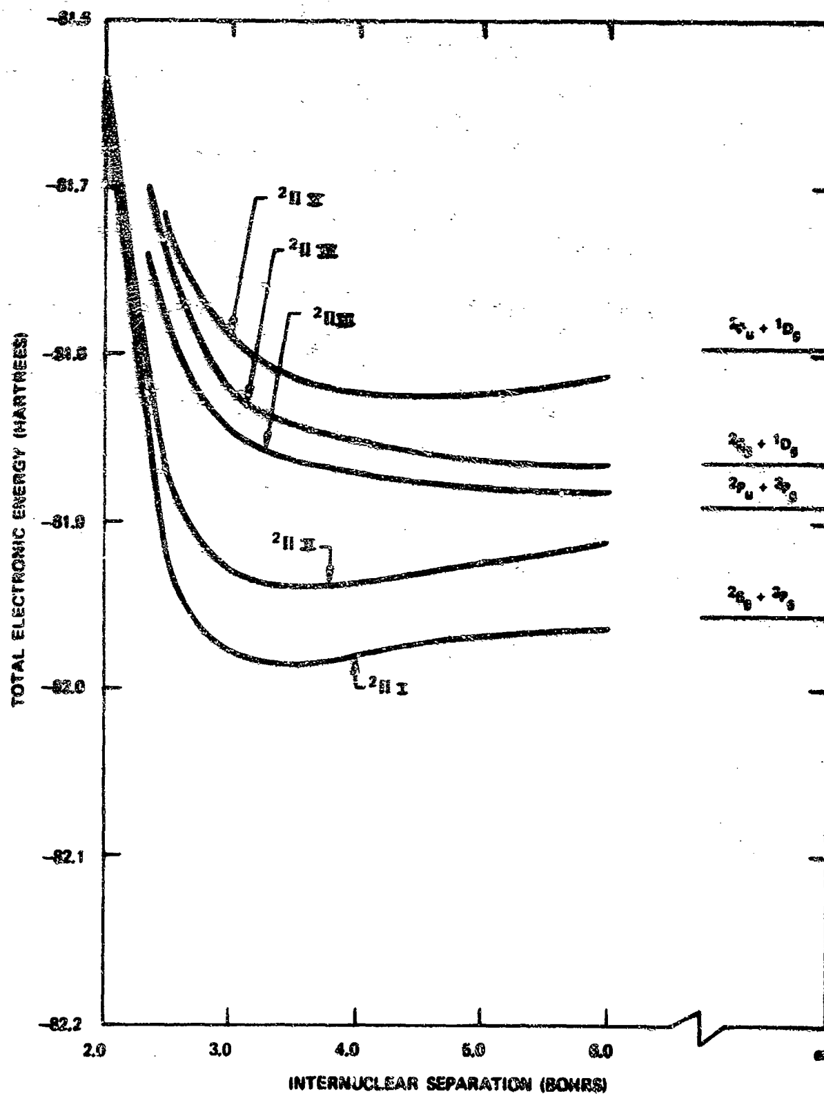
FIGURE 8. THE CALCULATED 2\Pi STATES OF LiO
