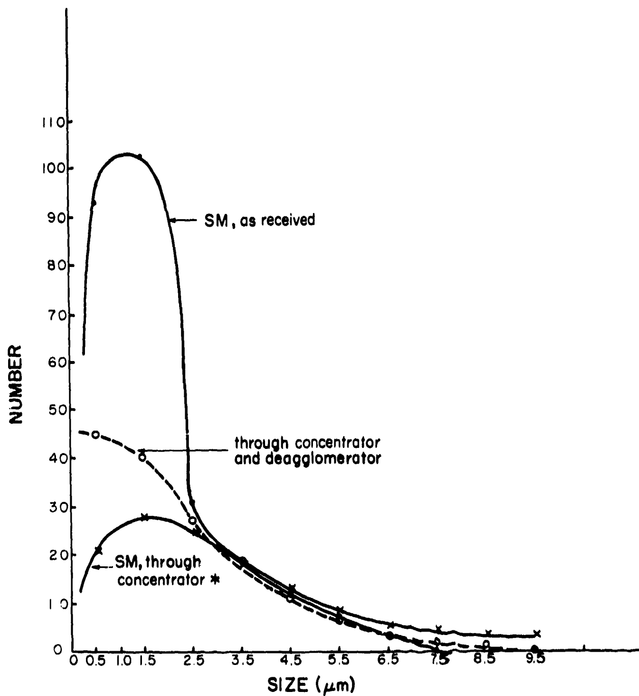
FIGURE 19. Particle size distribution of SM particles (normalized to same value at 3.5 \mu m for comparison).
