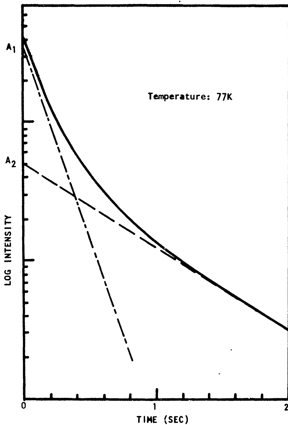
Fig 26 Phosphorescence decay of \text{RDX}_{d-6}
