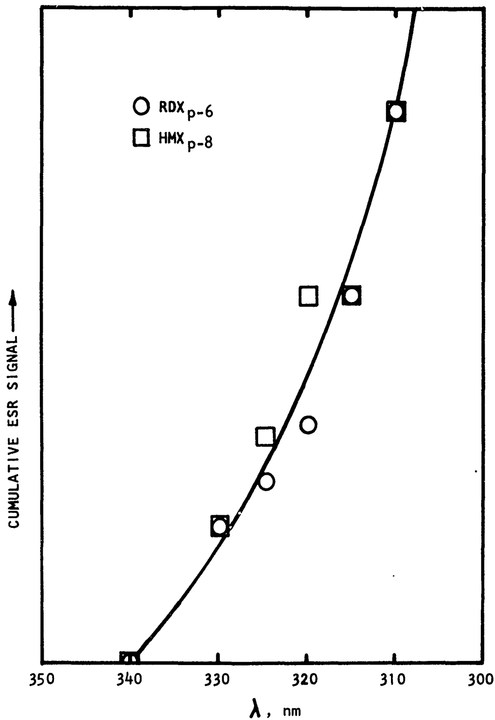
Fig 27 Threshold wavelength for photodecomposition in RDX and HMX
