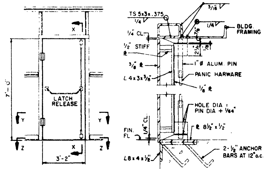
EXTERIOR ELEVATION
