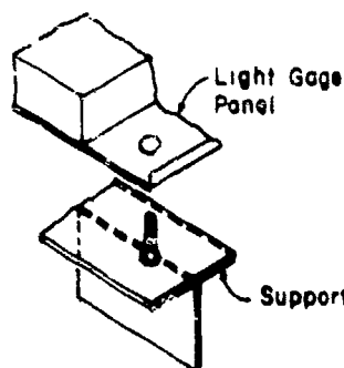
THREADED NELSON TYPE STUDS
