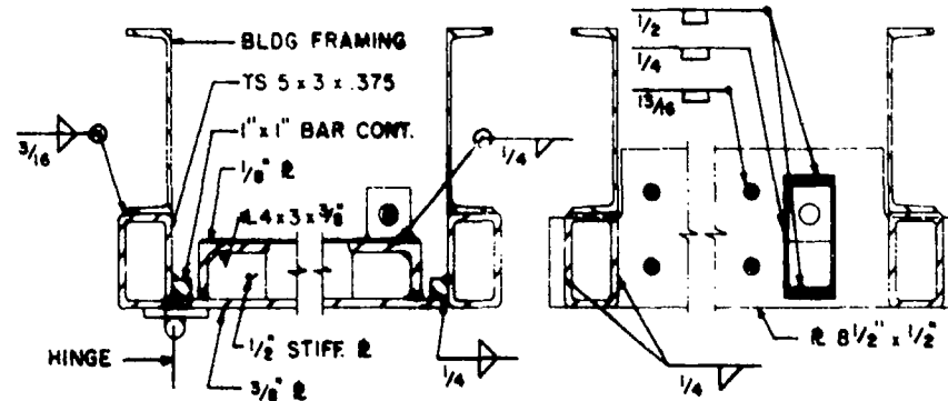
SECTION X-X
