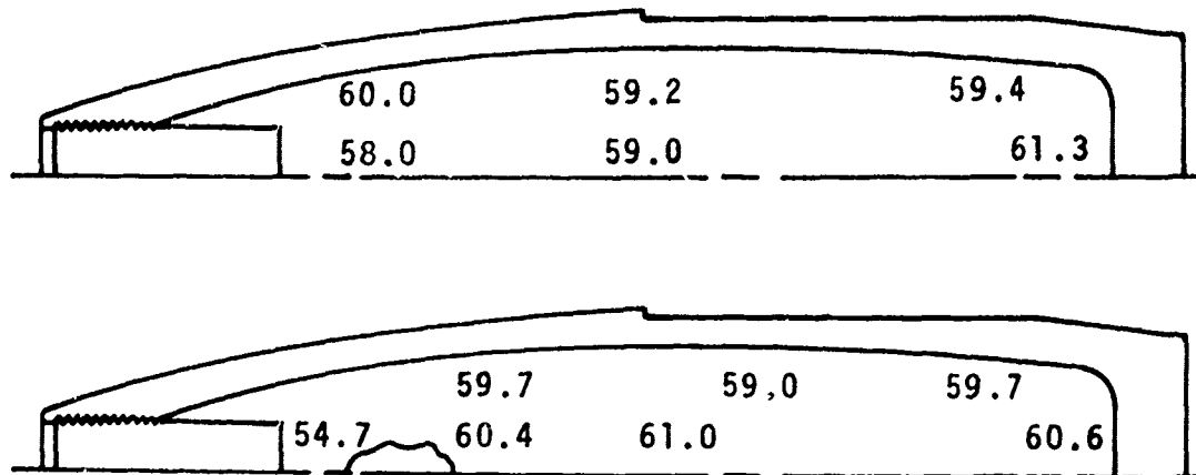
Figure 30. RDX Analysis (%)
