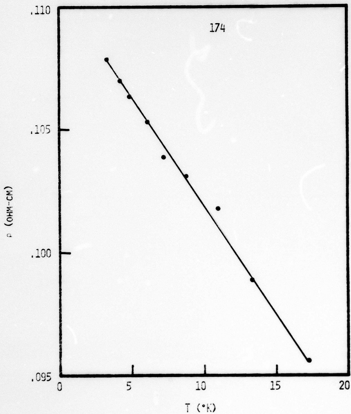
Figure 3.3 Resistivity versus absolute temperature for sample 174 for T < 20^{\circ}\text{K} .
