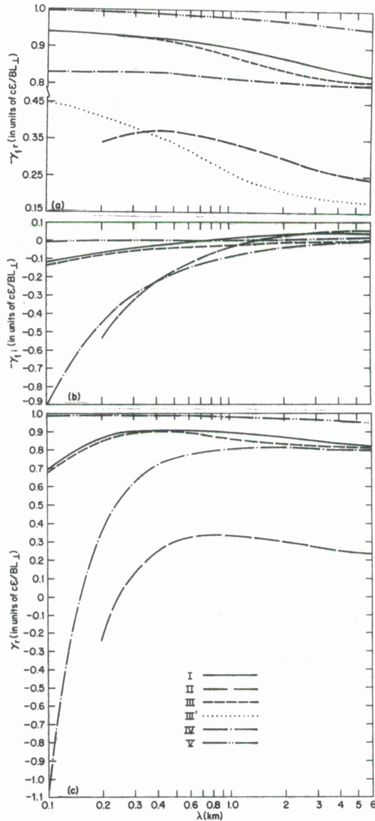
Fig. 15 — Eigenvalues for Cases (I) - (V). a) the zero temperature growth rate, \gamma_{1r} , in units of c\epsilon/BL_{\perp} . "III'" refers to \Sigma_p/\Sigma_p^1 = 0.2 , but with neglect of image density transport; b) \gamma_{1i} , the zero temperature frequency in units of c\epsilon/BL_{\perp} ; c) \gamma_r , the growth rate appropriate to T = 10^3 K, \epsilon = 5 mV/m, in units of c\epsilon/BL_{\perp} . [Eq. (15) with d\gamma_1/dz = 0 , relates \gamma to \gamma_1 .]
