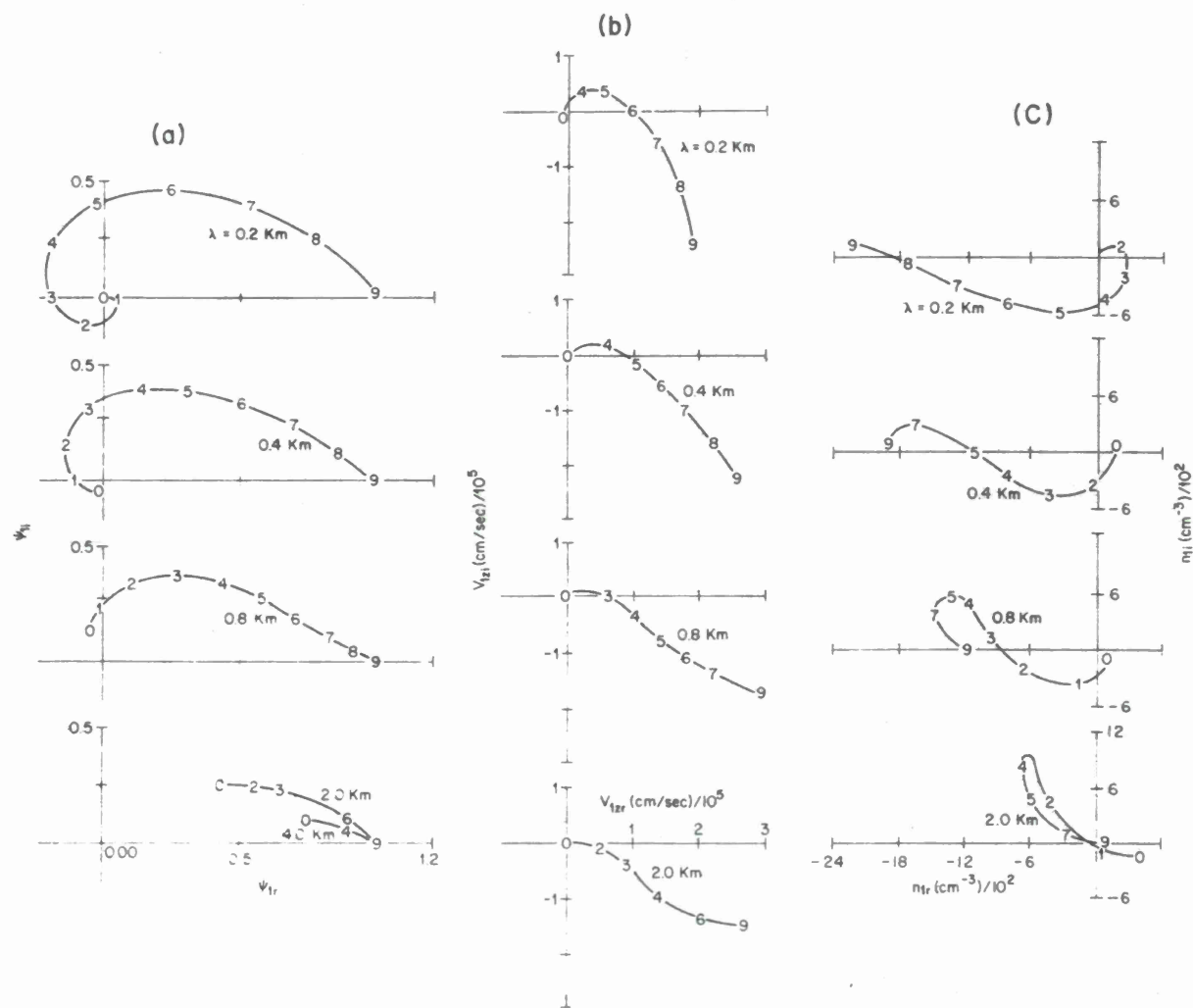
Fig. 13 — Hodographs for Case IV. Digits m along curves indicate values at altitude given by (100 + 10m)\text{km} . a) \psi_{1i}(z) vs \psi_{1r}(z) . |\psi_1(z)| is given by distance from origin. The striation structure has period \lambda along y . Locations in phase with \psi_1(190) at y = 0 are given by y = -\xi(z)\lambda/2\pi where \xi(z) is the polar angle. b) v_{1zi}(z) vs v_{1zr}(z) . |v_1(z)| is given by distance from origin. Locations in phase with \psi_1(190) are given by y = -\xi(z)\lambda/2\pi where \xi(z) is the polar angle. c) n_{1i}(z) vs n_{1r}(z) . |n_1(z)| is given by distance from origin. Locations in phase with \psi_1(190) are given by y = -\xi(z)\lambda/2\pi , where \xi(z) is the polar angle.
