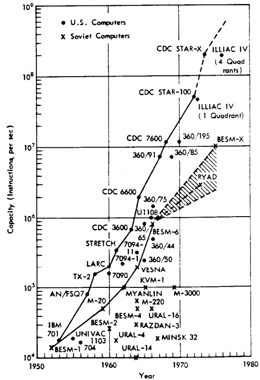
Fig. 4 — Comparison of U.S. and Soviet high-performance computers
