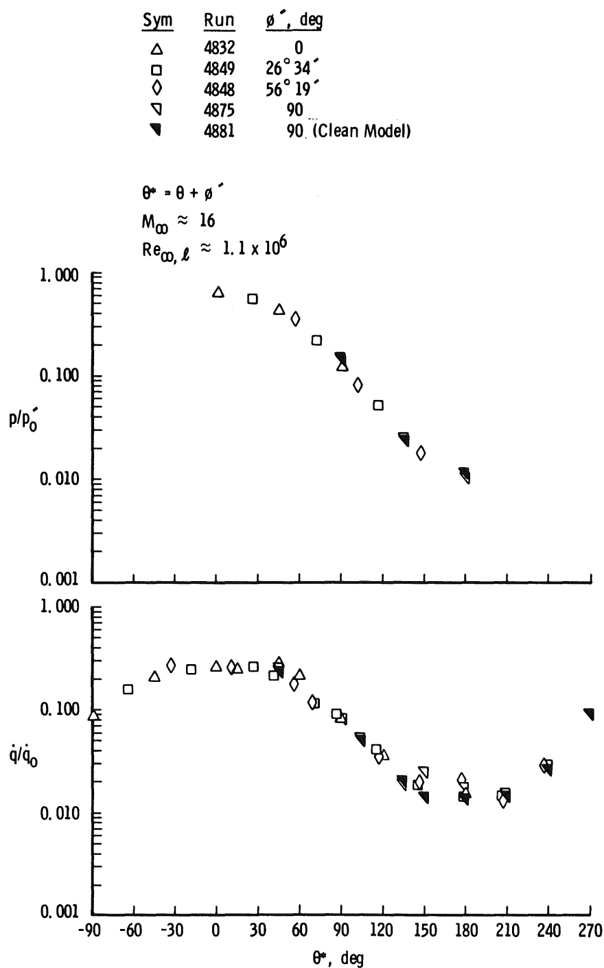
Figure 11. External tank peripheral heat-transfer and pressure distributions for \alpha' = -30 deg.
