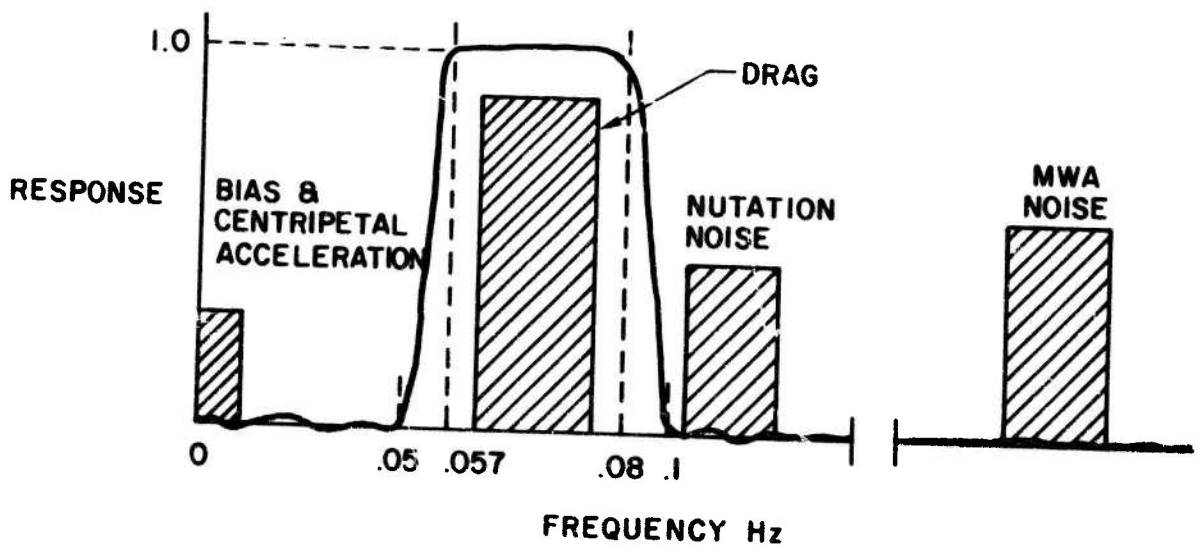
Figure 10. Band-Pass Filter
