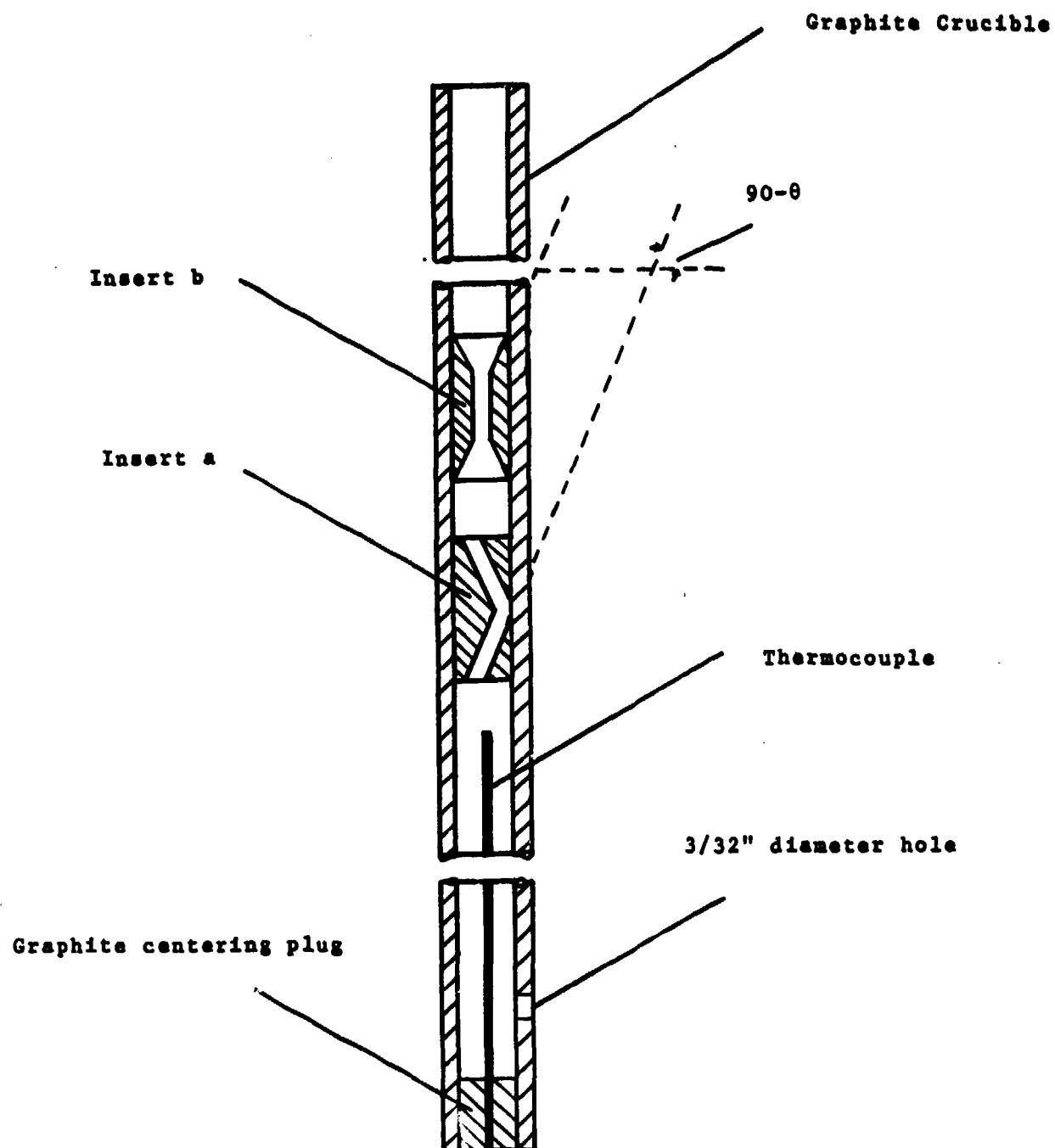
Figure 16. Cross-sectional view of crucible and insert system.
