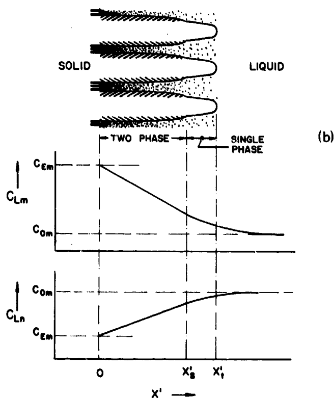
Figure 29. Schematic illustration showing the growth of cells or dendrites in a ternary system. (a) Phase diagram showing solidification path (full line) and diffusion path for a planar interface (dashed line). (b) Intercellular liquid composition. Primary phase solidifies first and, when the liquid composition reaches C_{2f} , two-phase material is formed.
