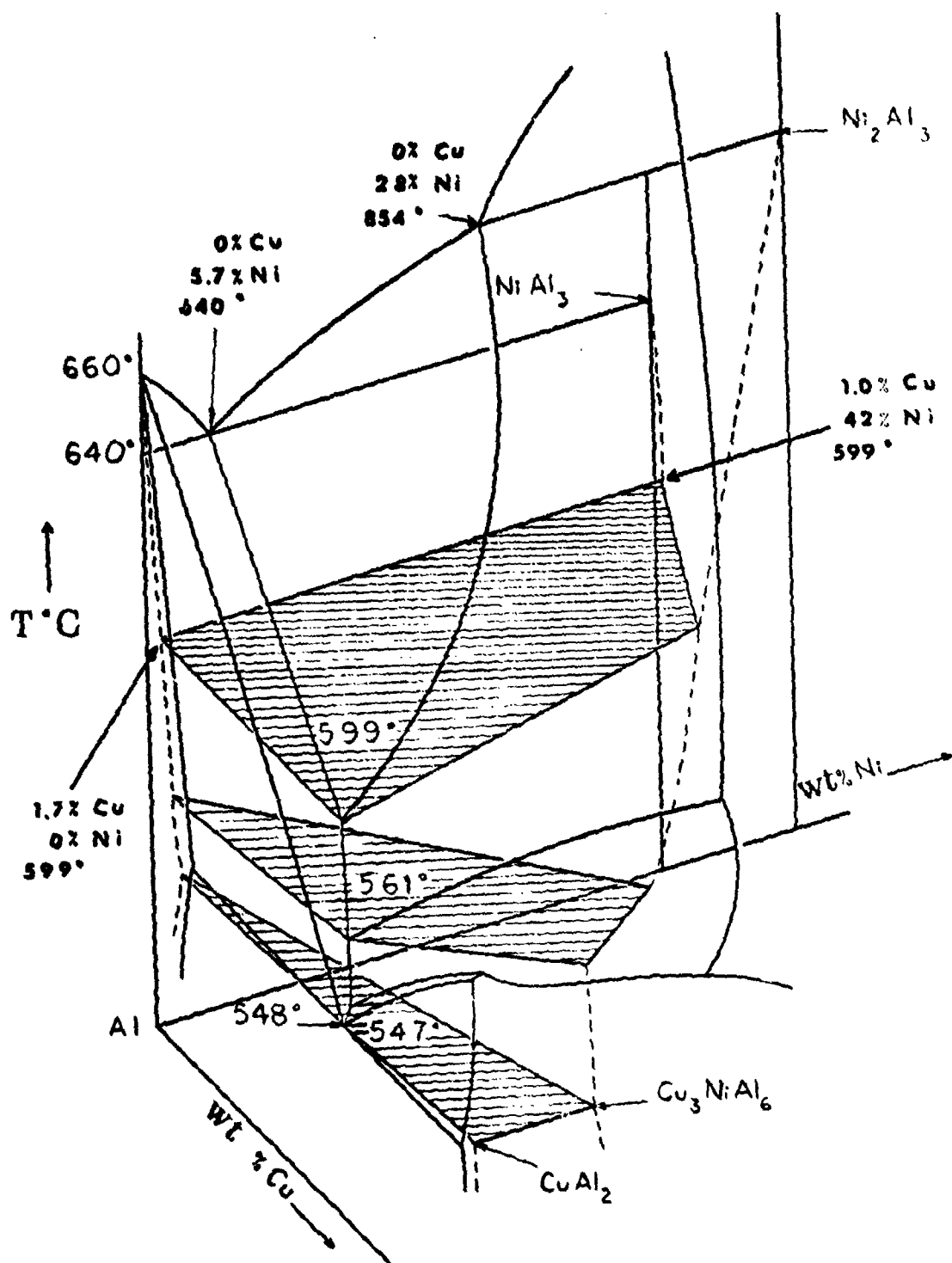
Figure 8. Aluminum-rich corner of Al-Cu-Ni system.
