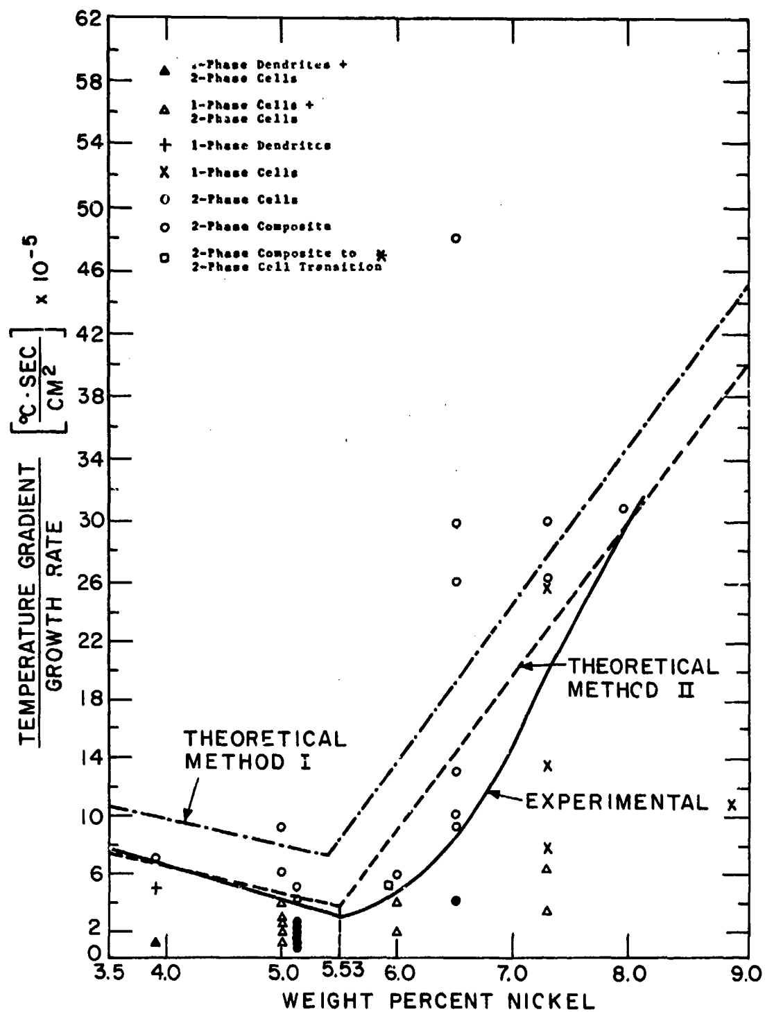
FIGURE 2. STRUCTURE OF DIRECTIONALLY SOLIDIFIED INGOTS AS A FUNCTION OF G/R AND C_{\text{ONi}} WITH C_{\text{OCu}} = 1 \text{ wt \% Cu} . * REFERENCE RINALDI, SHARP AND FLEMINGS.
