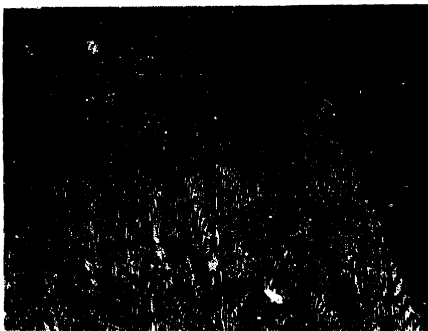
Figure 17. Insert b, lower portion, structure aligned in the original growth direction, longitudinal view, 115X. (a) Sample No. 0008, binary Al-Ni eutectic, \theta = 18^\circ . (b) Sample No. 0014, ternary Al-Ni-Cu eutectic, \theta = 10^\circ , corresponding schematic Figure 18.
