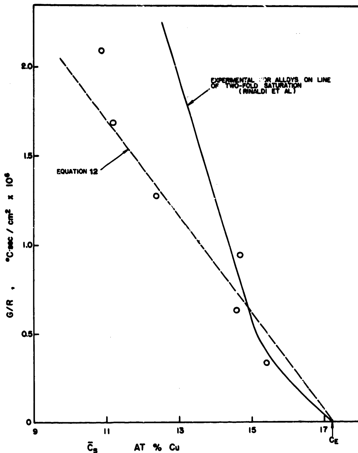
Figure 31. Average copper concentrations of interdendritic eutectic plotted as in Figure 3 for ternary Al-Cu-Ni system. The theoretical line is calculated from equation 12.
