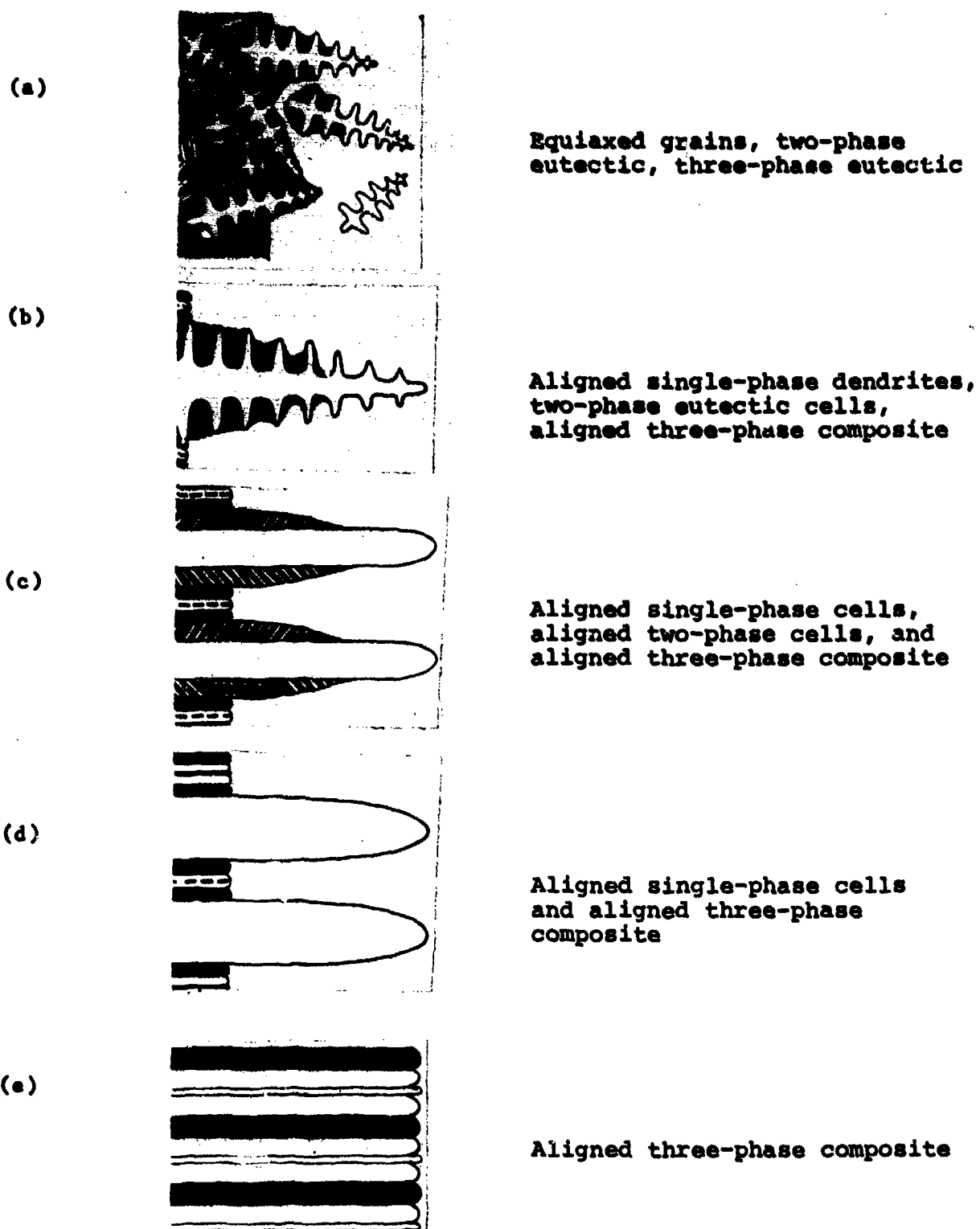
Figure I. Various possible microstructures obtained from three-phase alloys, in order of increasing G/R.
