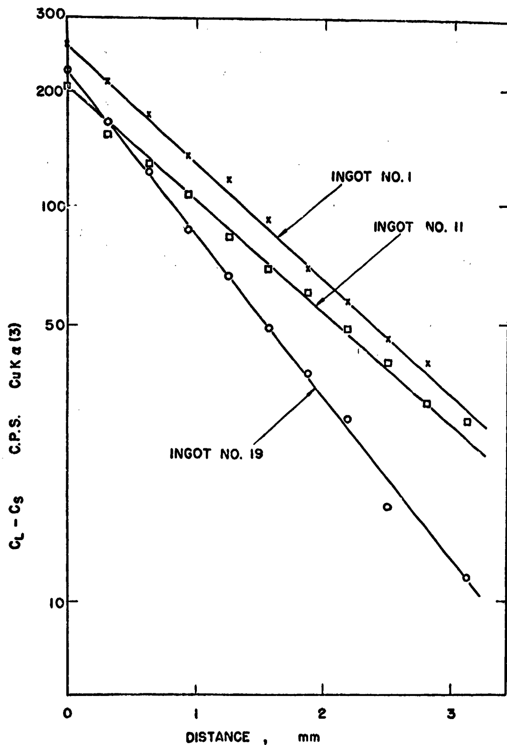
Figure 13. \ln(C_L - C_S) for Cu versus distance from the quenched interfaces in ingot #'s 1, 11 and 19.
