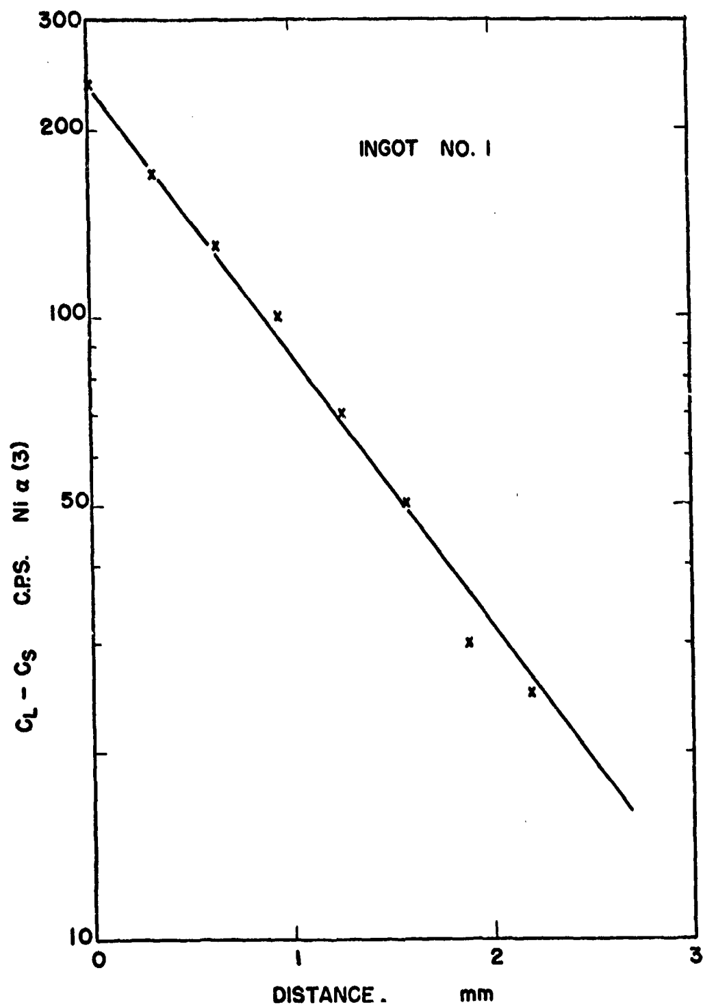
Figure 14. \ln(C_L - C_S) for Ni versus distance from the quenched interface in ingot #1.
