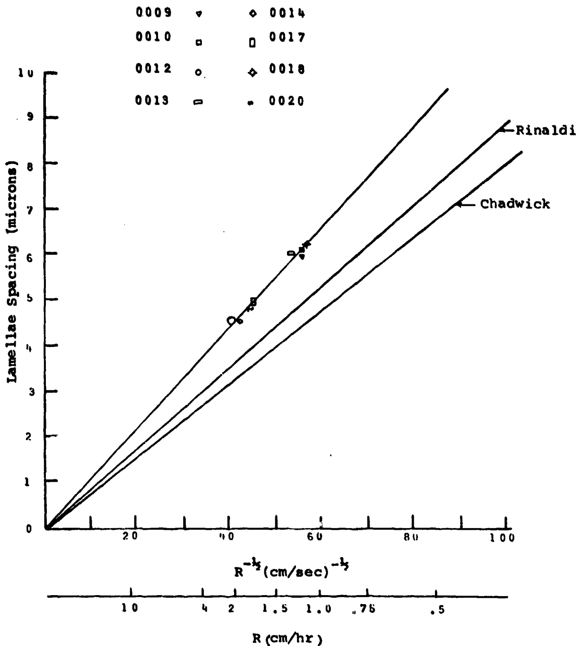
Figure 21. Lamellae spacing as a function of growth rate for ternary Al-Ni-Cu eutectic, Rinaldi's data 3 for compositions containing from 17.5 to 12.3 at. pct. Cu and from 0.0 to 1.32 at. pct. Ni, Chadwick's 22 data for the Al-Cu binary eutectic.
