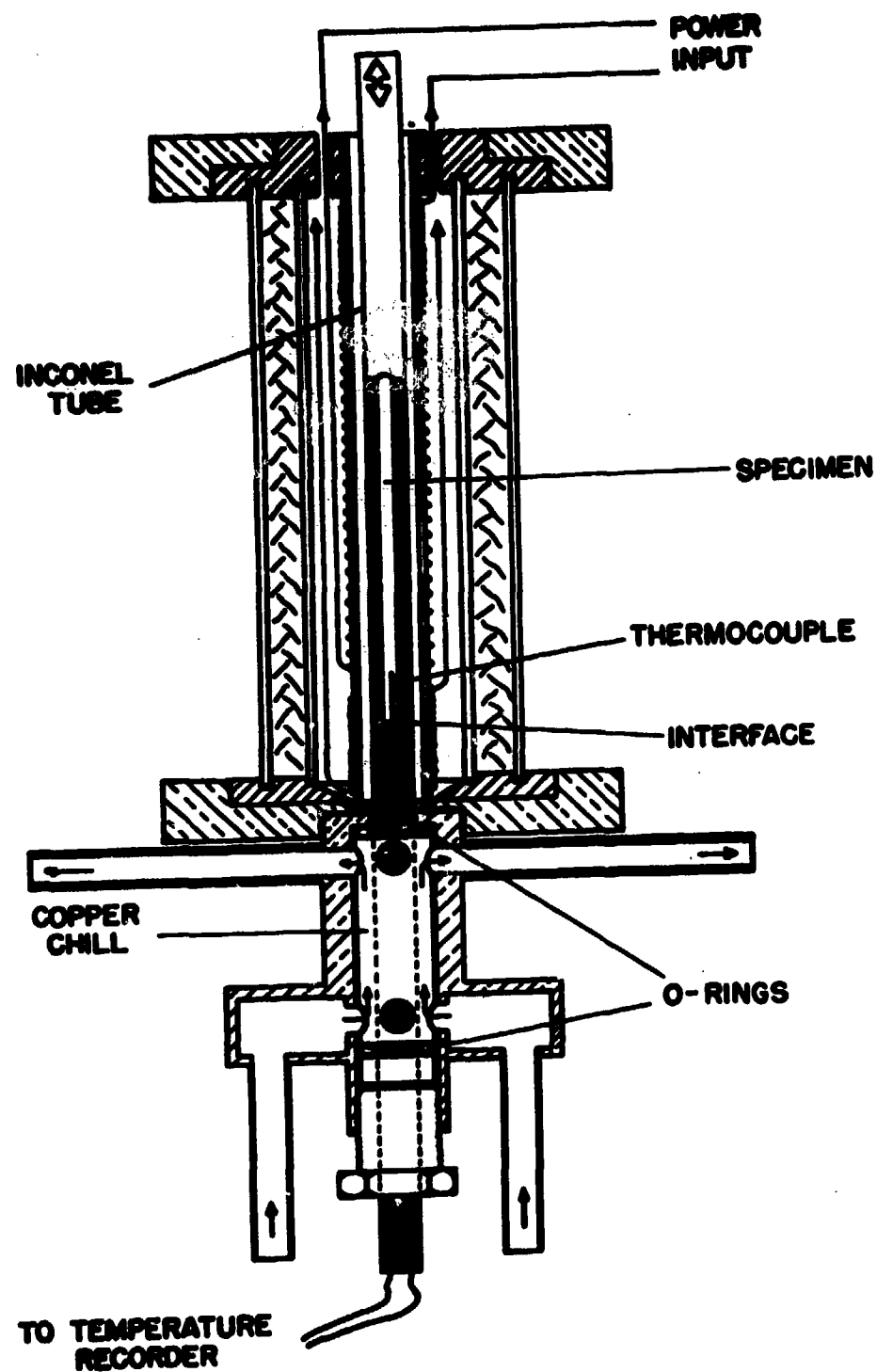
Figure 2. Schematic representation of the furnace-chill assembly of the apparatus used by Rinaldi et al.
