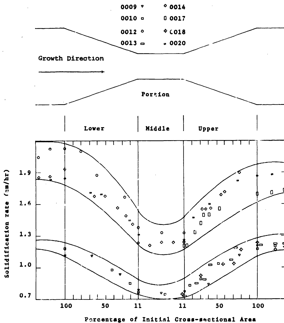
Figure 23. Solidification rate at various percentages of initial cross-sectional area into the portions of insert type b, ternary Al-Ni-Cu eutectic.
