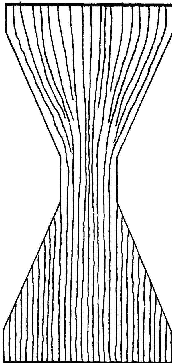
Figure 20. Schematic view of insert type b, \theta < 8^\circ , showing the structure following the contour of the insert at the upper portion.
