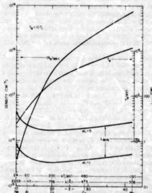
Fig. 2. Minimum length L_{\min} for amplification in carbonlike ions with gain \exp(\alpha L) vs atomic number Z , wavelength \lambda , and ion kinetic temperature kT_i . The electronic kinetic temperature kT_e is assumed equal to 10 kT_i and is plotted. Maximum electron density (N_e)_{\max} is also shown.
