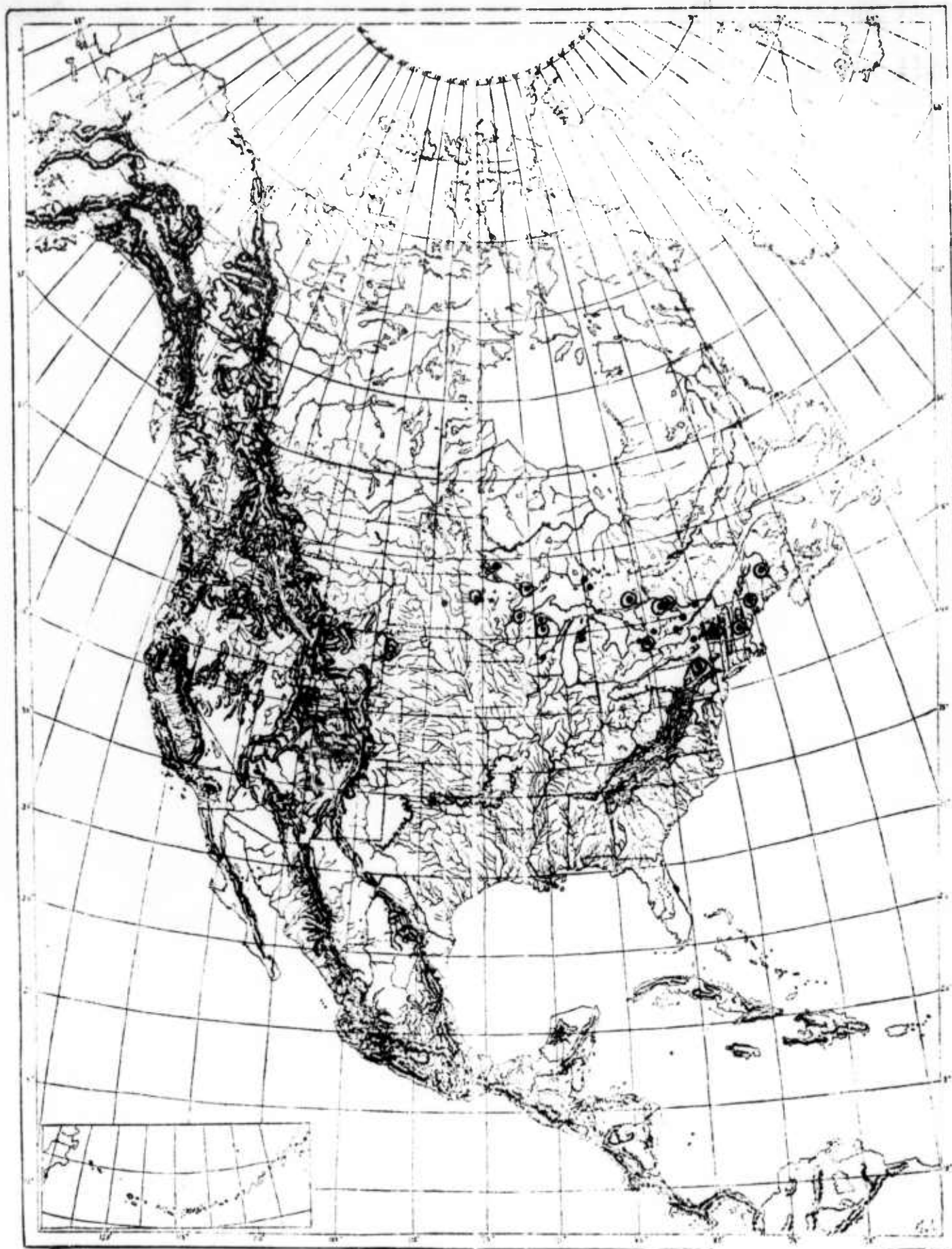
Figure 9 . Locations of lakes with varved sediments. Circled points indicate lakes with varves that are adequate for dating purposes.
