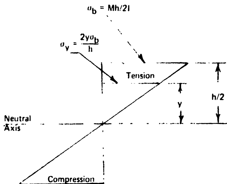
STRESS DISTRIBUTION
