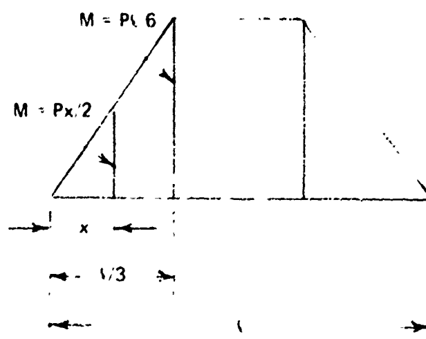
MOMENT DISTRIBUTION
