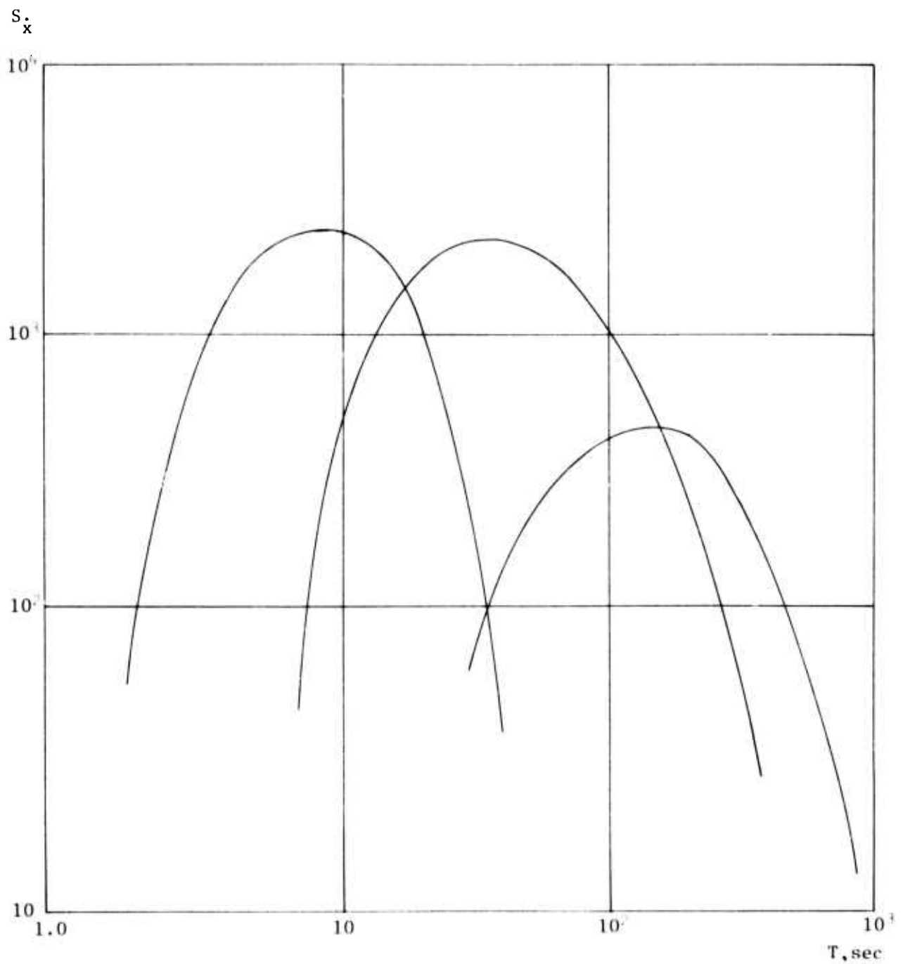
Fig. 57 -- Velocity sensitivity curves of the PSS system operating at the Sochi station during the late 1960s [84]
