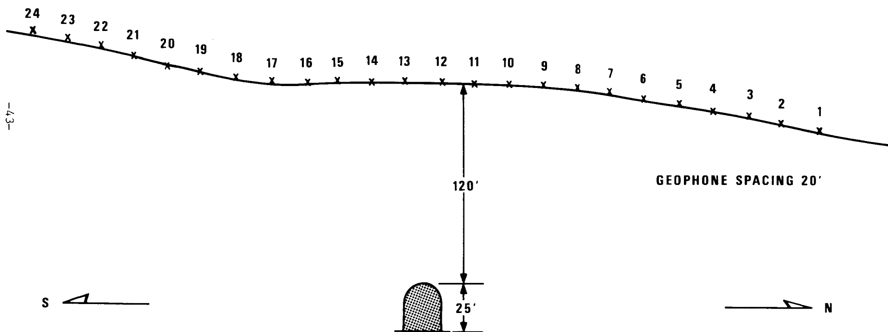
Figure 30. Seismic profile over Tunnel 19, DRGW Railroad.
