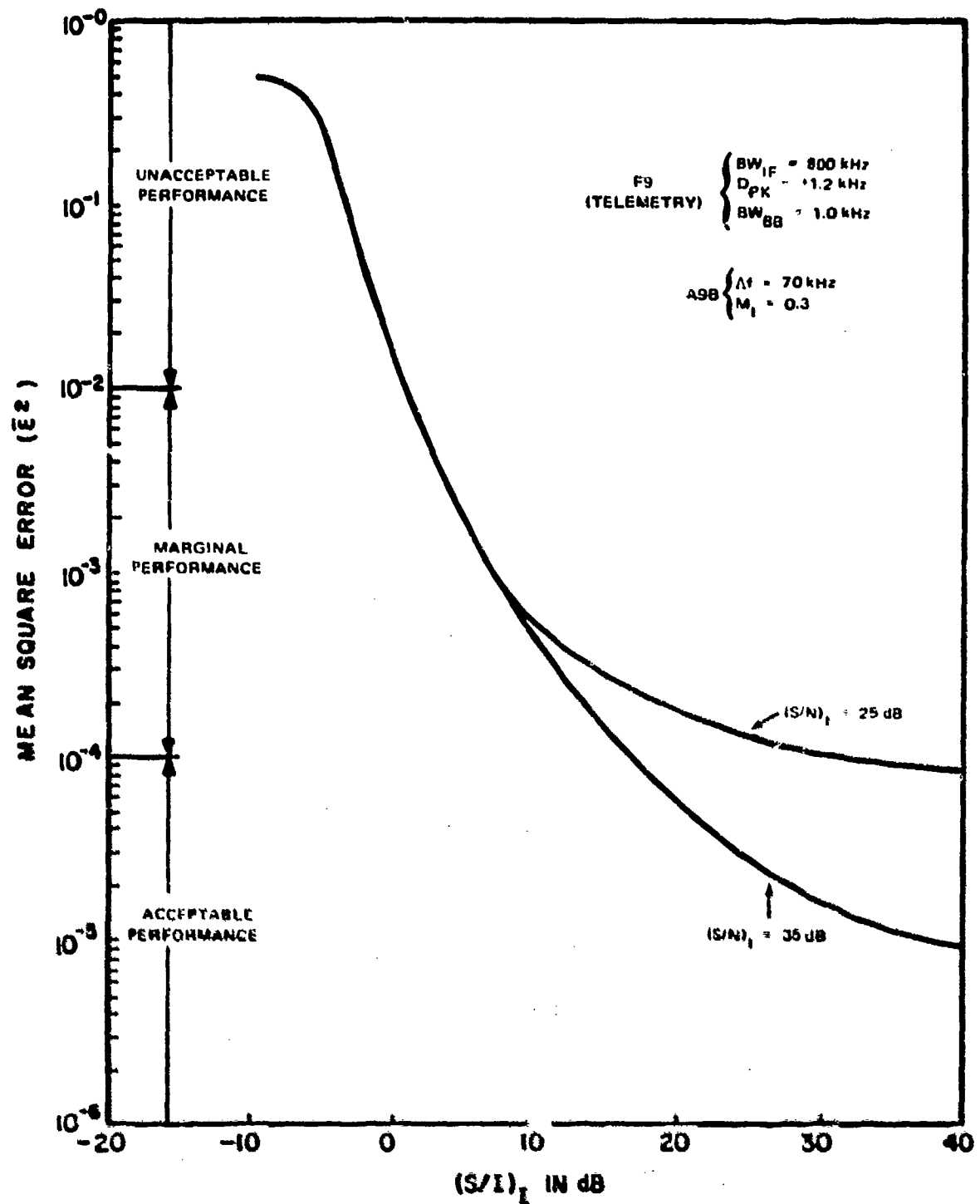
Figure C-140. Performance degradation curve for an F9 (telemetry) receiver with A9B ( \Delta f = 70 \text{ kHz} ) interference.
