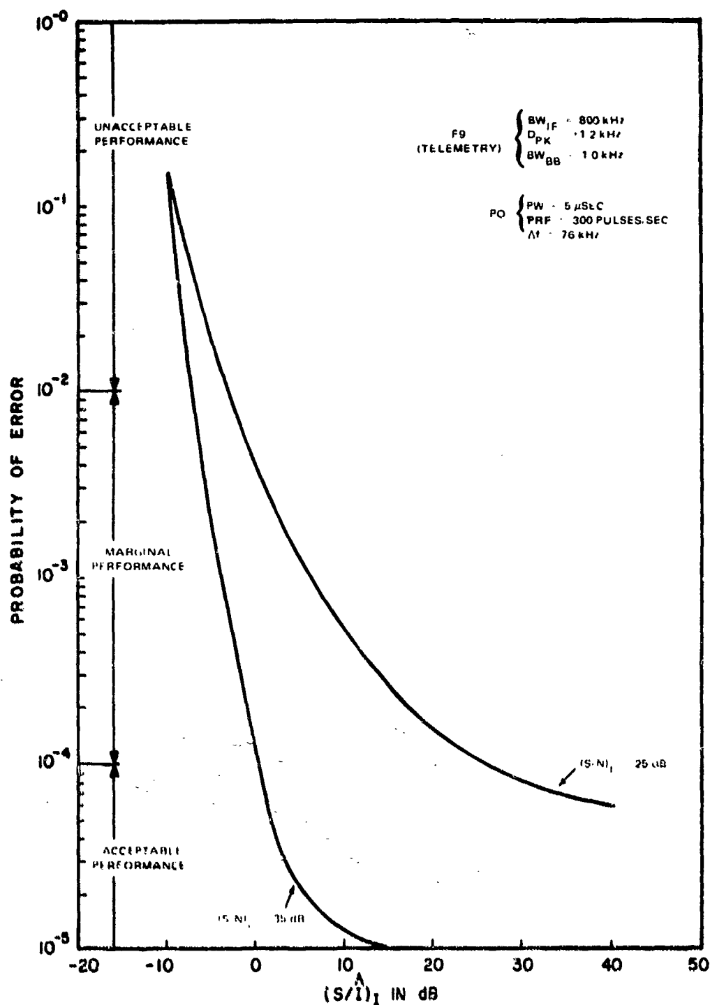
Figure C-148. Performance degradation curve for an F9 (telemetry) receiver with PO ( \Delta f = 76 \text{ kHz} ) interference.
