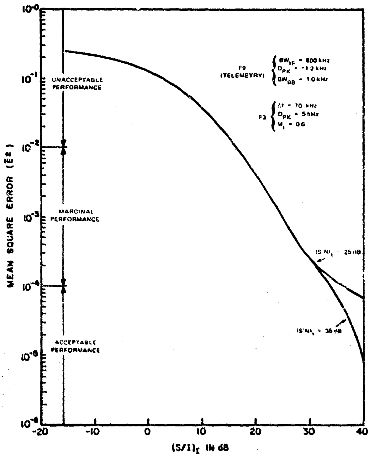
Figure C-144. Performance degradation curve for an F9 (telemetry) receiver with F3 ( \Delta f = 70 \text{ kHz} ) interference.
