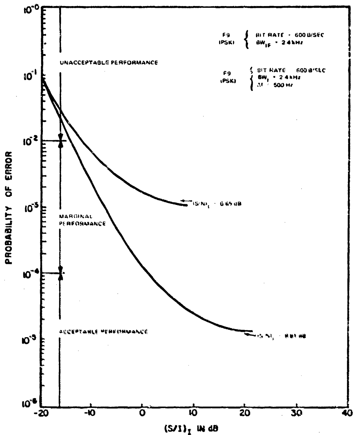
Figure C-130. Performance degradation curve for an F9 (PSK) receiver with F9 (PSK) interference ( \Delta f = 500 \text{ Hz} ).
