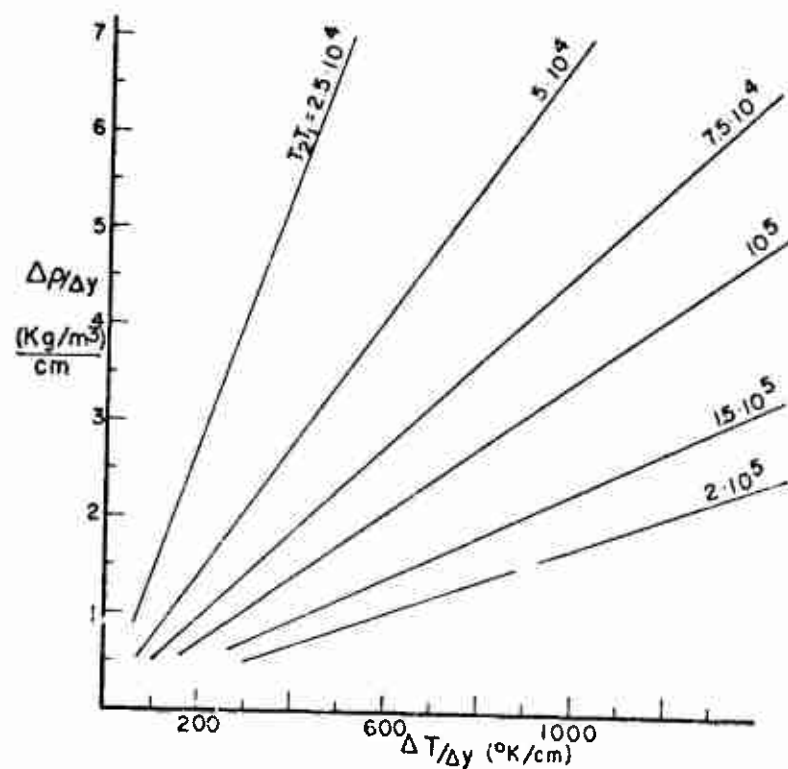
Fig.19 Density gradients for N_2 in terms of temperature extremes
