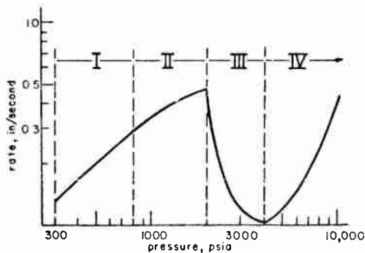
Fig 1. Deflagration rate of ammonium perchlorate in N_2 (after Boggs, ref. 3)
