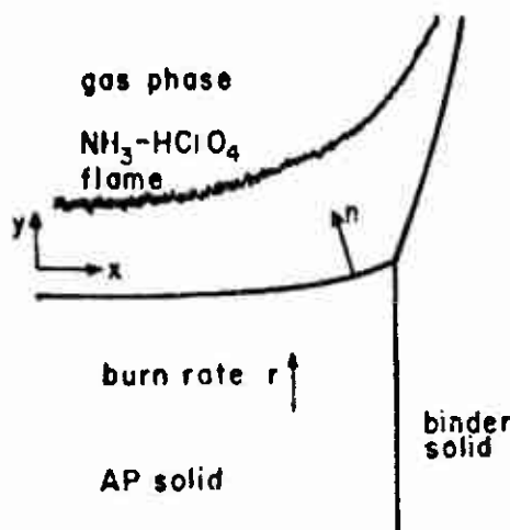
Fig.2 Sandwich schematic (after Strahle, et al., ref.5)
