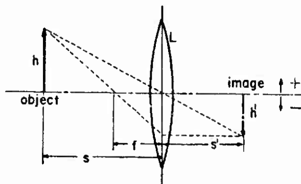
Fig.13a Thin lens model
