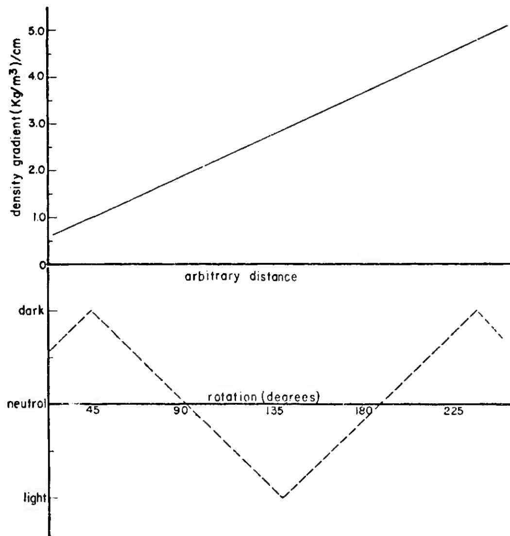
Fig.20 Cyclic intensity variation with monotonic density gradient
