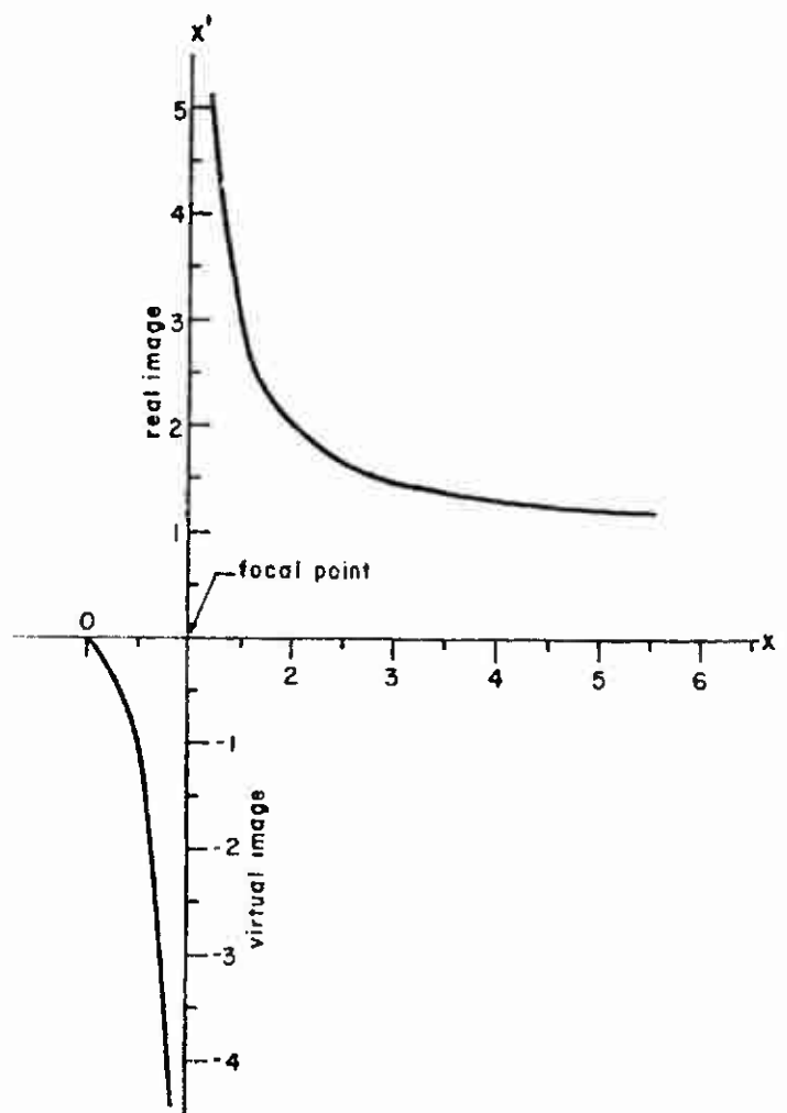
Fig.13b Non-dimensional thin lens model
