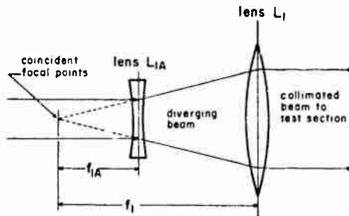
Fig.16 Divergence of laser beam
