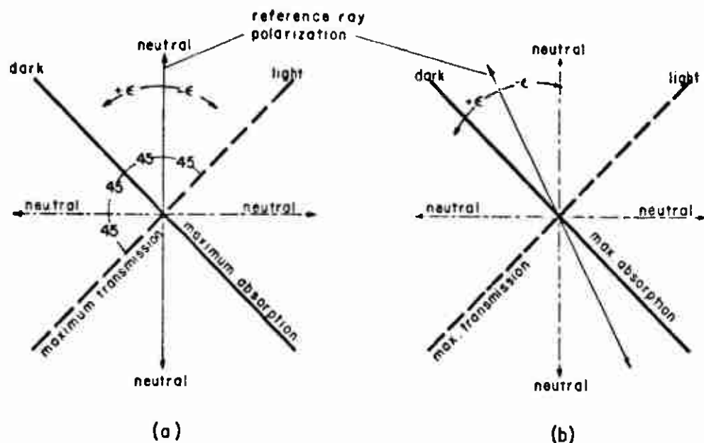
Fig.18 Polaroid sheet and reference ray polarization orientation
