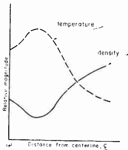
Fig 22c. Property profiles
