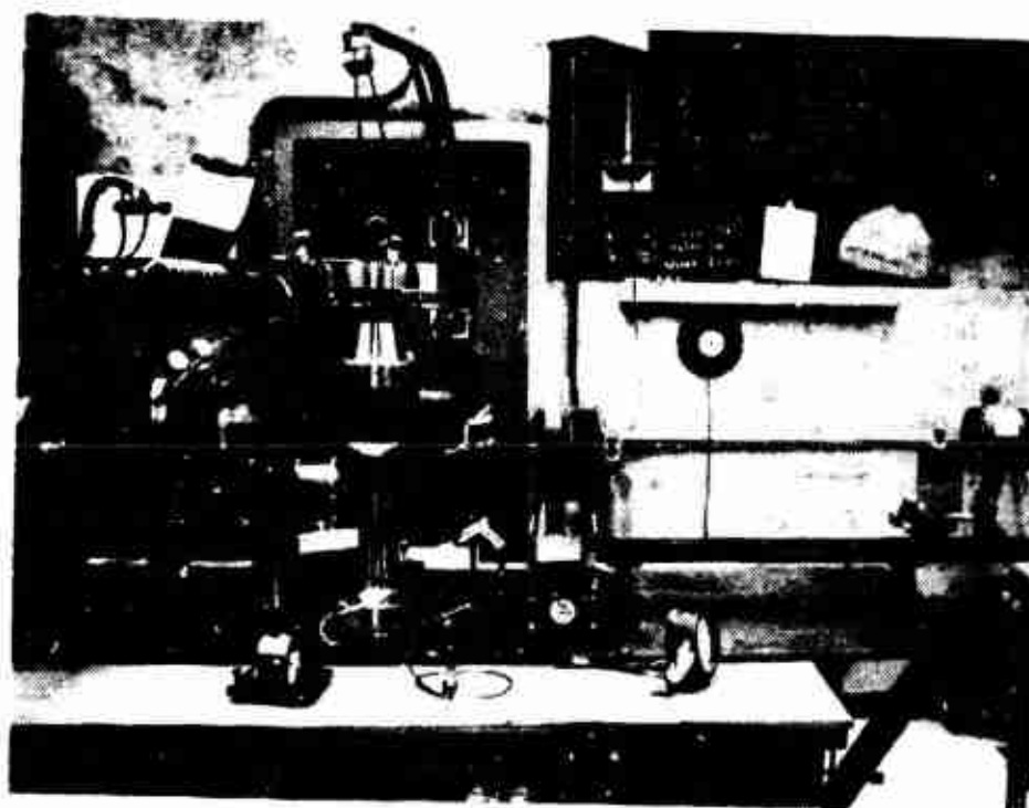
Fig.9b Side view of schlieren system from lens L_1 to lens L_3
