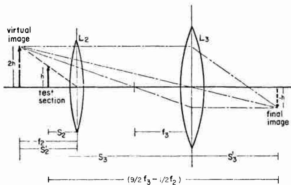
Fig.12 Virtual image setup ( S_2 = 0.5f_2 & S_3 = 3f_3 )
