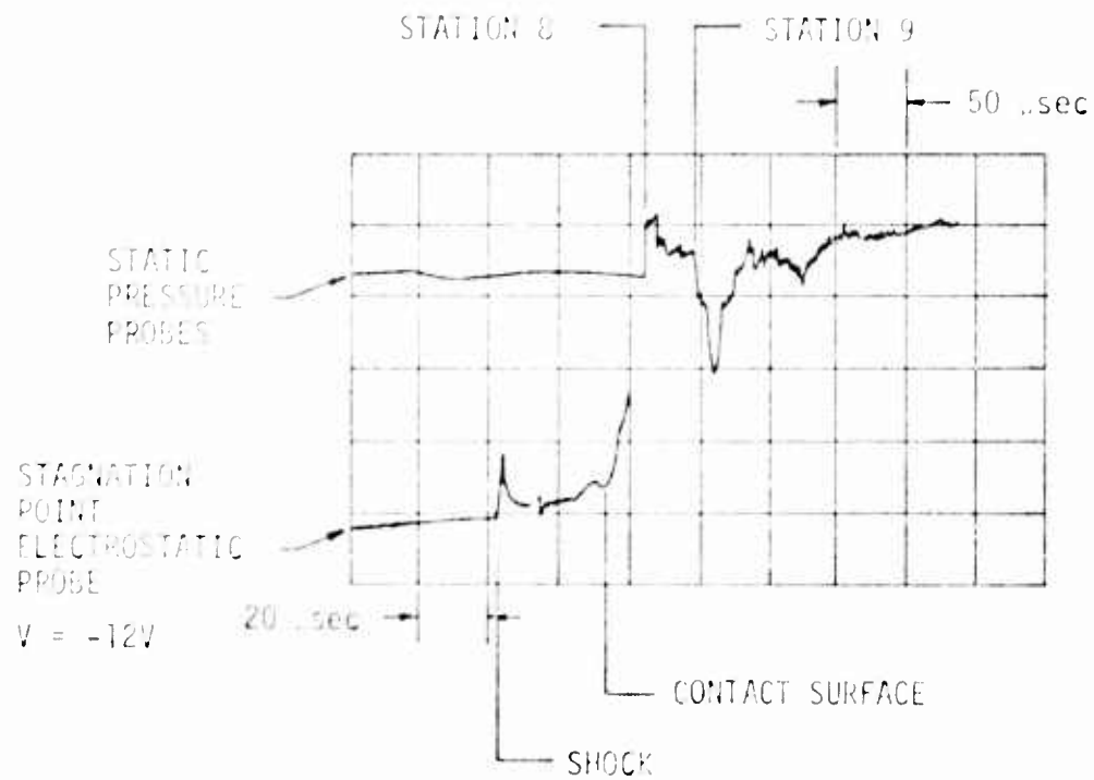
FIGURE 13B STAGNATION POINT ELECTROSTATIC PROBE RESPONSE
