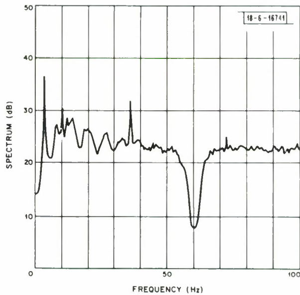
Fig. 28. ELF spectrum recorded in Saipan, 0600-0900 GMT, May 3, 1972 (tape 3005, channel 1, 3 dB/octave, soft limiter).
