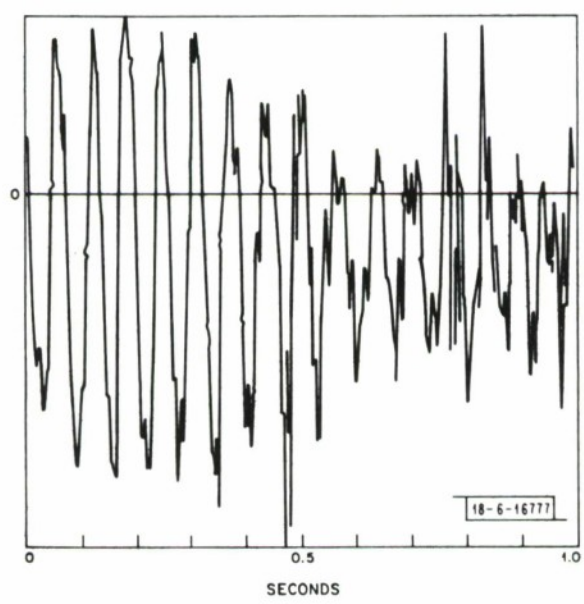
Fig. A-16. Typical waveform recorded in Norway, 2230 GMT, October 30, 1971 (tape 37).
