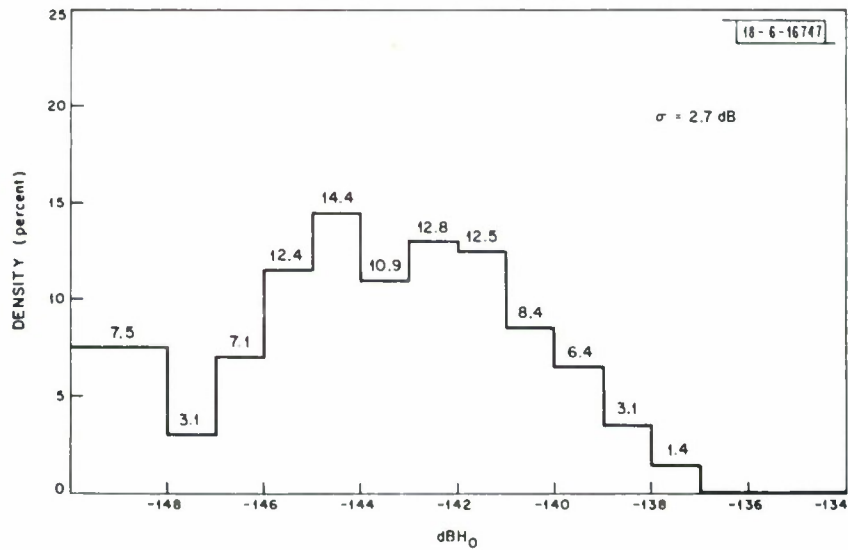
Fig. 34. Distribution of effective noise levels for Saipan data in the 72-76 Hz band (10 days in May 1972).
