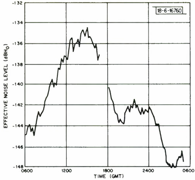
Fig. 47. Effective noise levels at 72 Hz recorded in Greece, May 7-8, 1972 (tapes 2013-2014).
