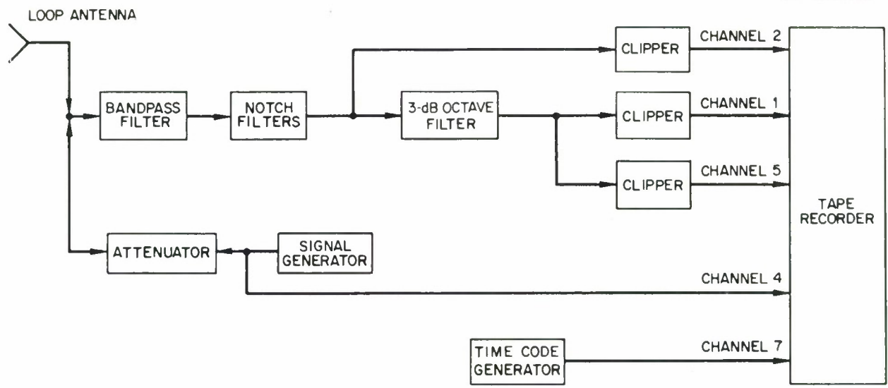
Fig. 1. Simplified block diagram of recording equipment.
