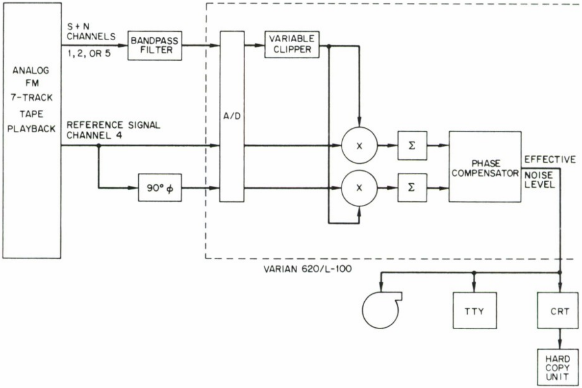
Fig. 2. Simplified block diagram of noise processor.
