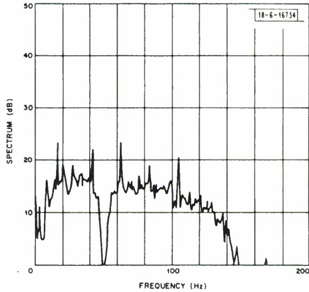
Fig. 21. ELF spectrum recorded in Norway, 1900-1920 GMT, January 4, 1972.
