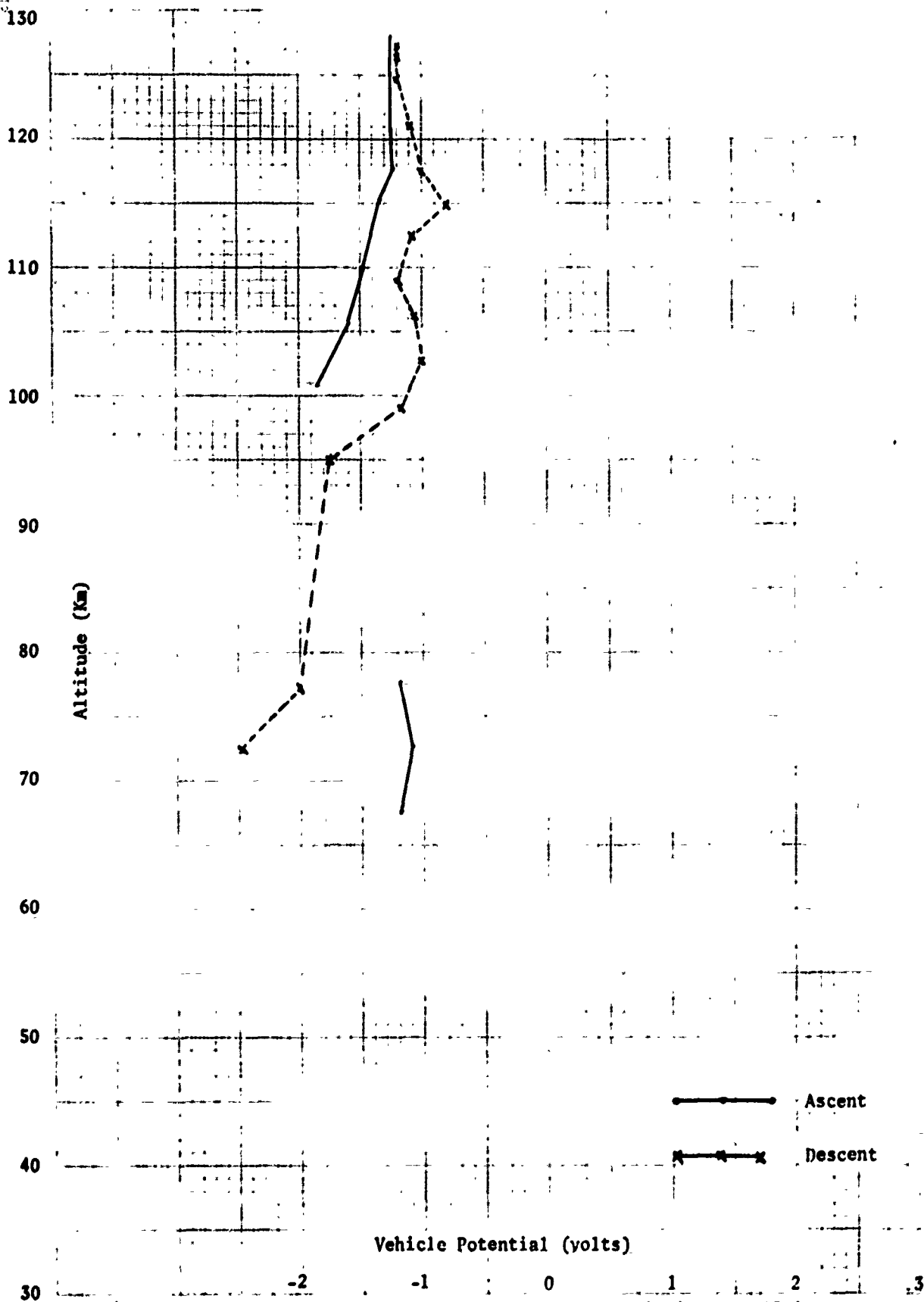
Figure 83 Vehicle Potential Measurement for Ute-Tomahawk AO 9.303-4
