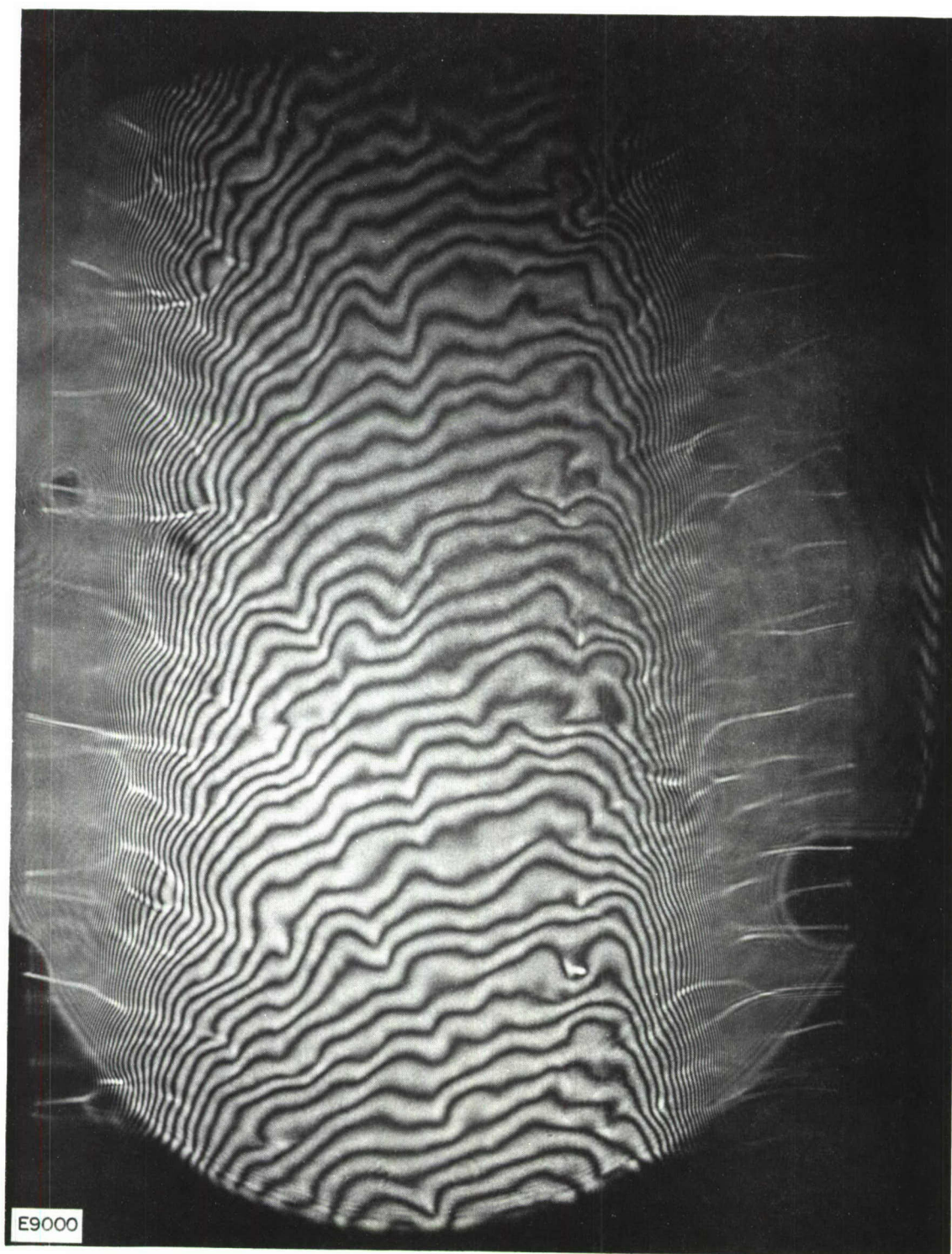
Fig. 6 Interferogram of the Medium Homogeneity looking along the Lasing Axis, taken at -175^{\circ}\text{C} , a Flow Velocity of 400\text{ cm/sec} and a Pressure of 1/6\text{ atm}
