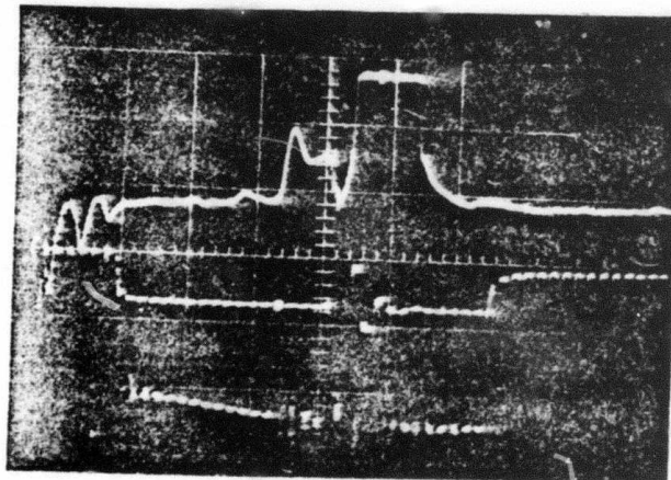
Figure 1. HCl Laser Emission Observed in the Plasma Diode Electron Gun Facility. Ar/H 2 /Cl 2 (49.5/49.5/1). P total = 200 torr.
