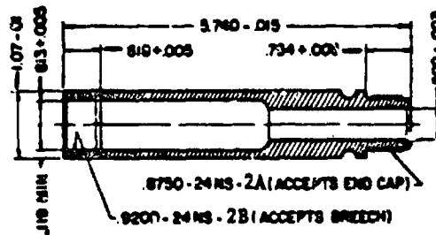
Figure 6-11. Thruster Body
