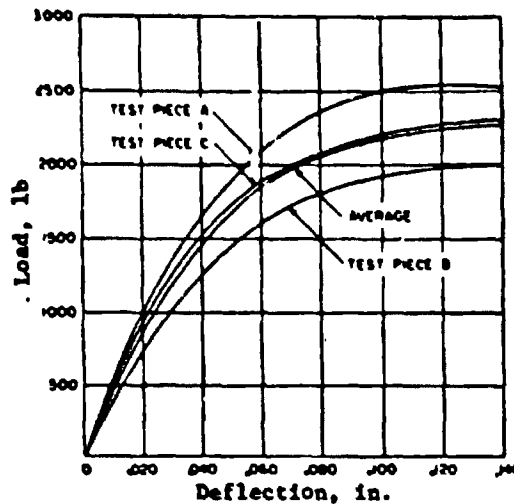
Figure 6-17. Load Deflection Curves for Keylock Mechanisms
