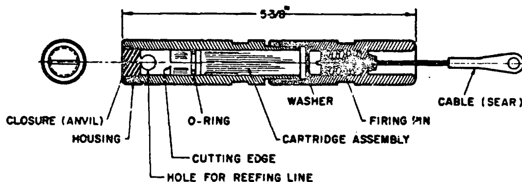
Figure 2-7. Typical Reefing Line Cutter
