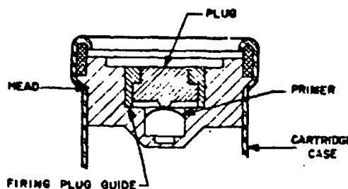
Figure 4-12. Firing Plug
