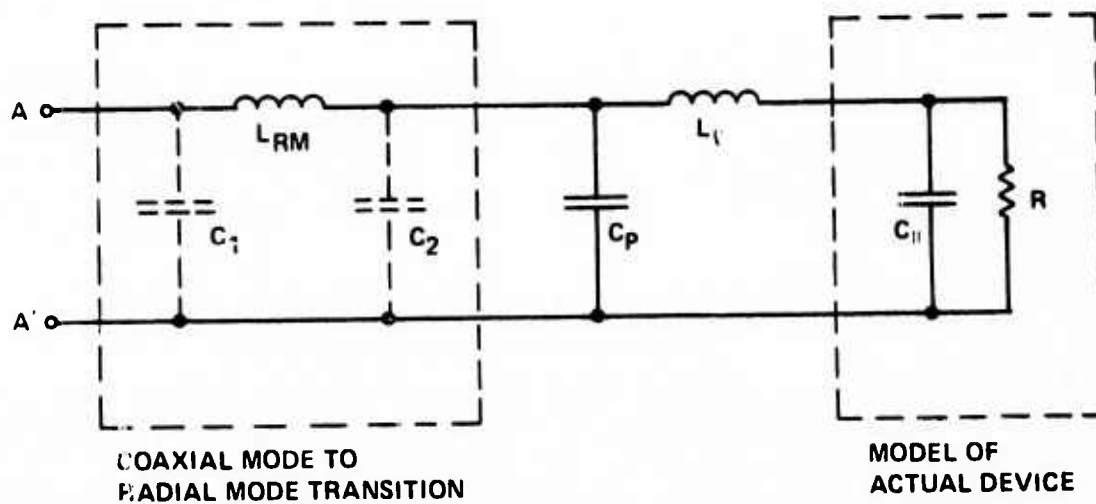
FIG. 20 Equivalent microwave circuit of package diode mounted in termination of coaxial transmission line.
