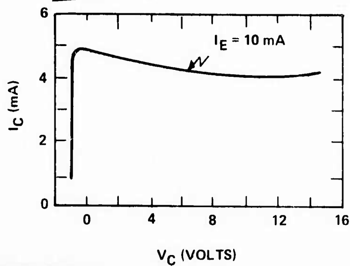
FIG. 33 Grounded-base characteristics of device shown at bottom of Fig. 31. Only single trace is shown (for I_E = 10 mA) because instabilities due to negative resistance occurred when curve tracer was set to automatic step emitter current.
