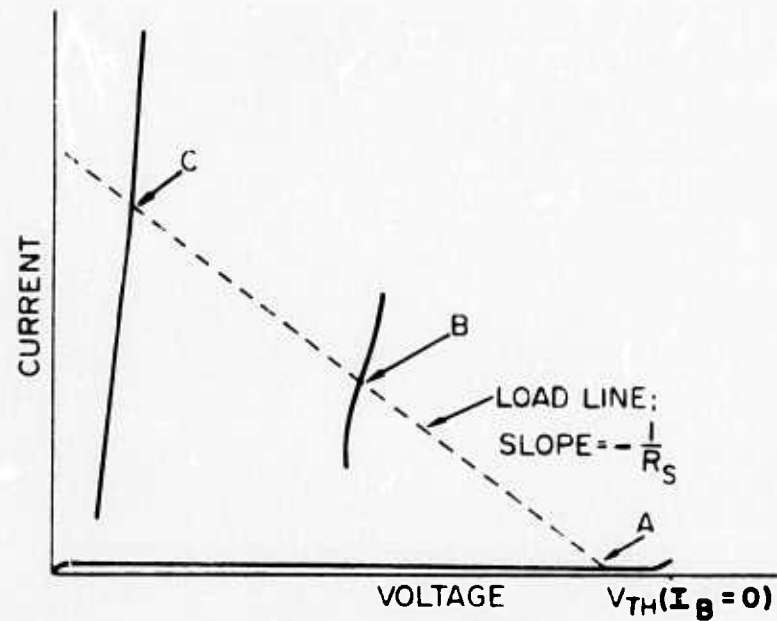
FIG. 1 Current voltage characteristics for a CID. If base current drive is supplied threshold voltage V_{th} is reduced. Load line is determined by series resistance of collector power supply. Switching from A \rightarrow B , B \rightarrow C or A \rightarrow C is possible with base current drive.
