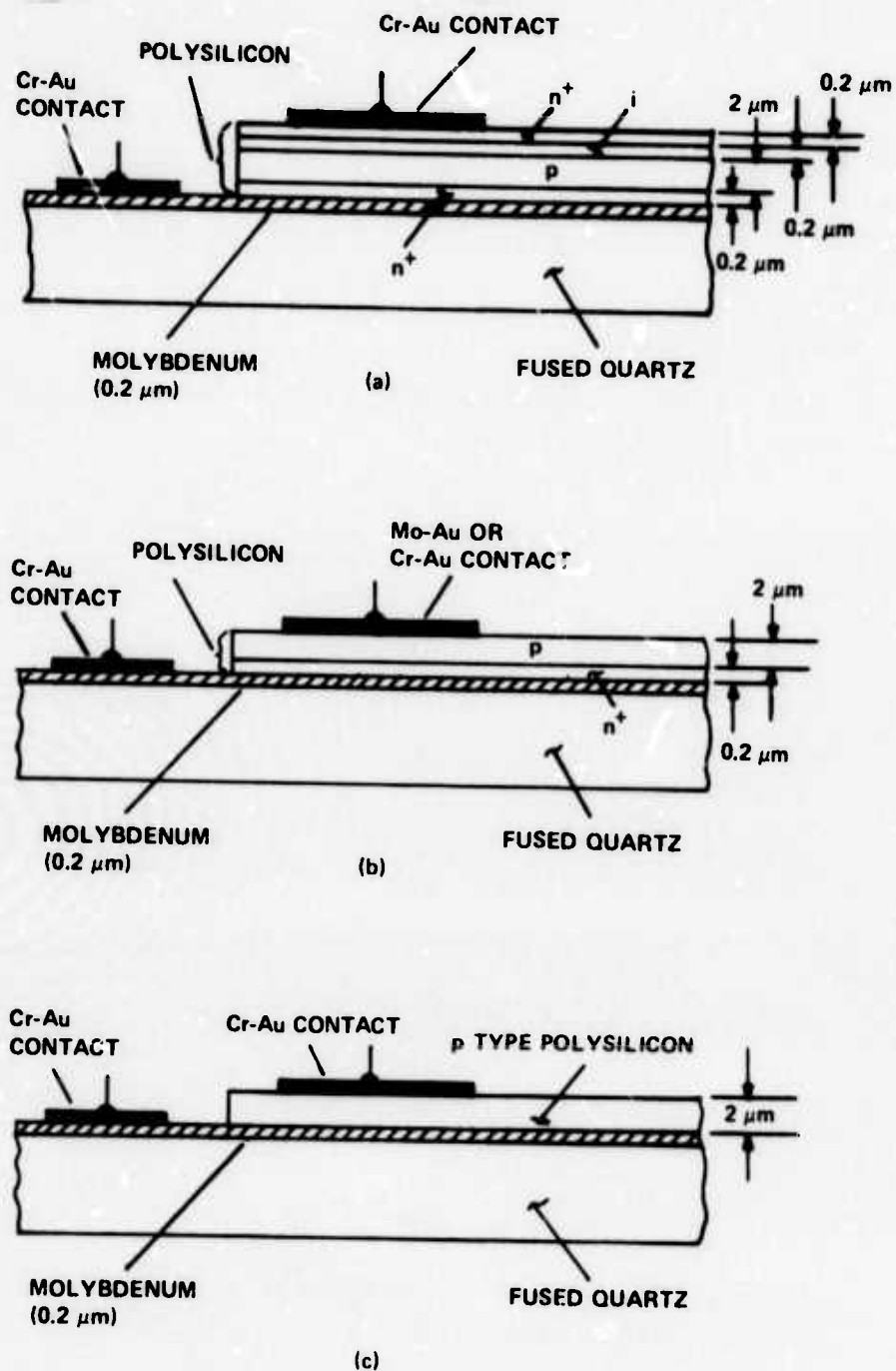
FIG. 54 Cross-sectional diagrams of three device structures fabricated using no single crystal silicon:
