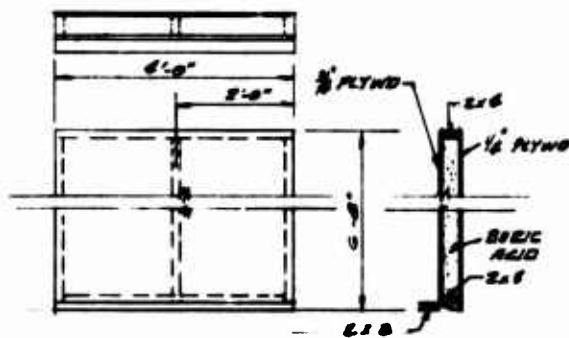
WALL SHIELD 9 REQ'D EST WT. 400 LBS
