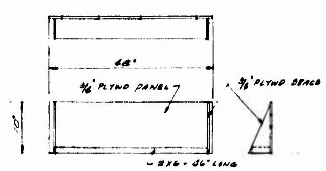
PIPE SUPPORT BRACKET WOOD - ONE REQ'D (NOT TO SCALE)
