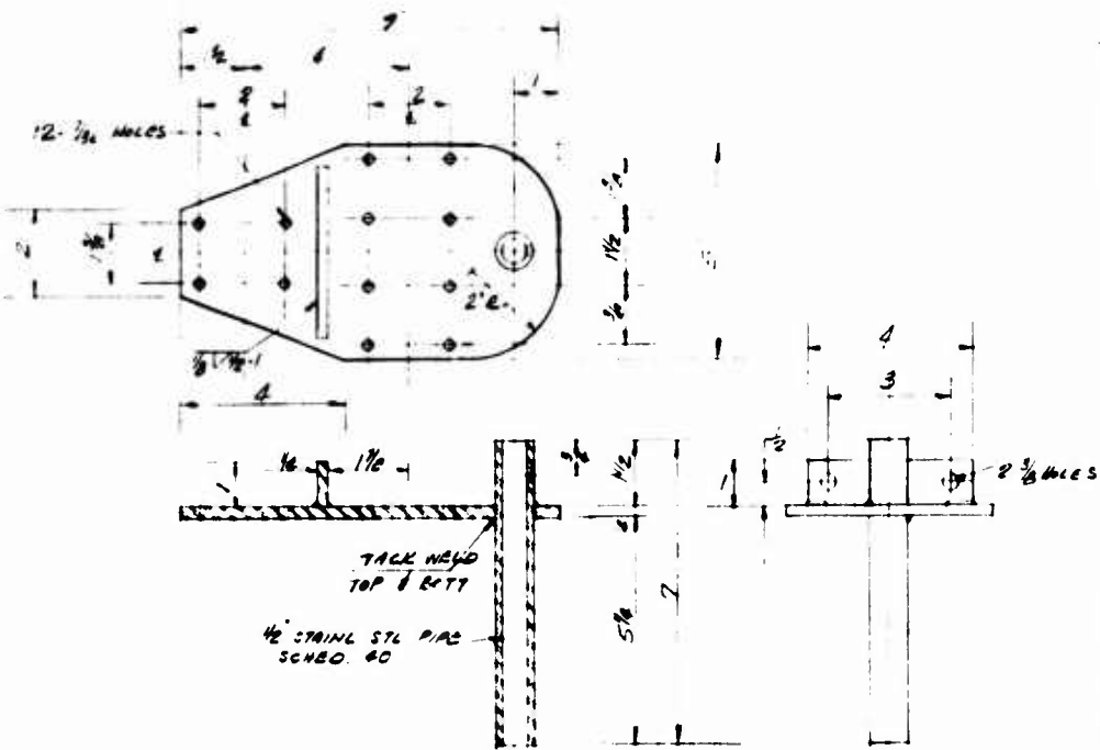
SOURCE GUIDE & CARRIER PLATE 316 STAINL STL PL ONE REQ.
