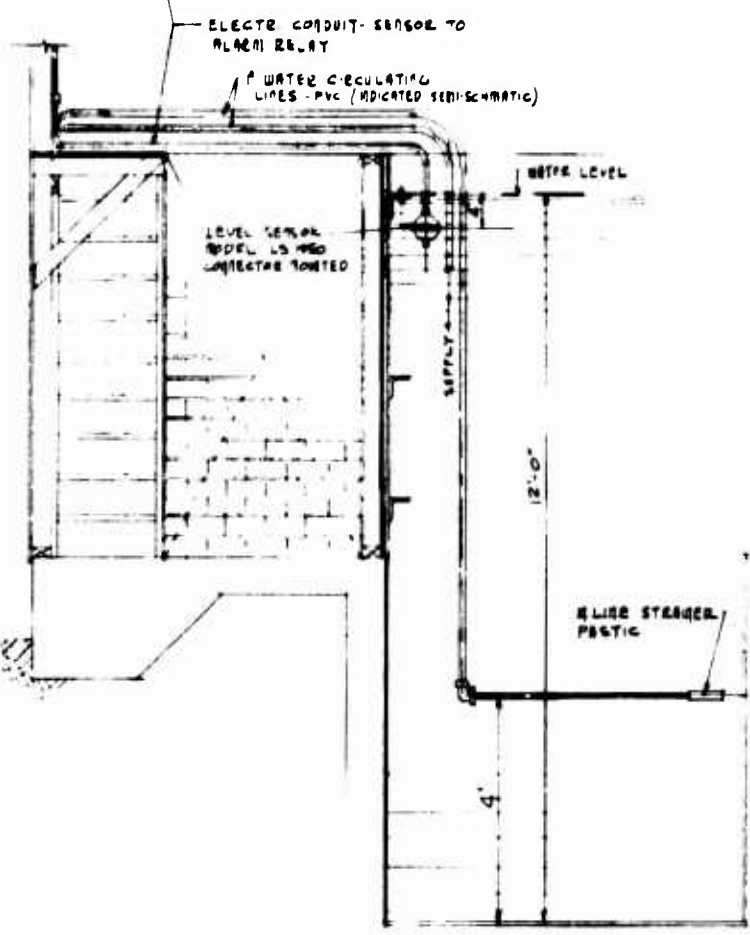
SECTION 1
