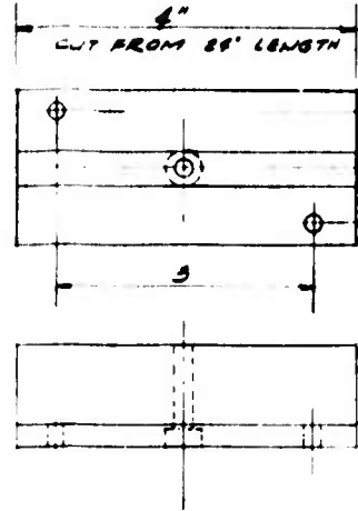
BAIL SUPPORT THOMSON # SR 12 - ALUM. 12 REQ'D
