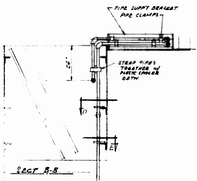
PIPE SUPPORT PLATES 1/2" THK PLEXIGLAS ONE EACH REQ'D
