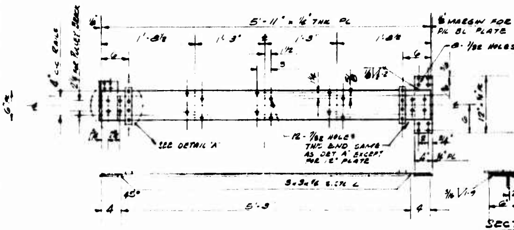
SOURCE CARRIER BEAM 316 STAINLESS STL PLS 308 STAINL STL ANGLE ONE REQ.
