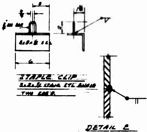
DETAIL E
