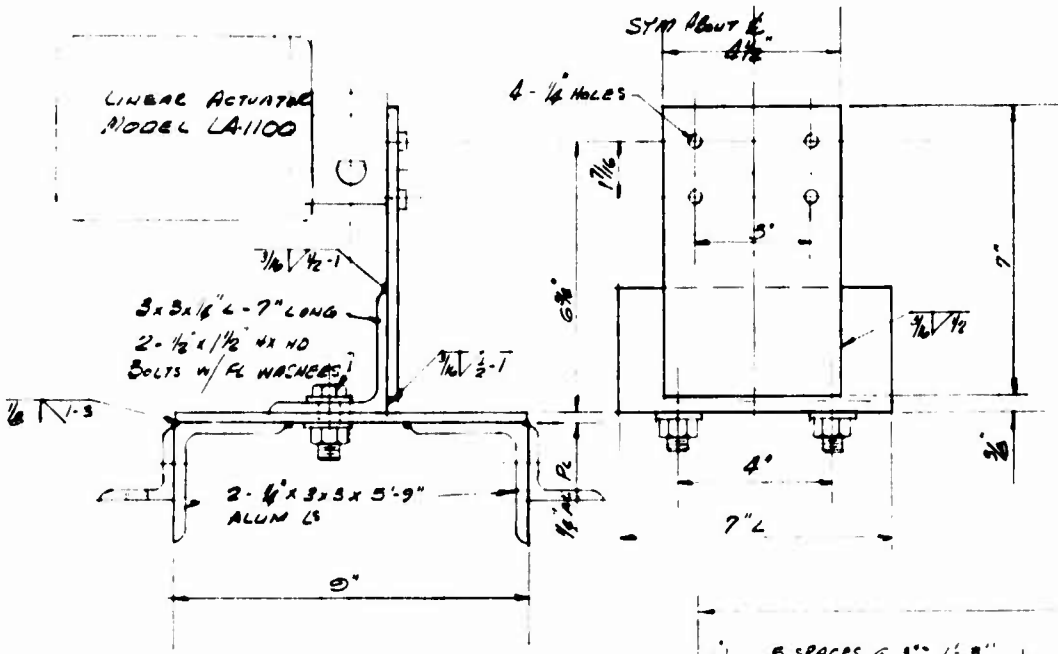
END VIEW A-A LINEAR ACTUATOR MOUNTING DETAIL
