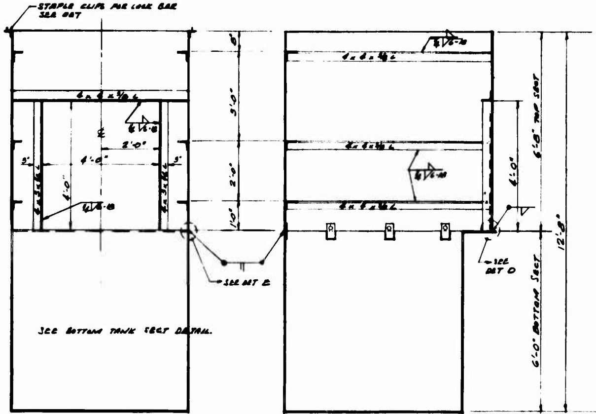
SECTION B
