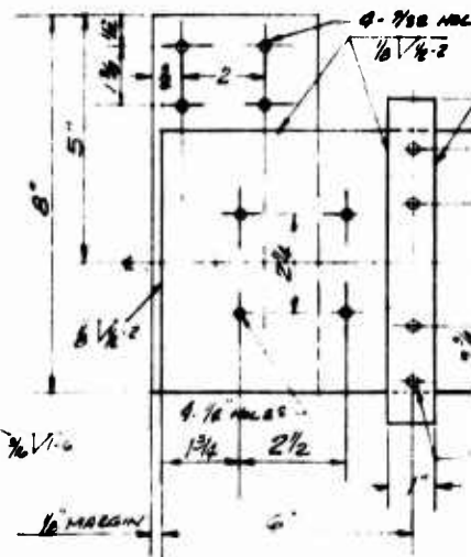
DETAIL
