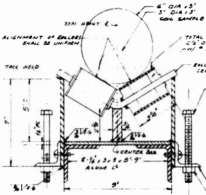
SECT B-B TYPICAL SECT.
