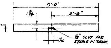
LOCK BAR 3x2x1/4 AL. ANGLE - 2 REQ'D WT = 9 LBS. EA
