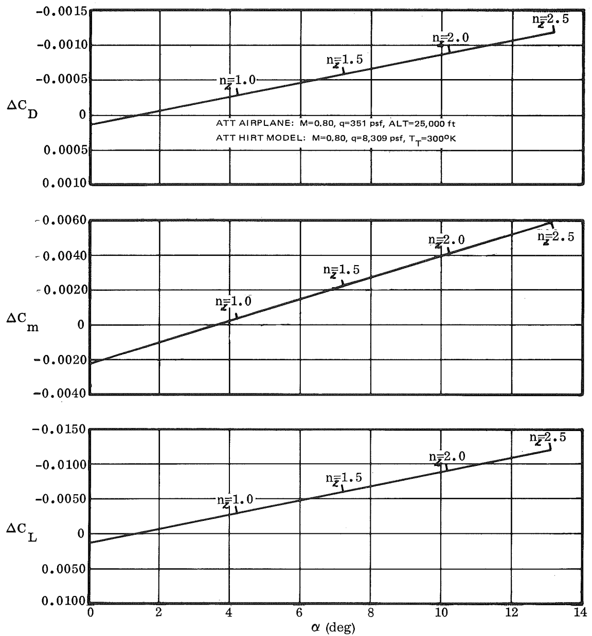
Figure 70 . Estimated Effect of Angle of Attack on the Incremental Aerodynamic Data for the ATT Study Configuration at Mach 0.8
