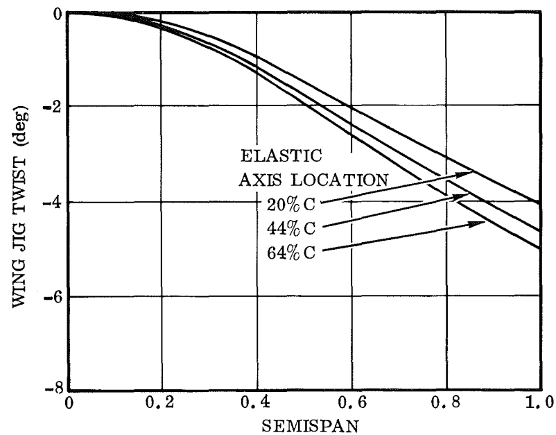
Figure A-3. Wing Jig Twist Distribution for the F-111 Composite Wings
