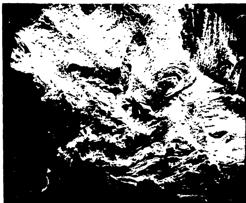
Fig. 5-4 Origin of Fatigue Fracture of Stiffened Panel at Gas Pore at Edge of Fusion of GMAW Weld. Test in Air.
