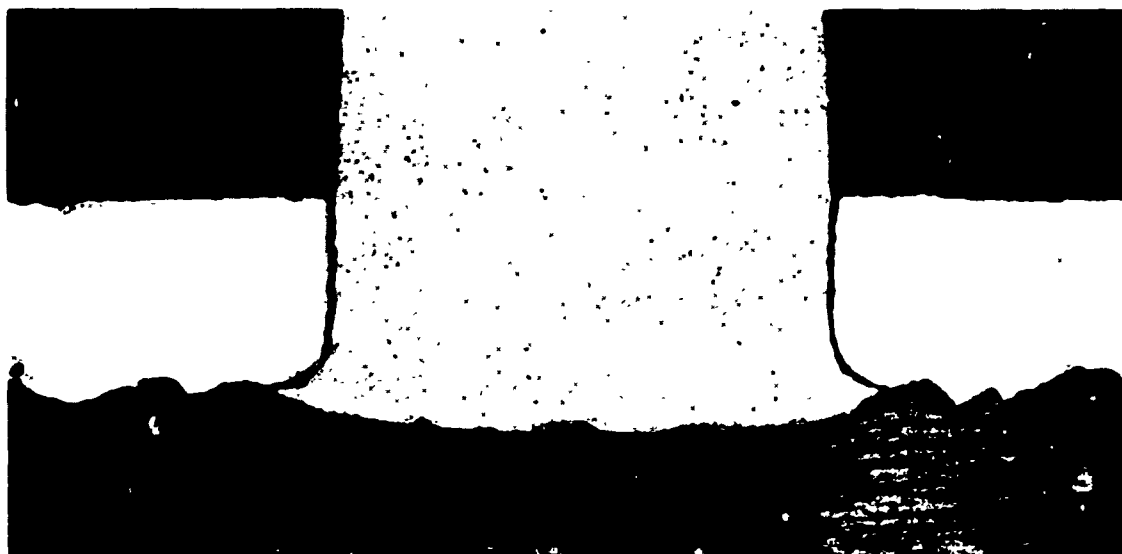
EXPLOSION WELD SPEC. NO. 420952-4 NEG. NO. 197603A MAG. 20X ETCH: ELECTROPOLISHED NOT POLARIZED SOUND WELD, SMALL UNFUSED ZONE .006" LAND - USI = .5 IN. - % PENETRATION = 95% EST. % PENETRATION = 75-90%
