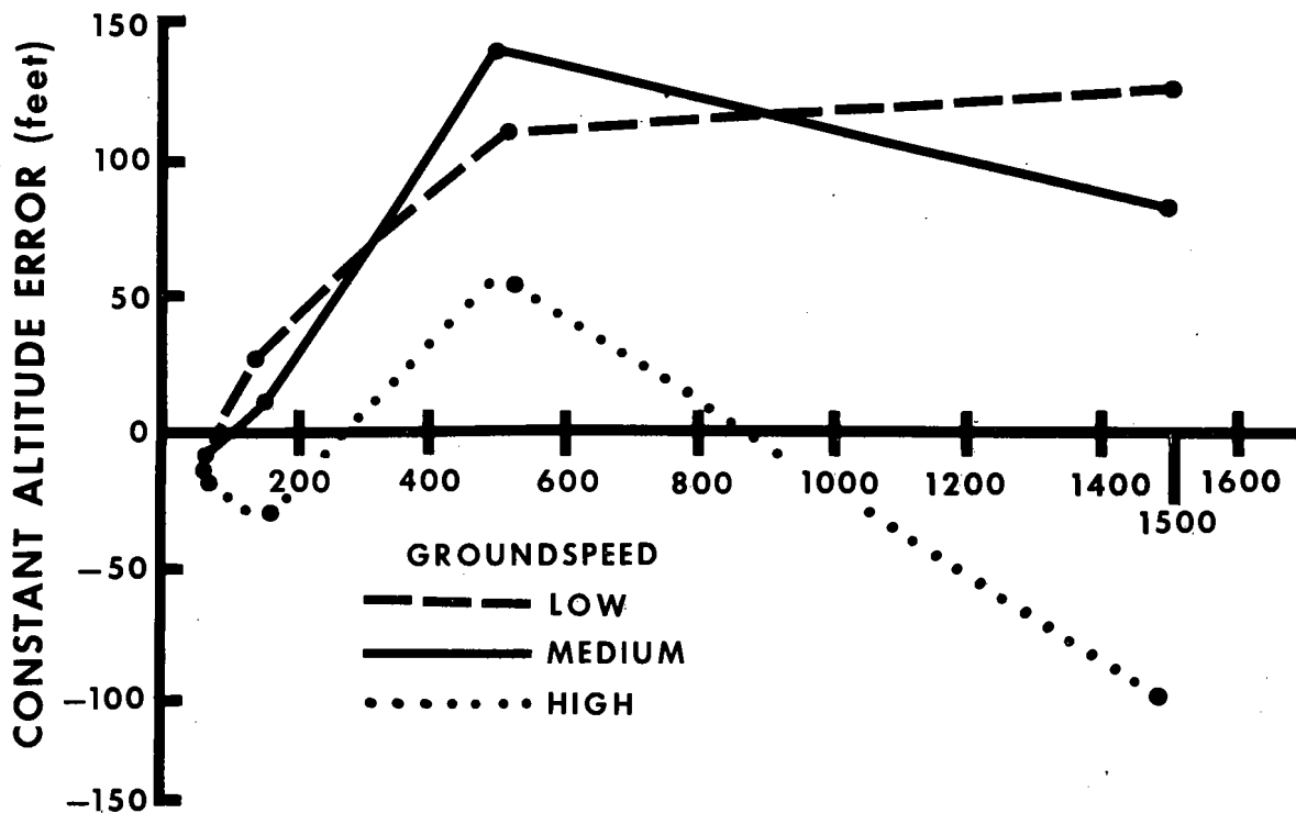
ALTITUDE-GROUND SPEED INTERACTIONS FIGURE 4
