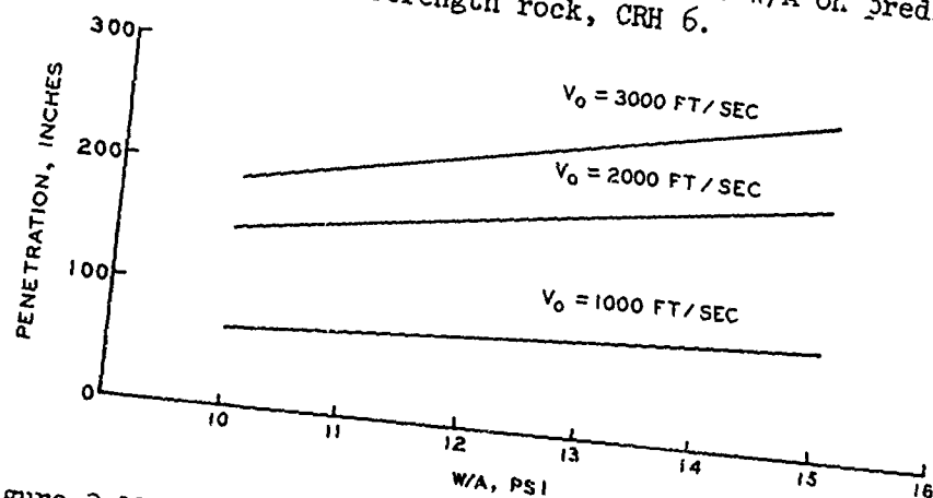
Figure 3.11 Effect of weight-to-area ratio W/A on predicted penetration into medium-strength rock, CRH 6.
