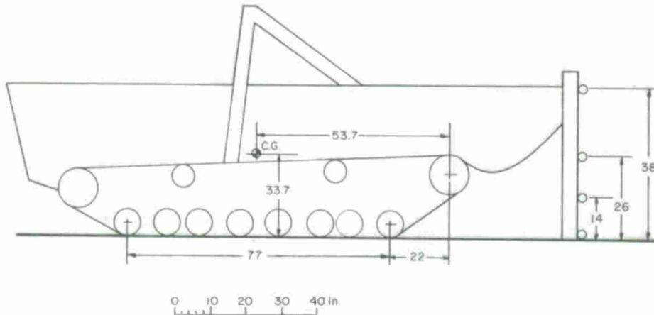
Figure 11. Vehicle dimensions.
